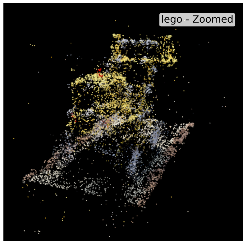
COLMAP | | num_points=10313
