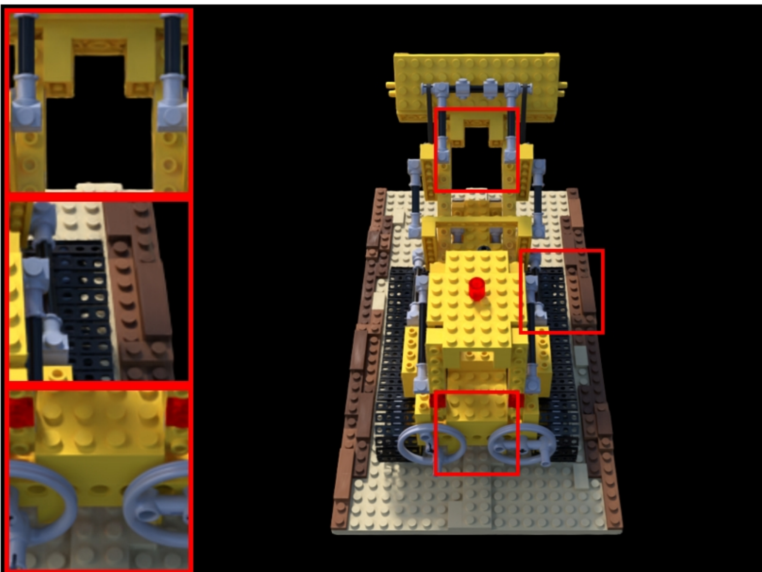
lego: COLMAP | | num_points=10313 PSNR: 22.79 | LPIPS: 0.0657 | SSIM: 0.8508
