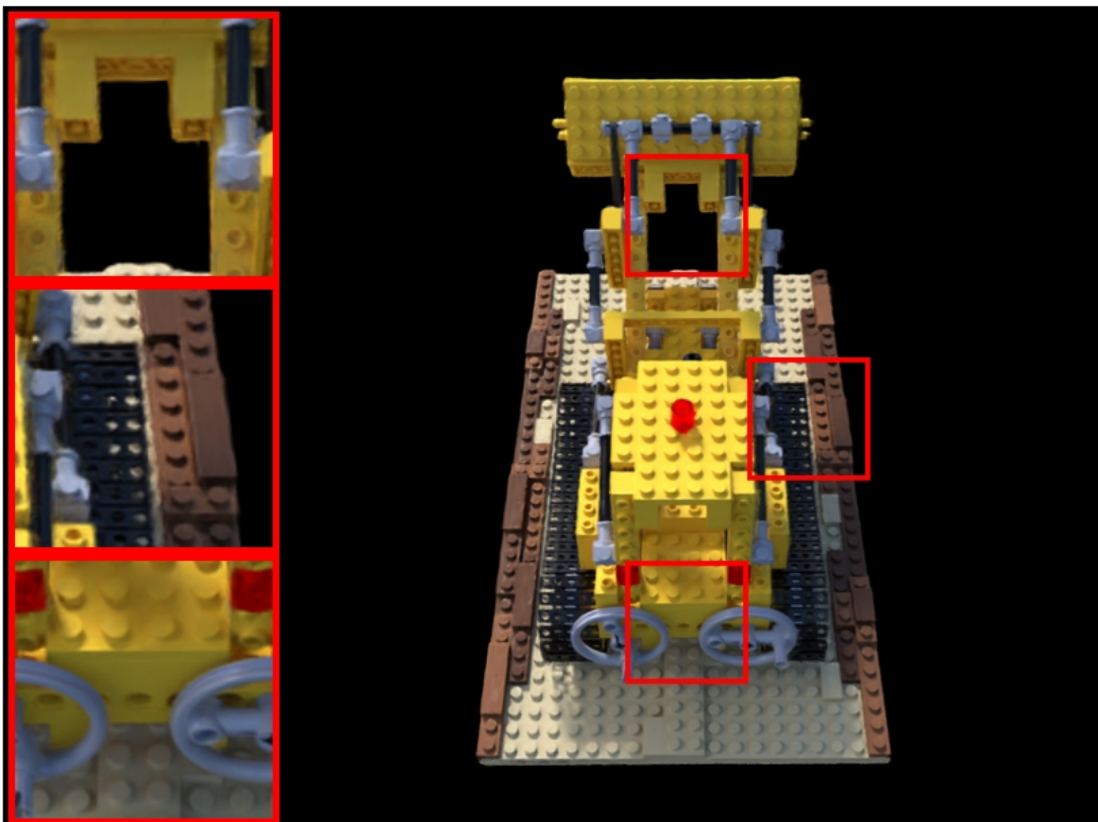
lego: VGGT | voxels | num_points=87000 PSNR: 20.56 | LPIPS: 0.0959 | SSIM: 0.7731
