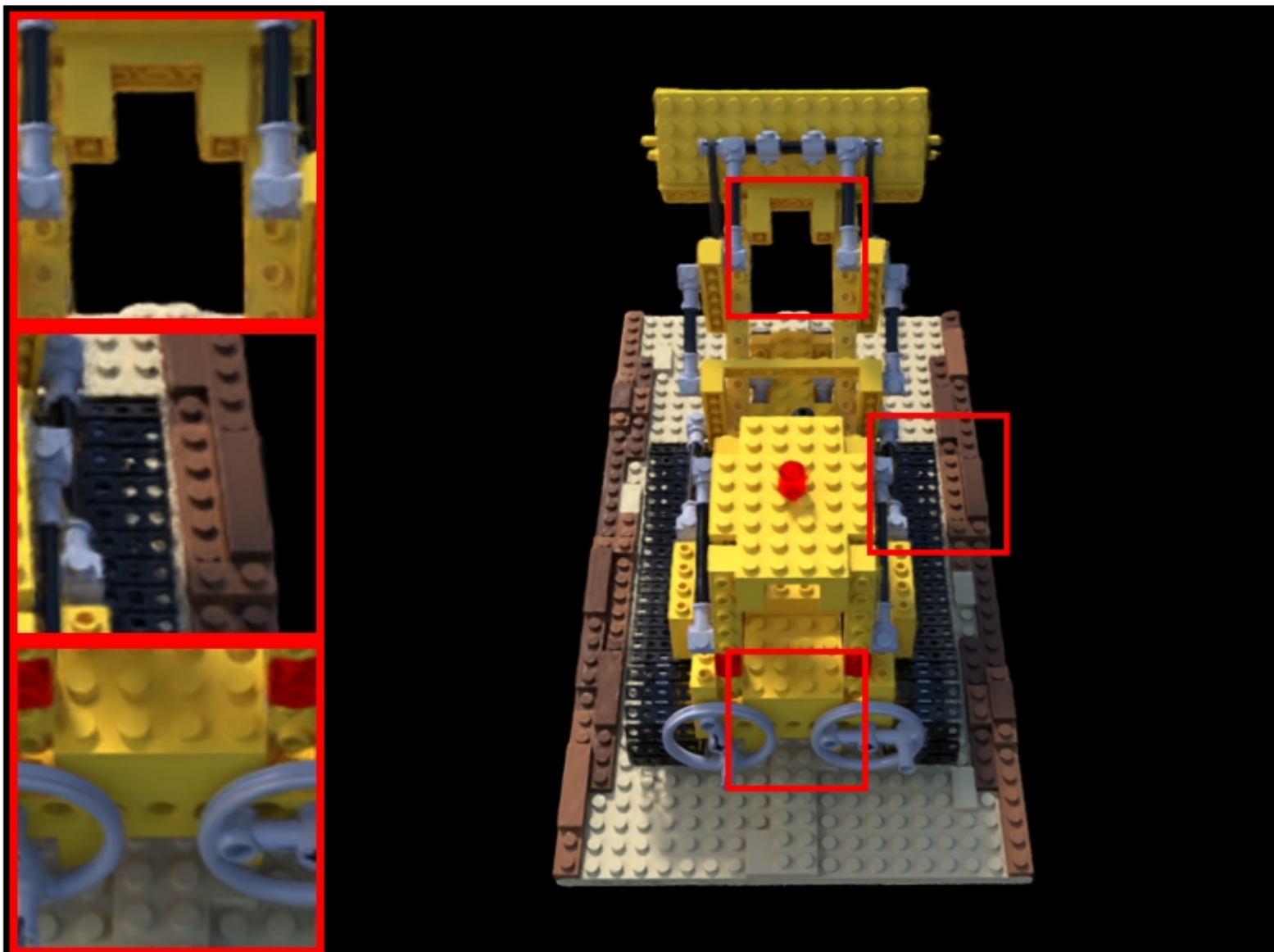
lego: VGGT | confidence | num_points=87000 PSNR: 20.61 | LPIPS: 0.0946 | SSIM: 0.7749
