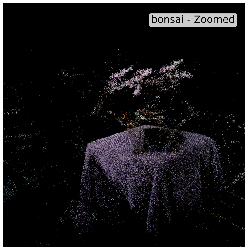
COLMAP | | num_points=80892
