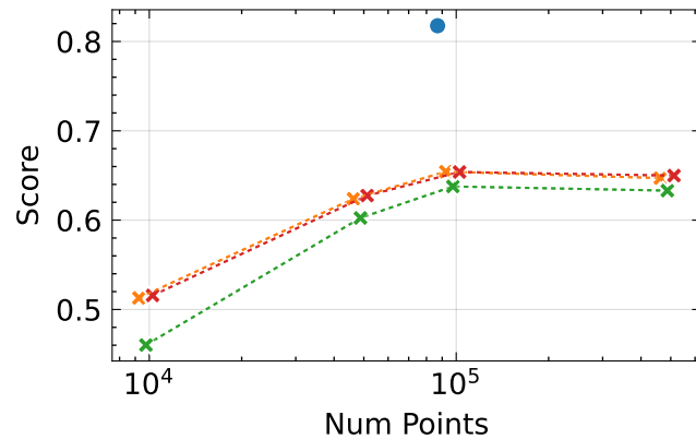
Composite Quality \uparrow - bonsai
