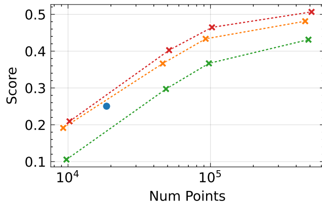
Composite Quality \uparrow - bicycle
