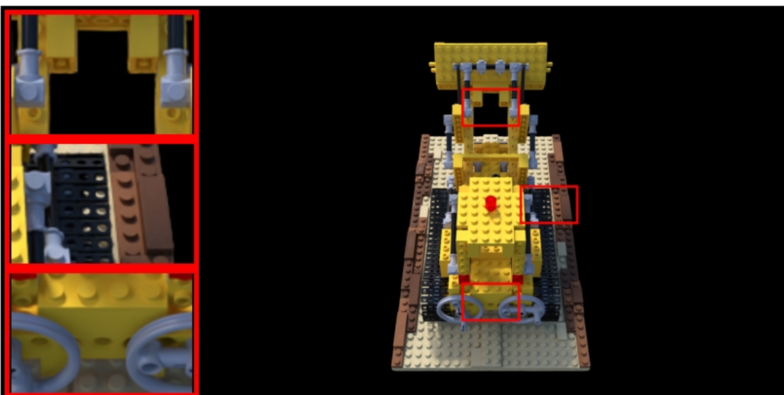
lego: VGGT | imagefreqvoxels | | num_points=87000 PSNR: 33.03 | LPIPS: 0.0337 | SSIM: 0.9797
