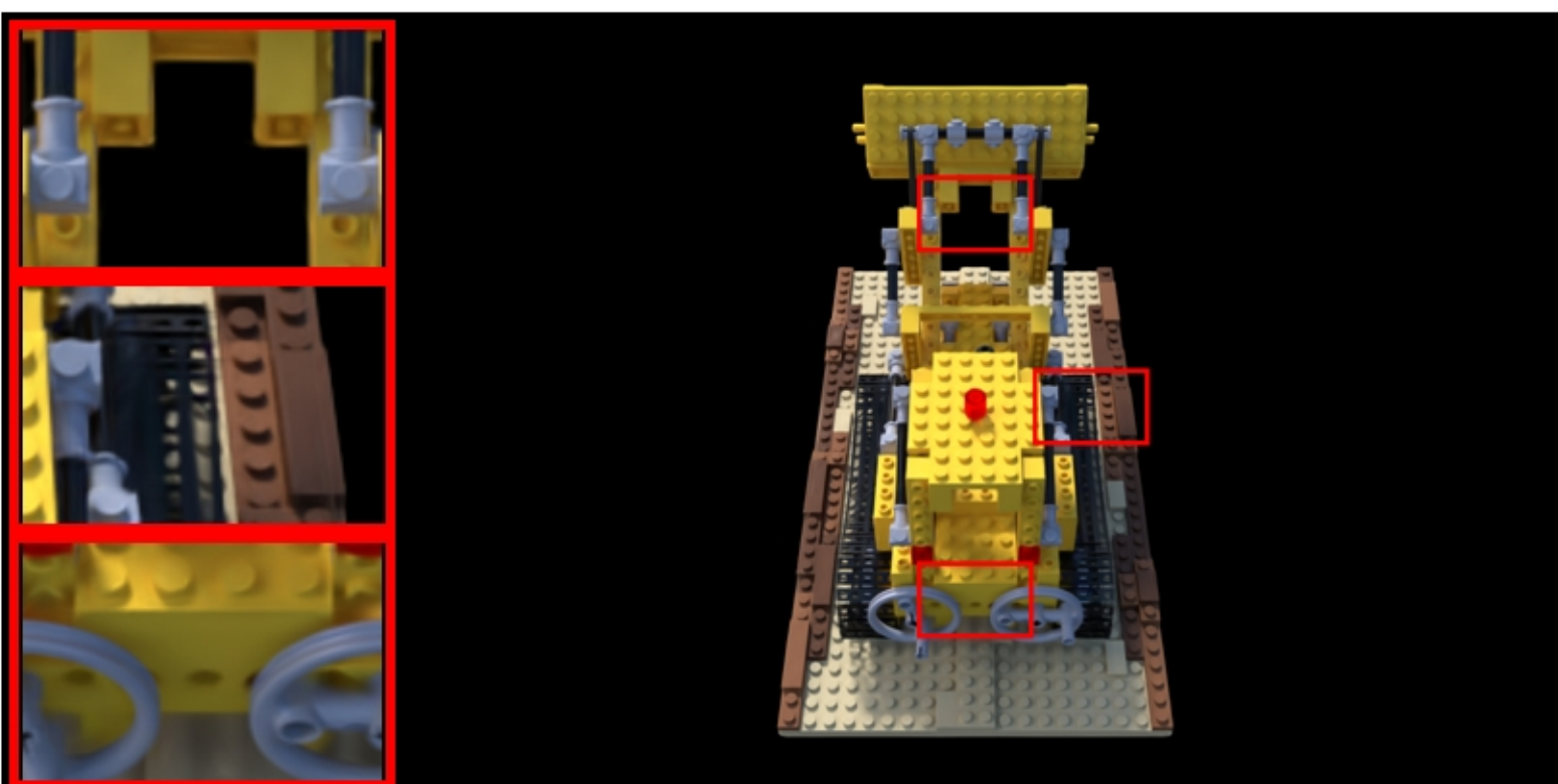
lego: COLMAP | | num_points=10069 PSNR: 31.35 | LPIPS: 0.0600 | SSIM: 0.9637
