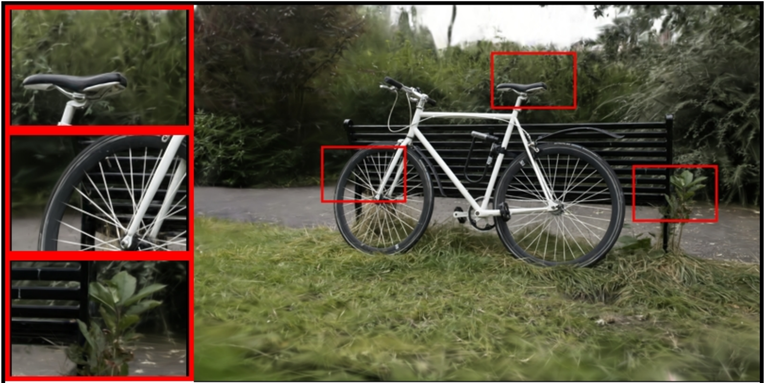
bicycle: VGGT | imagefreqnovis | | num_points=100000 PSNR: 22.41 | LPIPS: 0.3714 | SSIM: 0.5836
