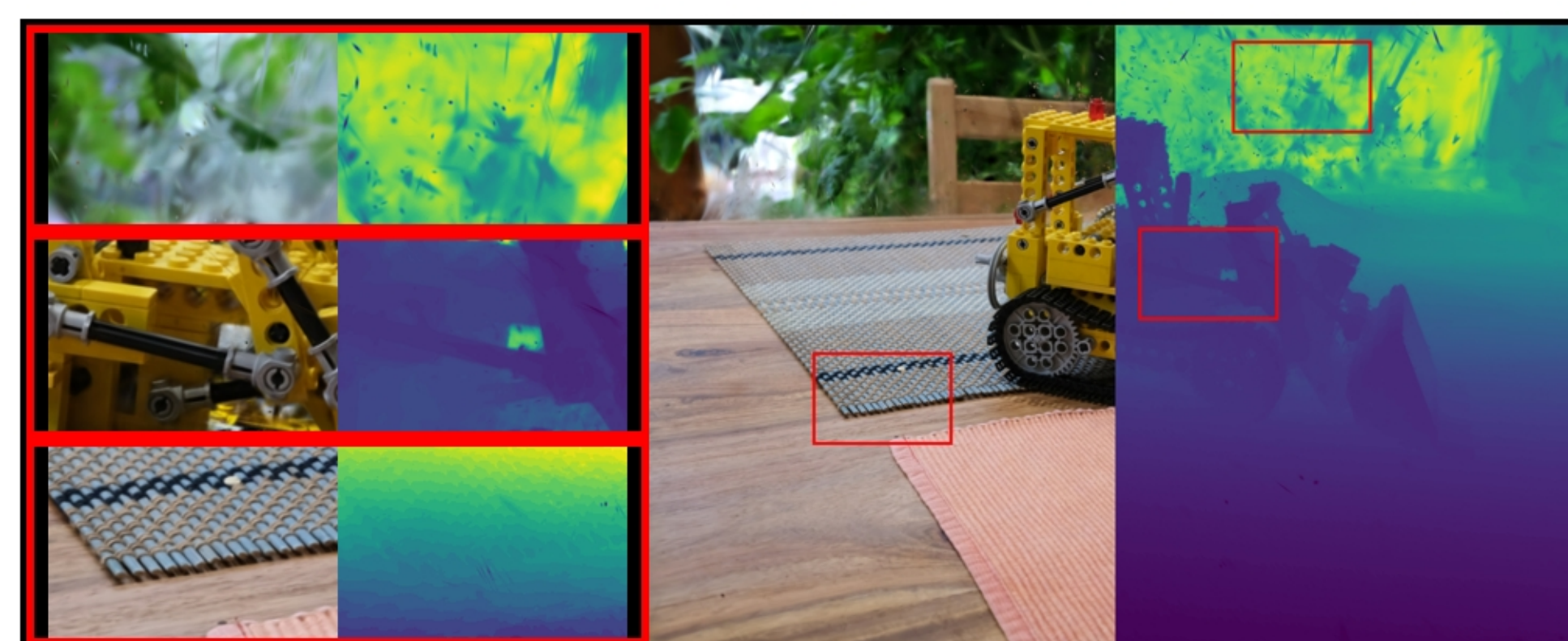
kitchen: VGGT | points PSNR: 19.31 | LPIPS: 0.2160 | SSIM: 0.4216
