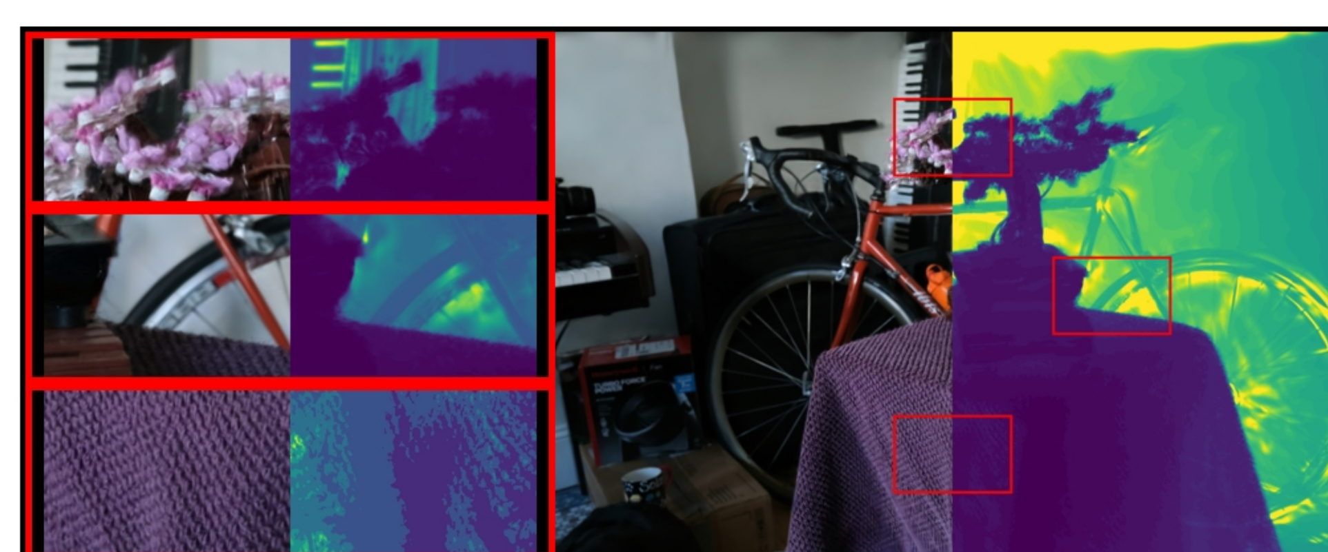
bonsai: VGGT | closer | Pose Opt PSNR: 17.64 | LPIPS: 0.3894 | SSIM: 0.5626
