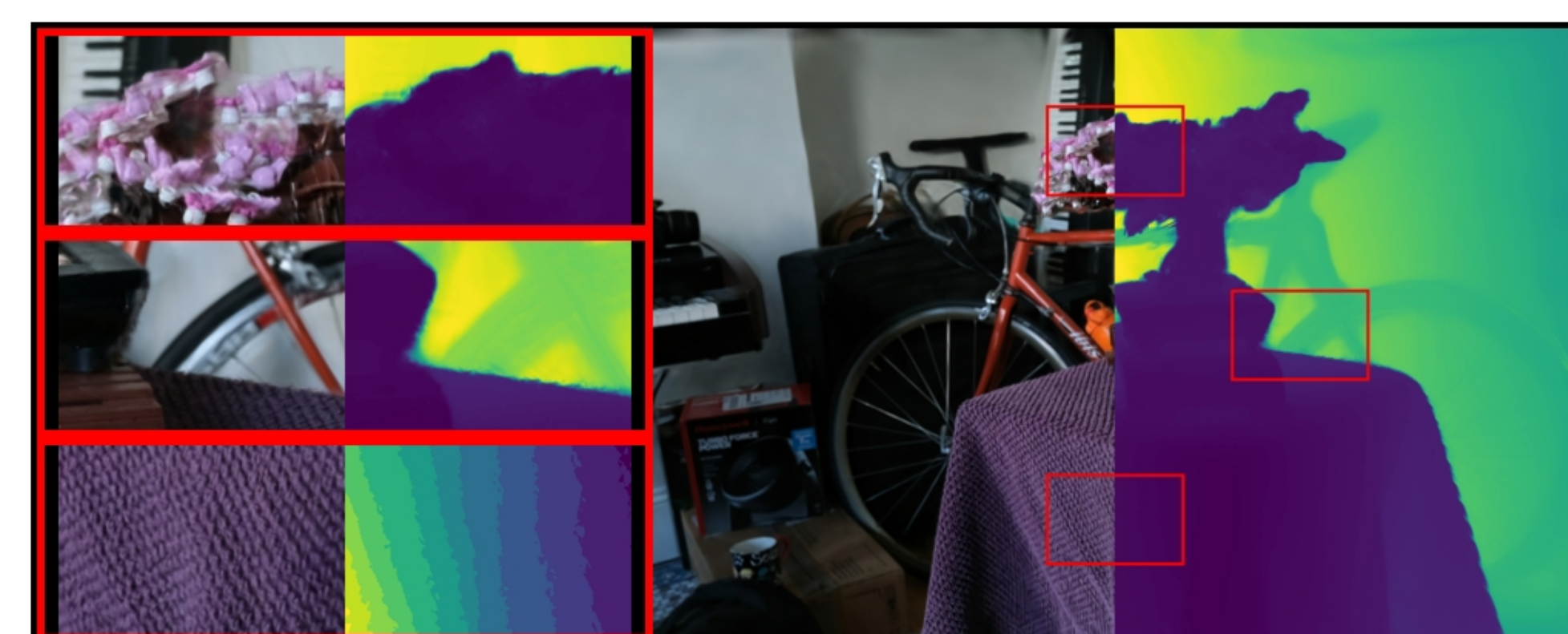
bonsai: VGGT | full | Pose Opt PSNR: 17.47 | LPIPS: 0.3922 | SSIM: 0.5574
