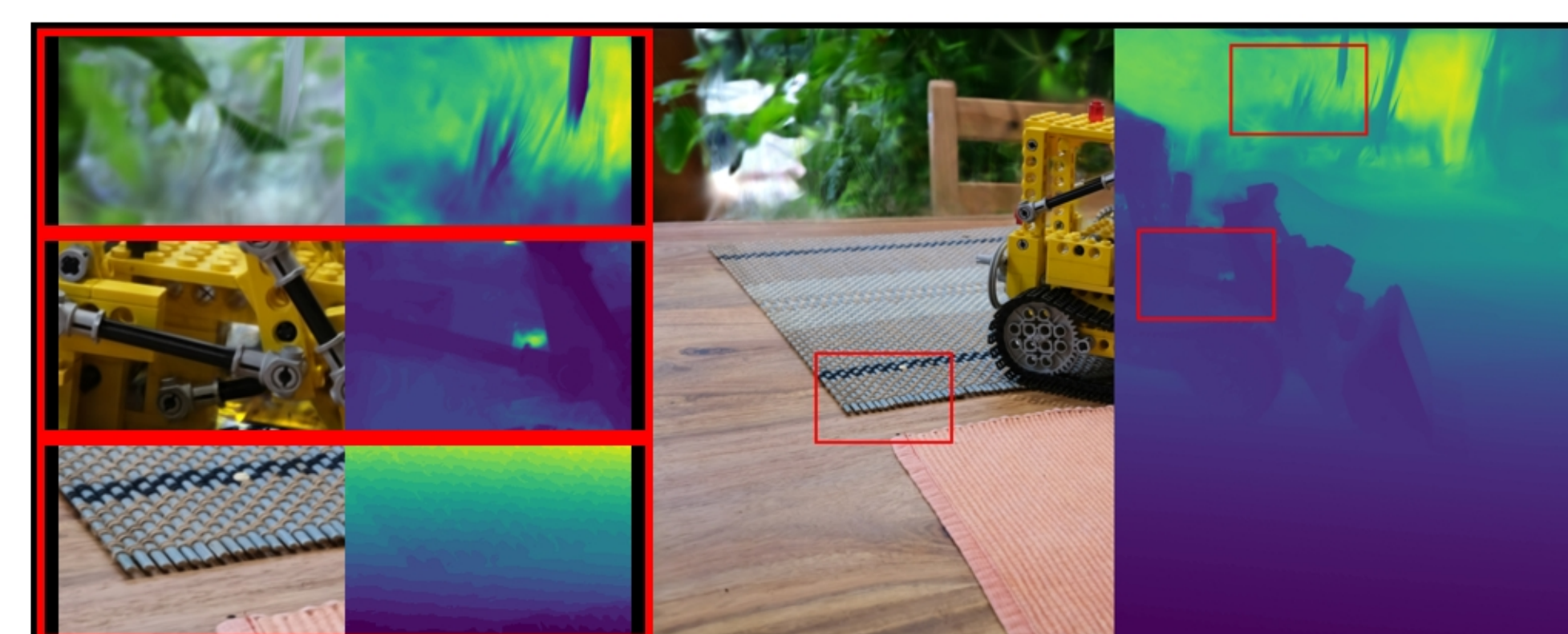
kitchen: VGGT | full | Pose Opt PSNR: 19.04 | LPIPS: 0.2102 | SSIM: 0.4003
