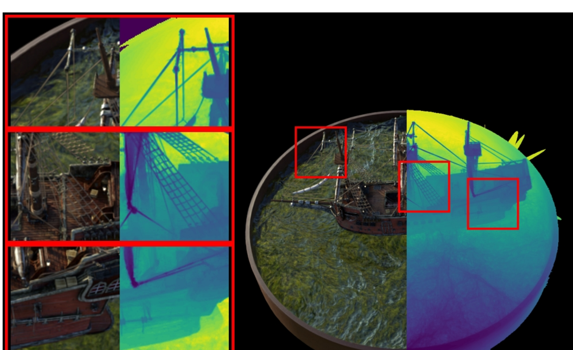
ship: VGGT | Pose Opt PSNR: 22.86 | LPIPS: 0.1296 | SSIM: 0.7485
