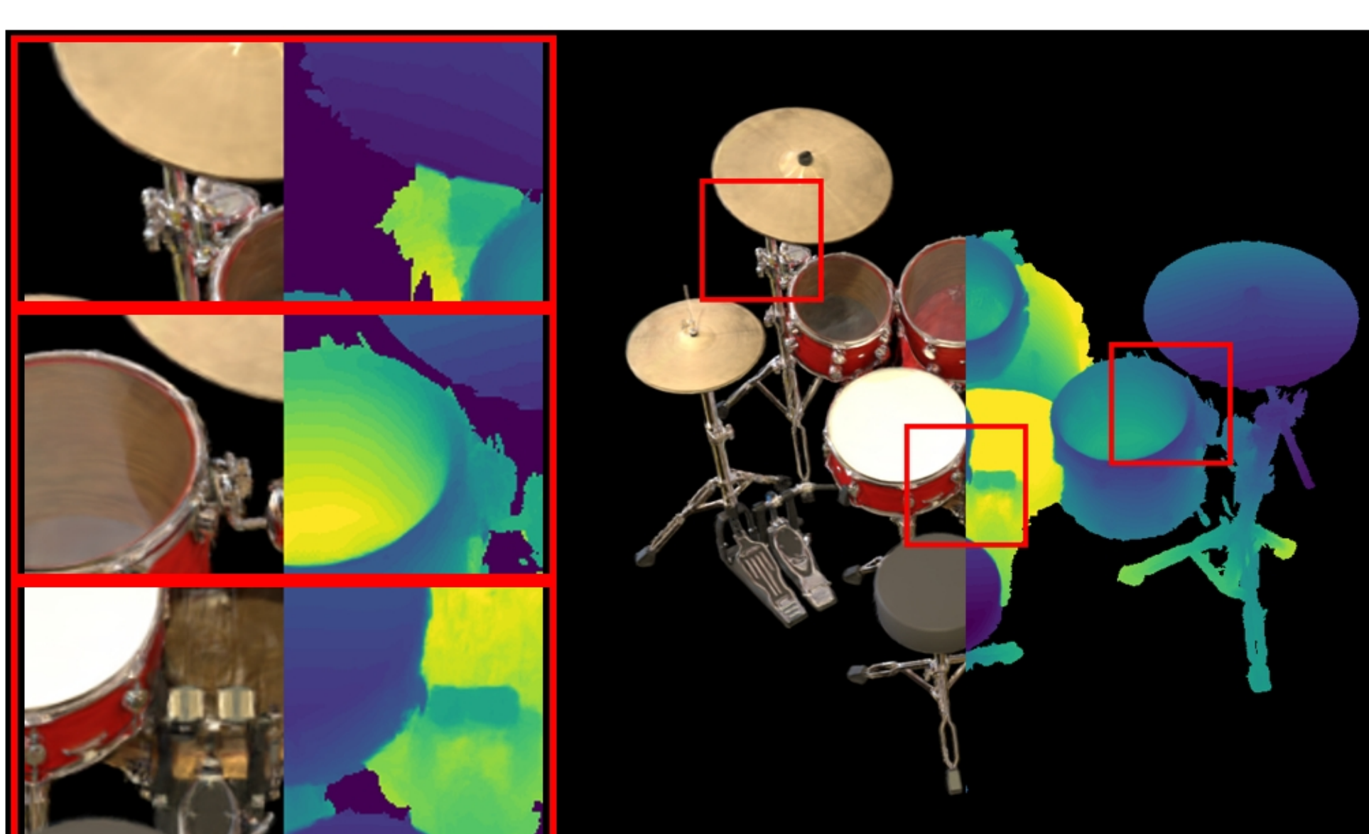
drums: VGGT | full | PSNR: 19.69 | LPIPS: 0.1111 | SSIM: 0.8364
