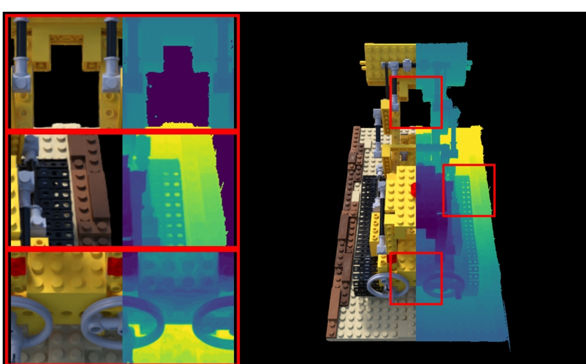
lego: VGGT | Pose Opt PSNR: 20.35 | LPIPS: 0.0759 | SSIM: 0.7735
