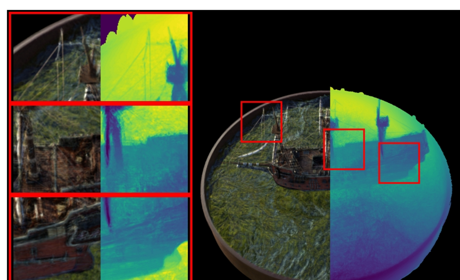
ship: VGGT | closer | PSNR: 20.87 | LPIPS: 0.1919 | SSIM: 0.7020
