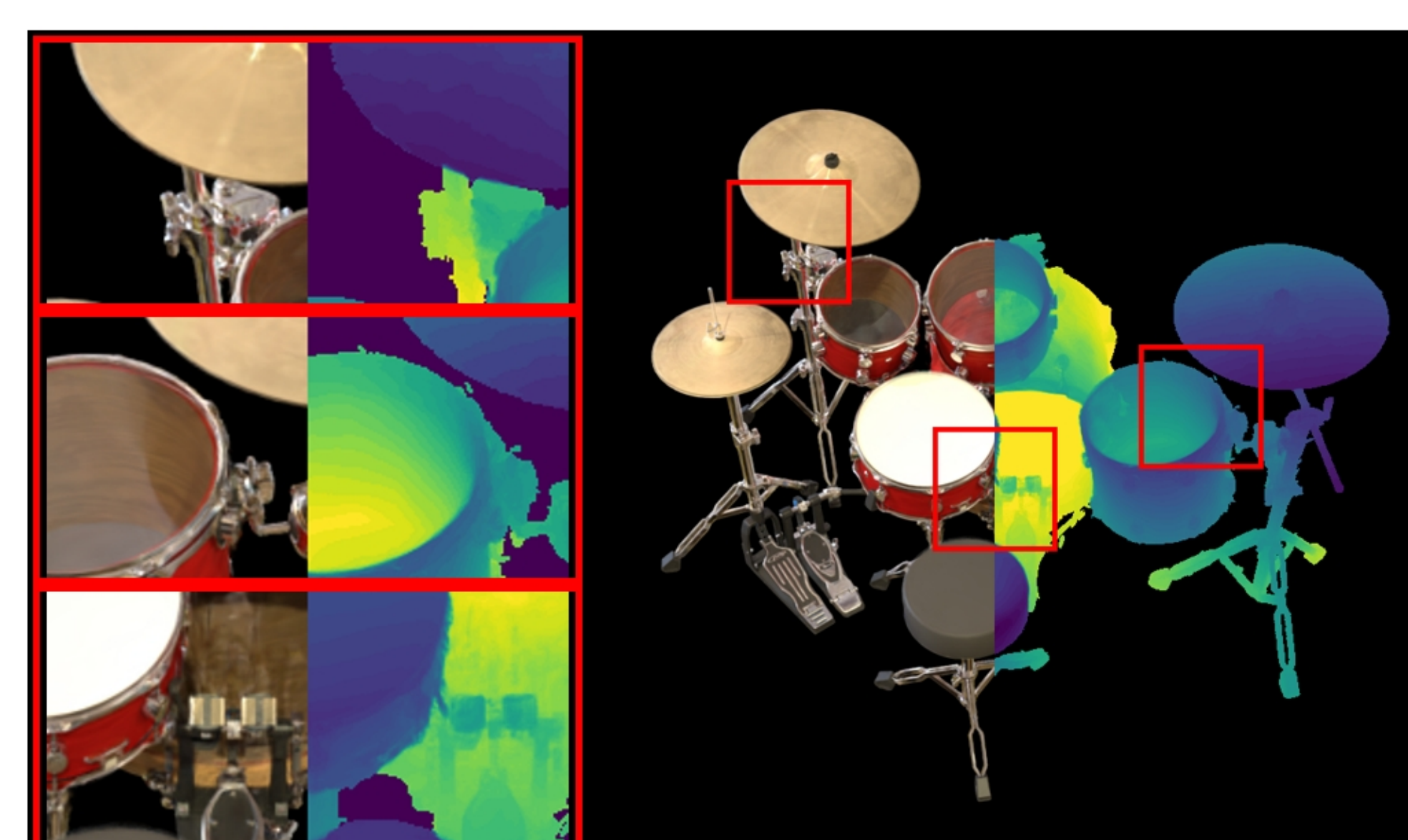
drums: VGGT | closer | Pose Opt PSNR: 20.03 | LPIPS: 0.0915 | SSIM: 0.8510
