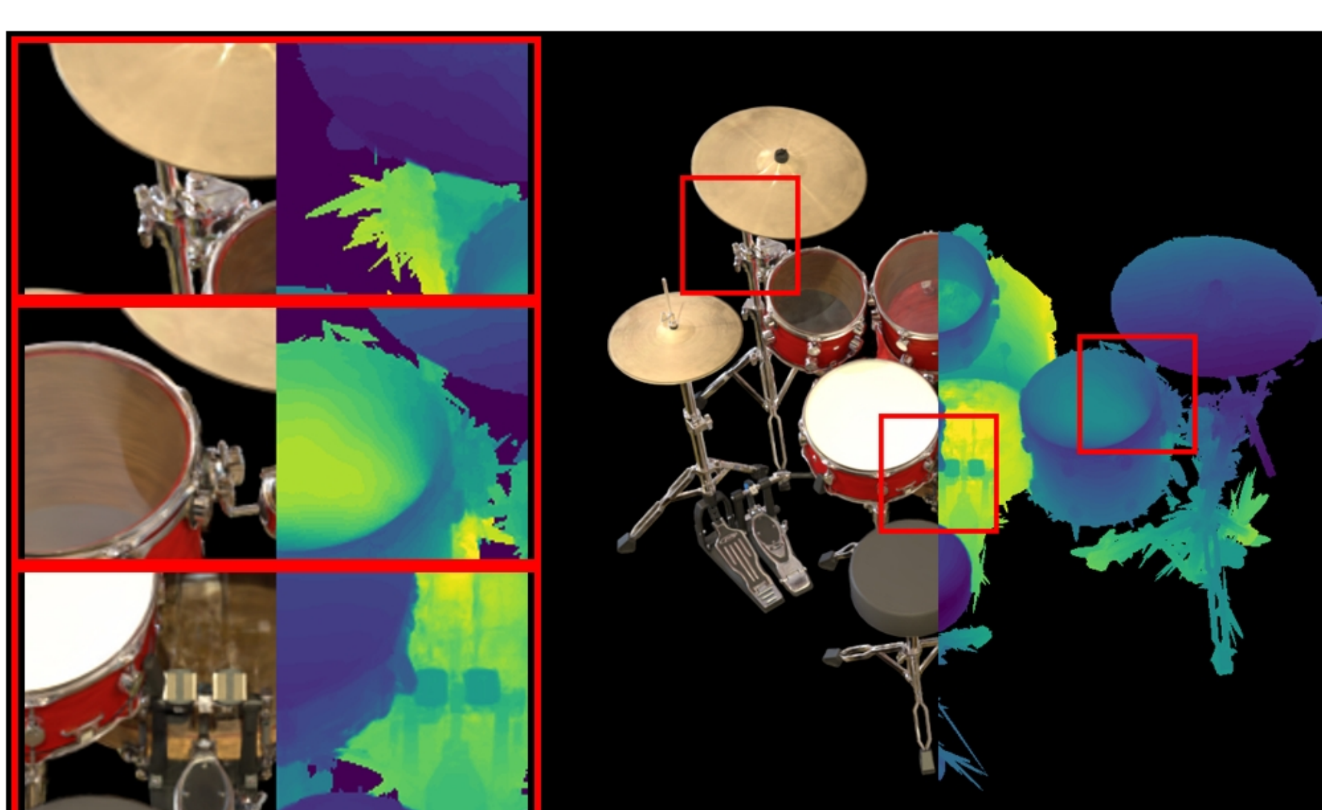
drums: VGGT | Pose Opt PSNR: 20.90 | LPIPS: 0.0848 | SSIM: 0.8690
