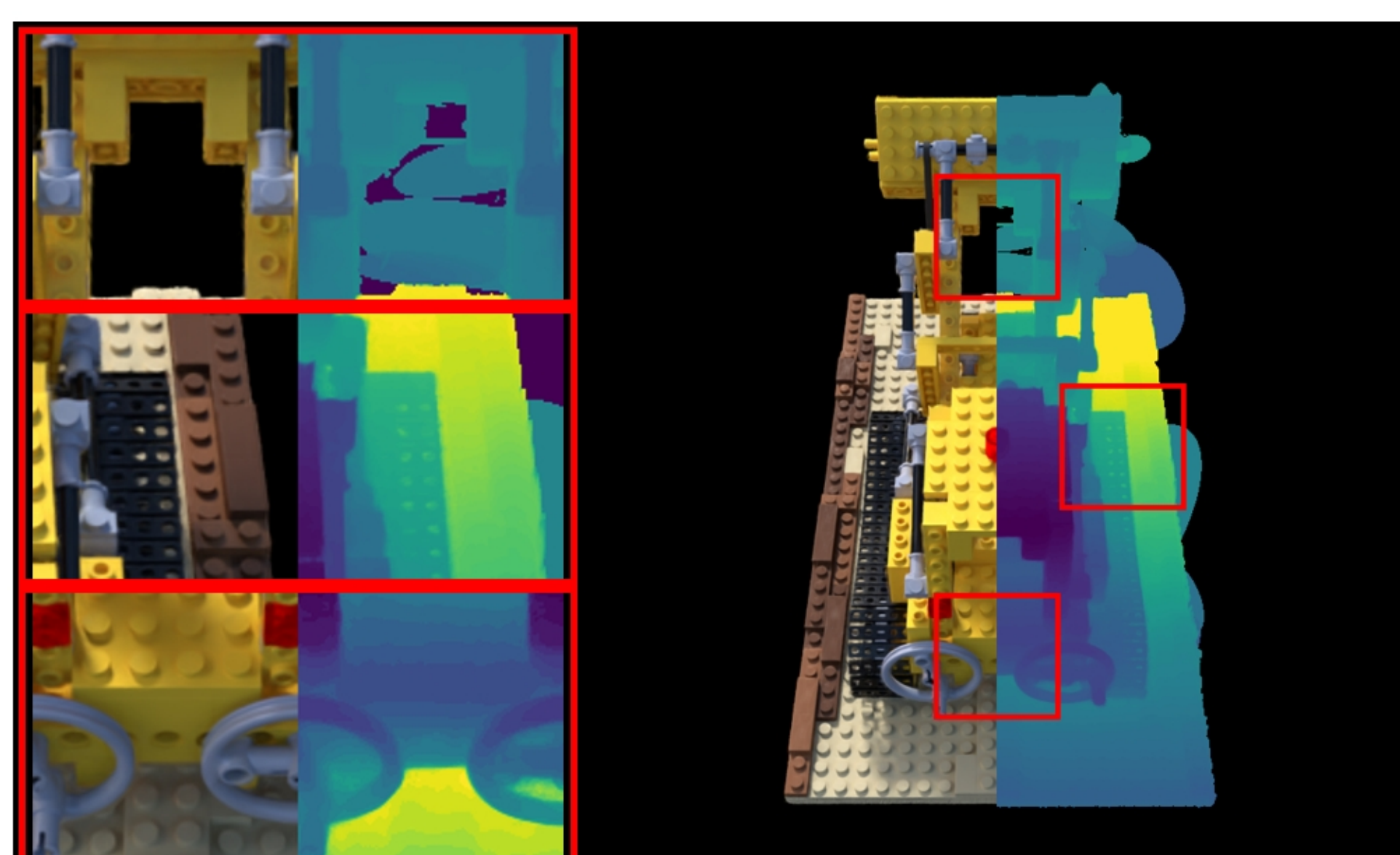
lego: VGGT | full | Pose Opt PSNR: 21.97 | LPIPS: 0.0697 | SSIM: 0.8123
