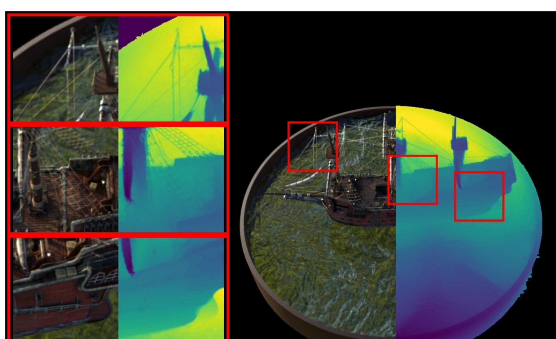
ship: VGGT | full | Pose Opt PSNR: 23.49 | LPIPS: 0.1317 | SSIM: 0.7647
