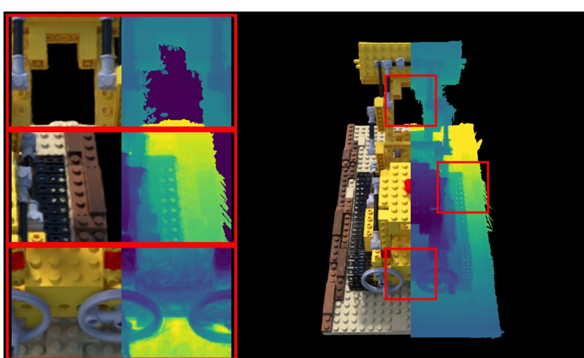
lego: VGGT | PSNR: 20.57 | LPIPS: 0.0950 | SSIM: 0.7737
