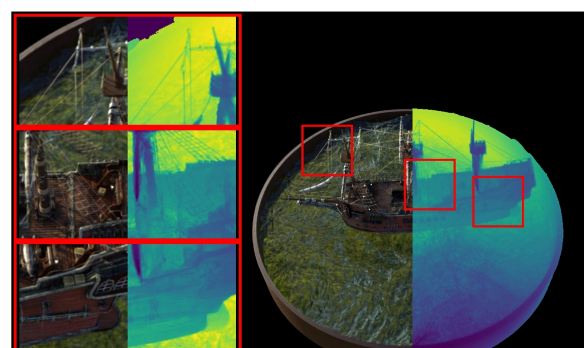
ship: VGGT | closer | Pose Opt PSNR: 22.62 | LPIPS: 0.1390 | SSIM: 0.7433
