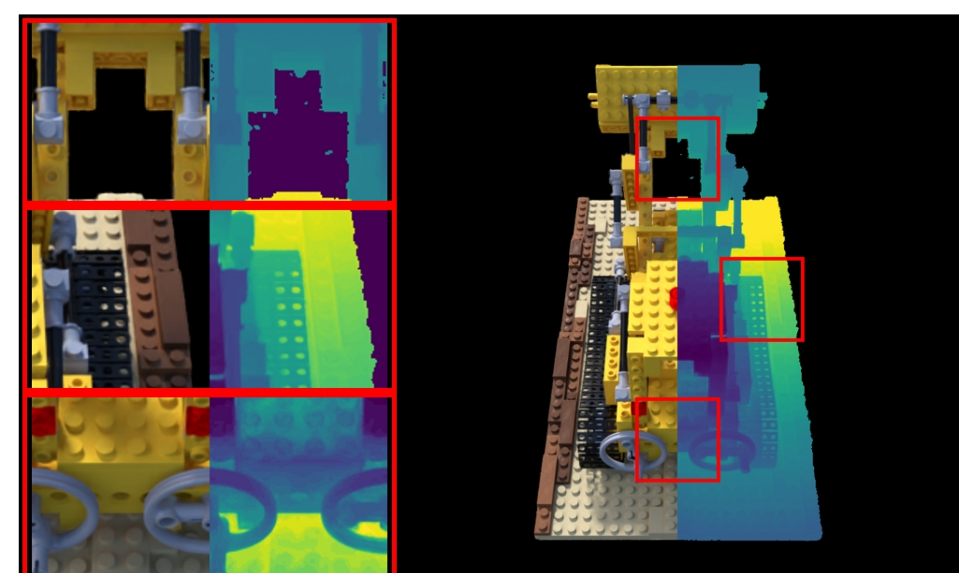
lego: VGGT | closer | Pose Opt PSNR: 20.37 | LPIPS: 0.0786 | SSIM: 0.7747
