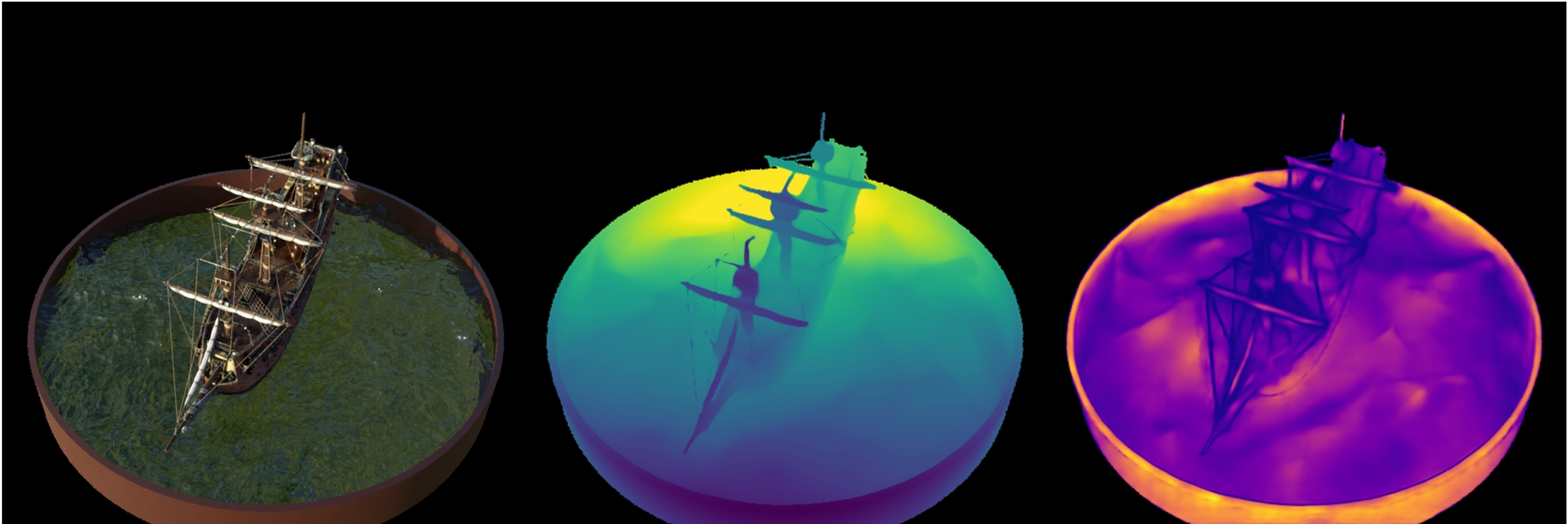
ship: VGGT | Original | Depth (max=1.23) | Confidence (max=146.85)
