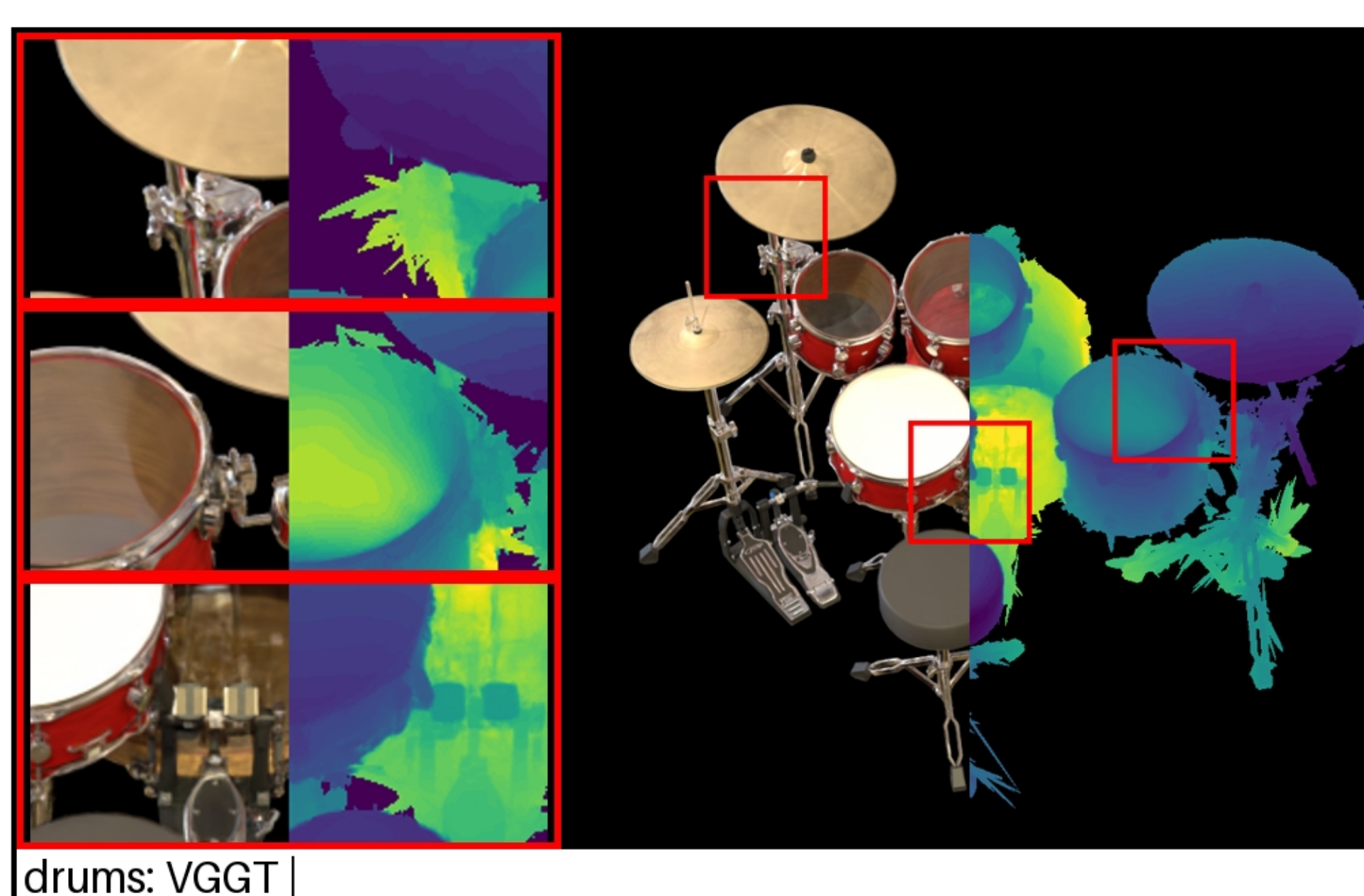
drums: VGGT | PSNR: 20.90 | LPIPS: 0.0848 | SSIM: 0.8690
