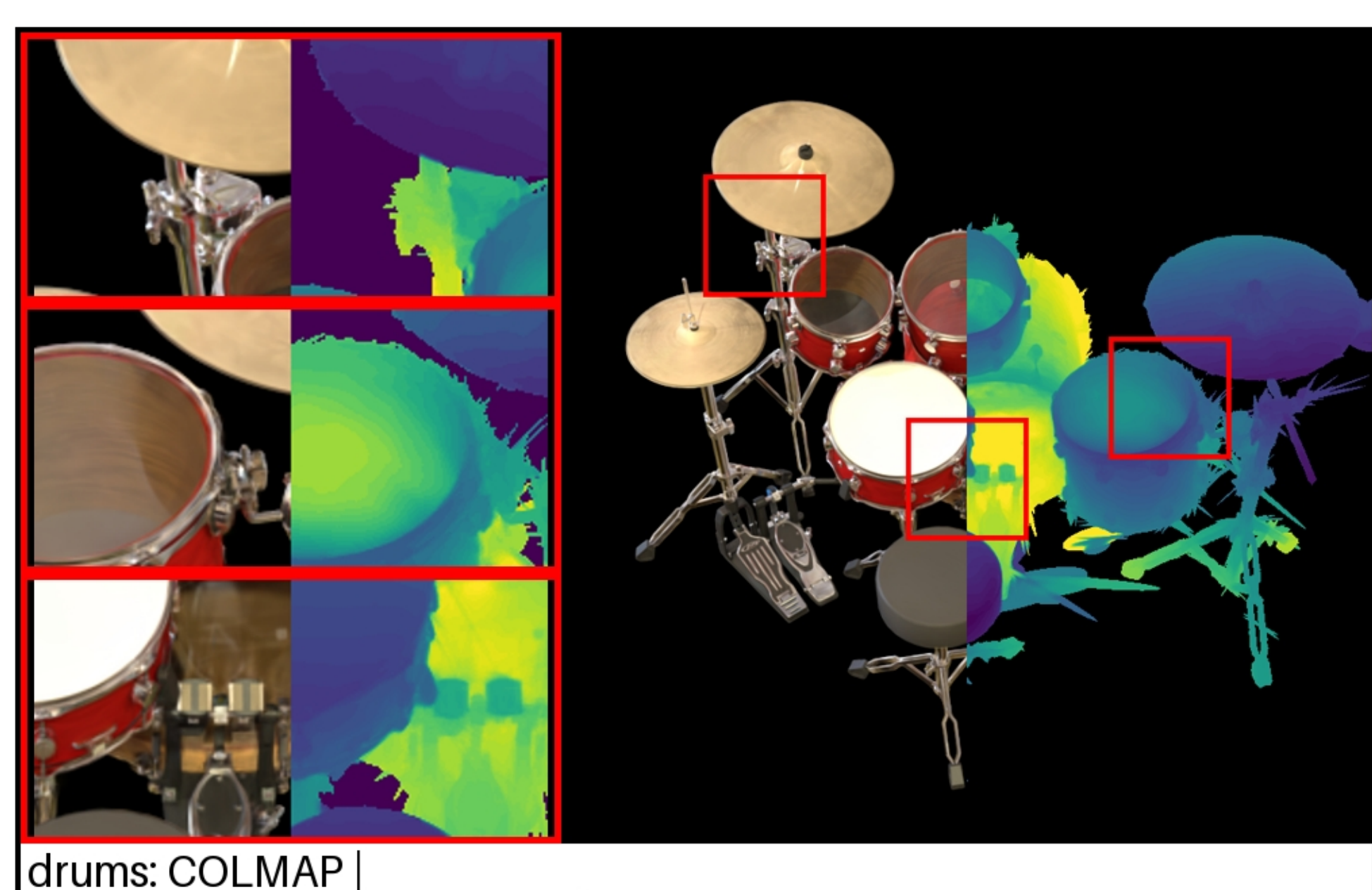
drums: COLMAP | PSNR: 22.80 | LPIPS: 0.0892 | SSIM: 0.9061
