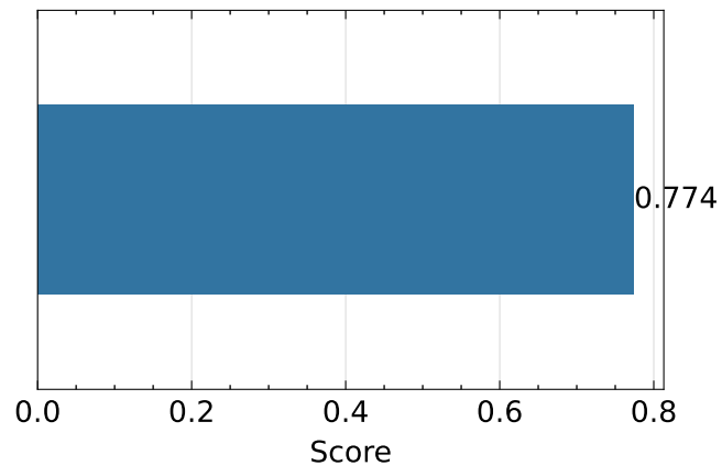
Composite Quality ↑
