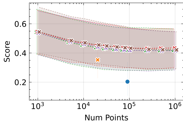
LPIPS \downarrow
