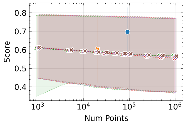
SSIM \uparrow
