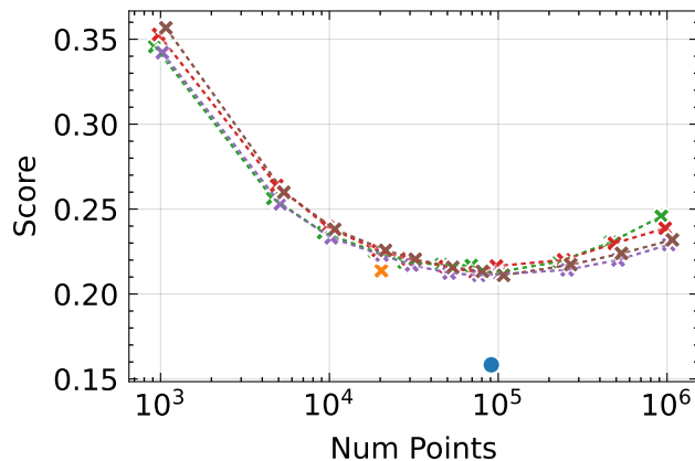
LPIPS \downarrow
