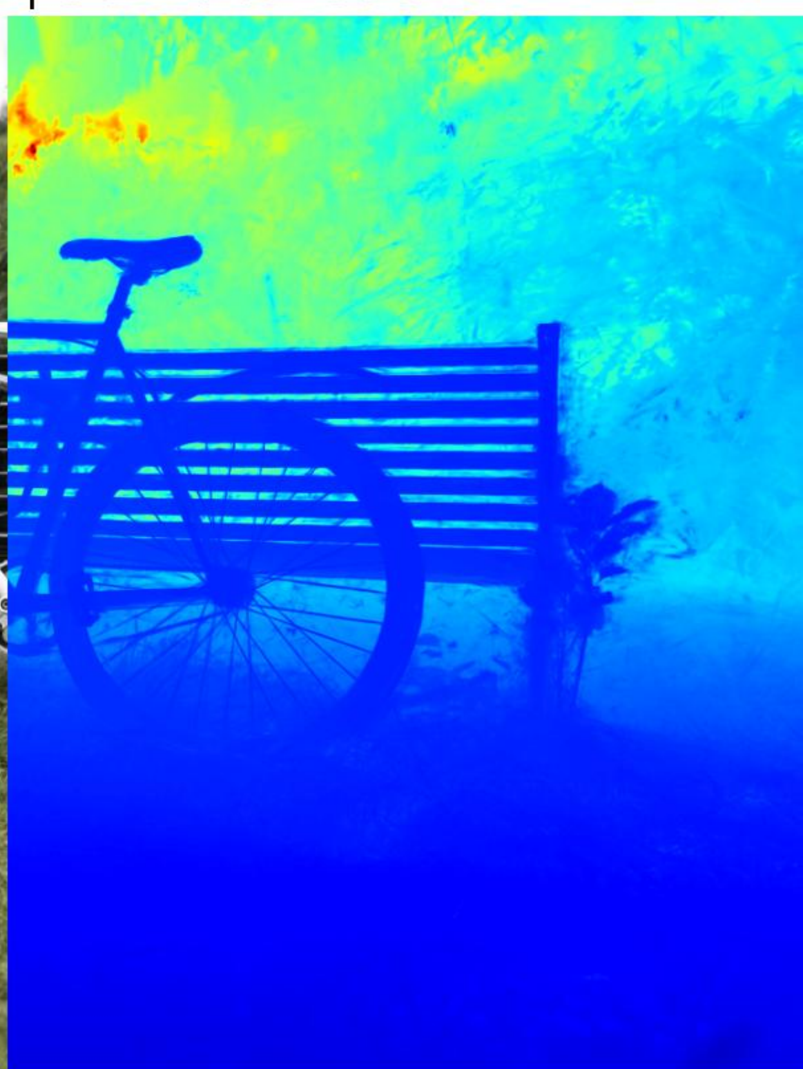
Config: VGGT | standard | points | depth_lambda=0.01 PSNR: 16.76 | LPIPS: 0.3743 | SSIM: 0.2539
