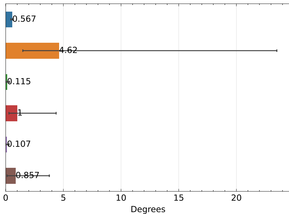
Aligned Cameras ↑
