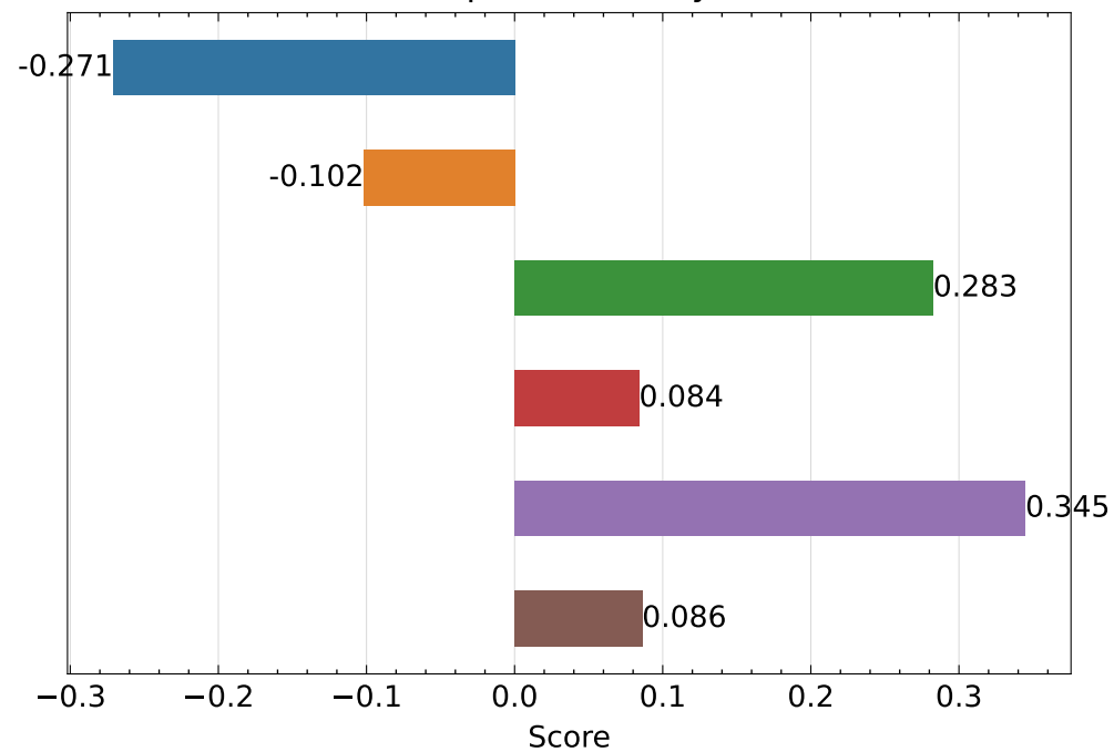
Composite Quality ↑
