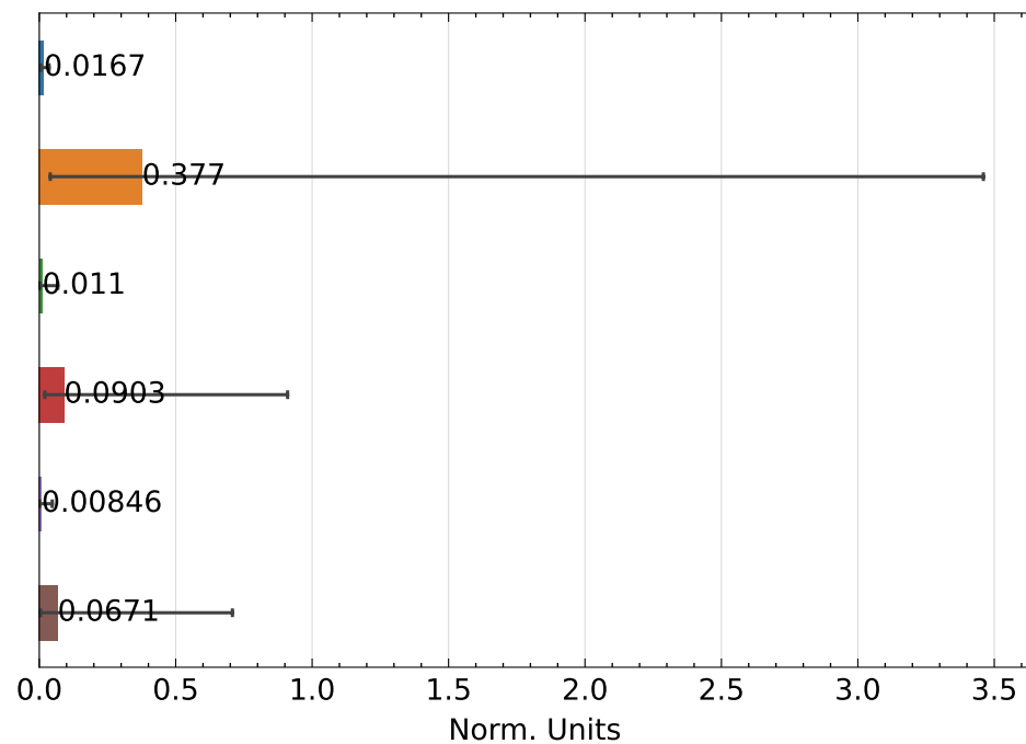
Composite Quality ↑
