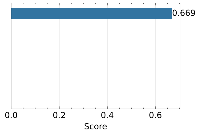
Composite Quality ↑
