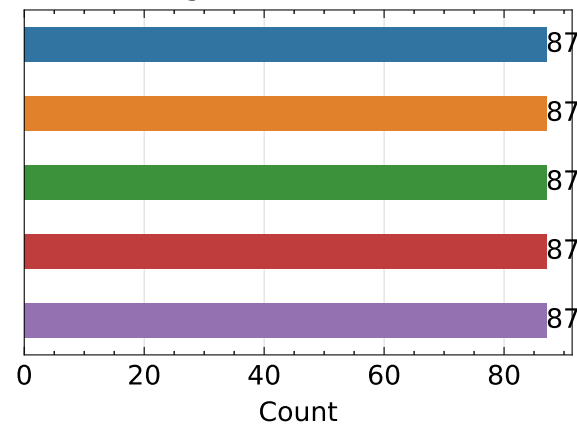
Composite Quality ↑
