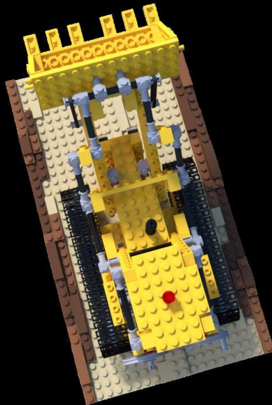
Ground Truth
