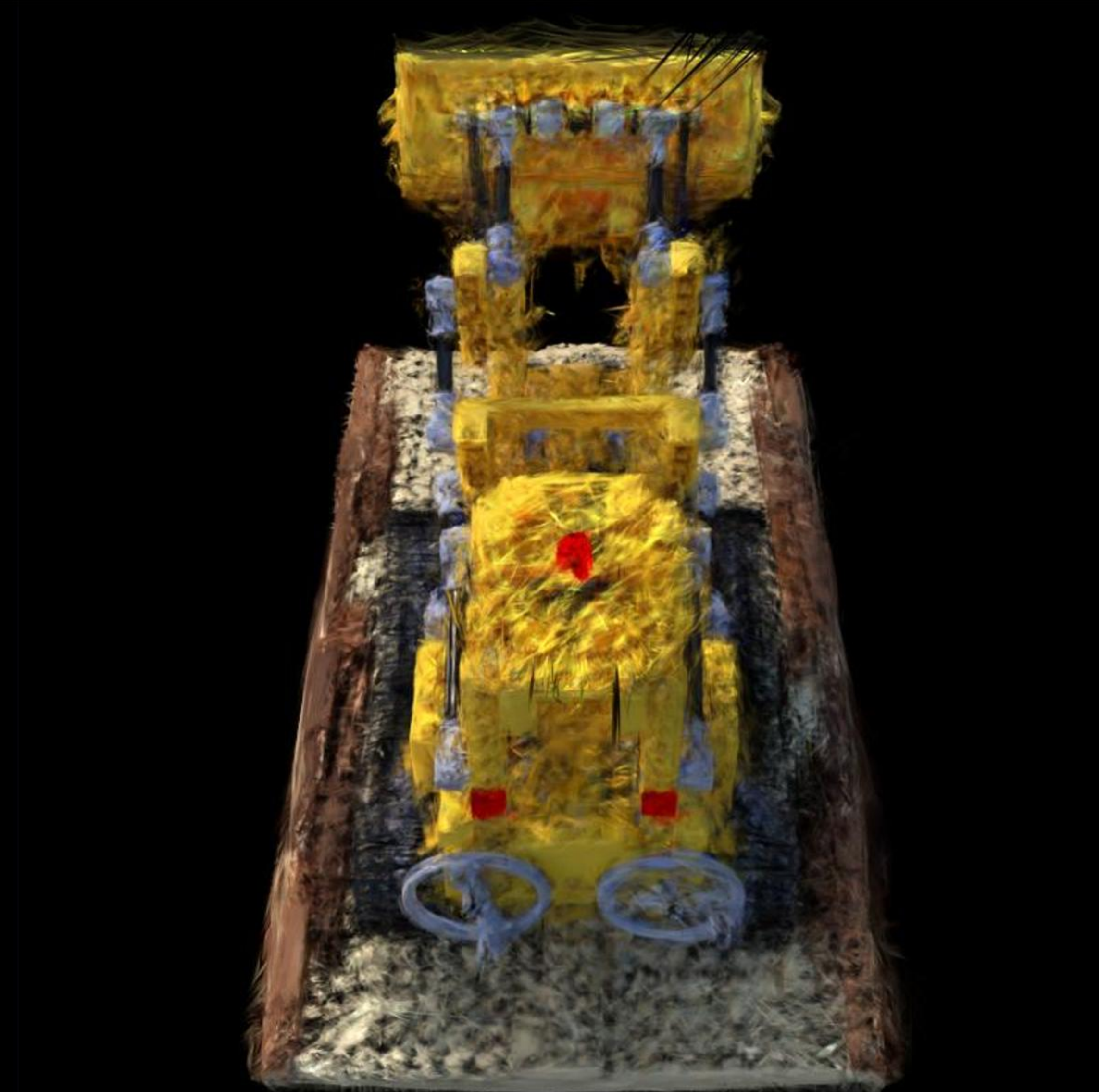
Config: VGGT | Pose Opt | num_images=40 PSNR: 15.11 | LPIPS: 0.3085 | SSIM: 0.6135
