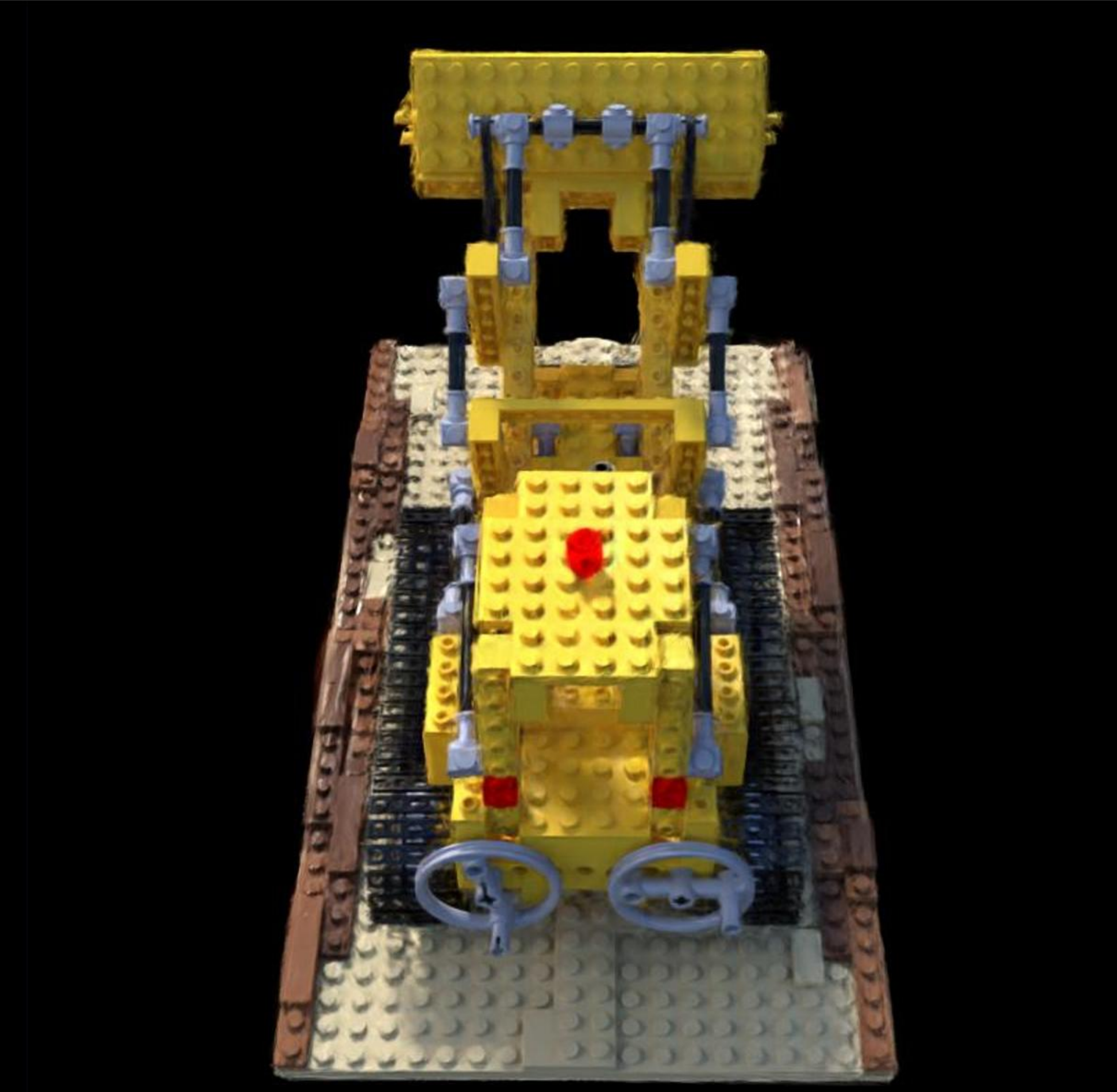
Config: VGGT | Pose Opt | num_images=100 PSNR: 15.09 | LPIPS: 0.2566 | SSIM: 0.6636
