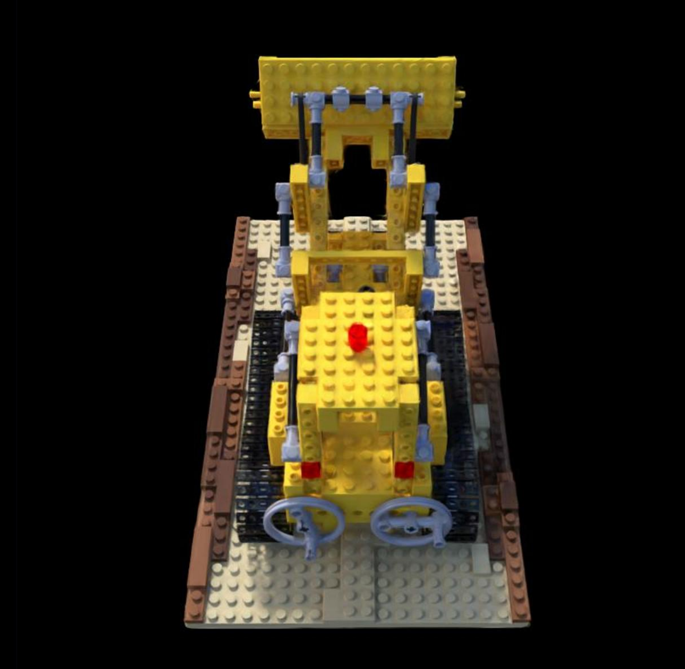
Config: COLMAP | Pose Opt | num_images=100 PSNR: 24.84 | LPIPS: 0.0798 | SSIM: 0.8807
