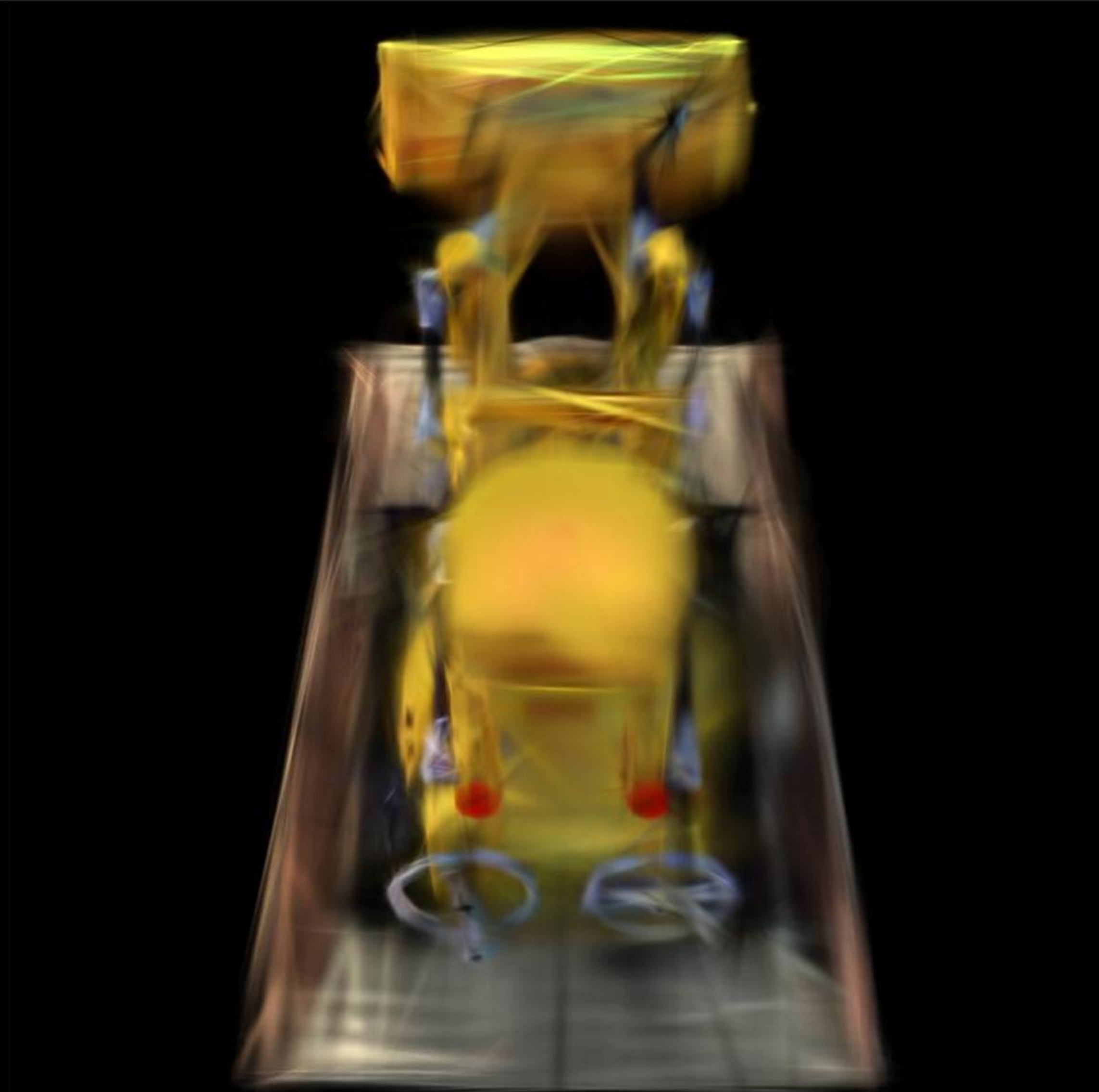
Config: VGGT | Pose Opt | num_images=30 PSNR: 15.13 | LPIPS: 0.3705 | SSIM: 0.6605
