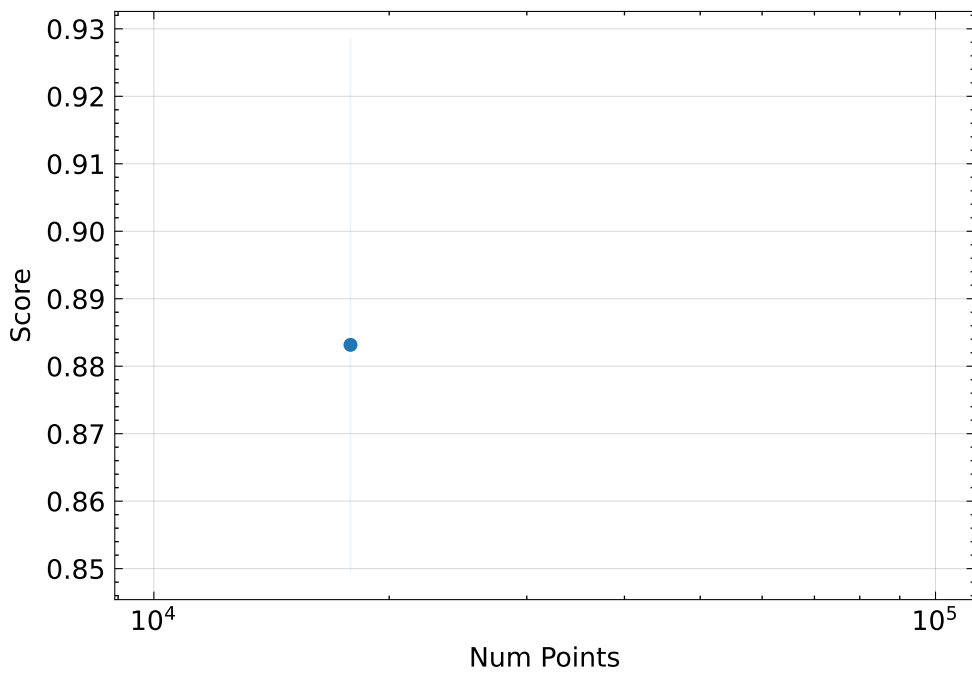
SSIM \uparrow
