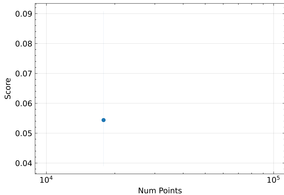
LPIPS \downarrow
