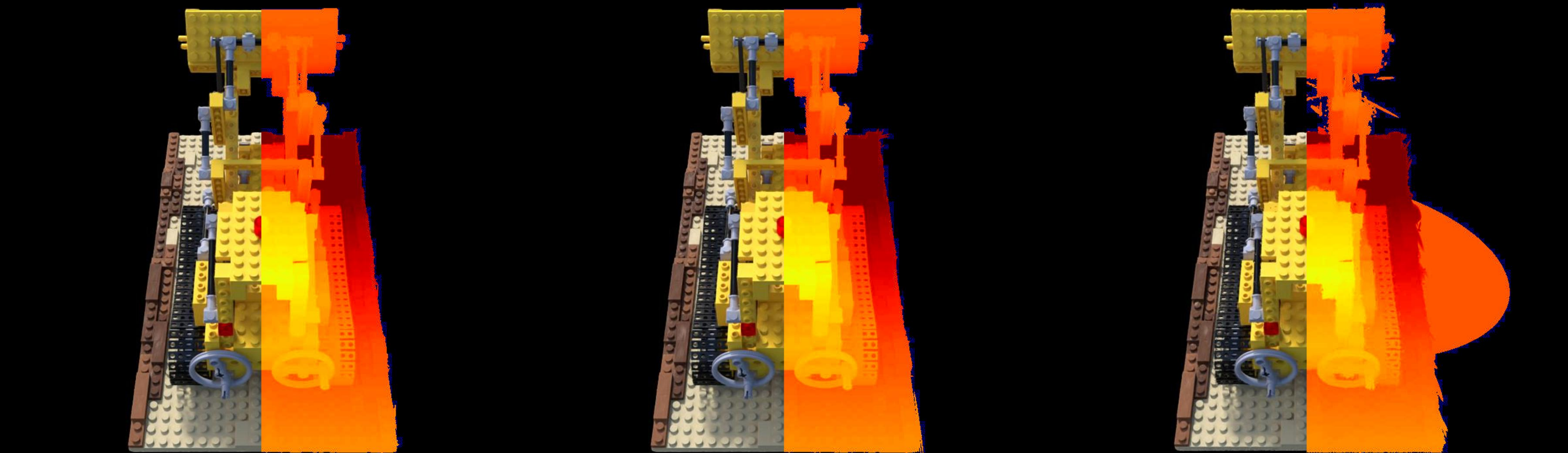
Config: VGGT | sigmoid | depth_lambda=0.0 PSNR: 26.01 | LPIPS: 0.0446 | SSIM: 0.9335
