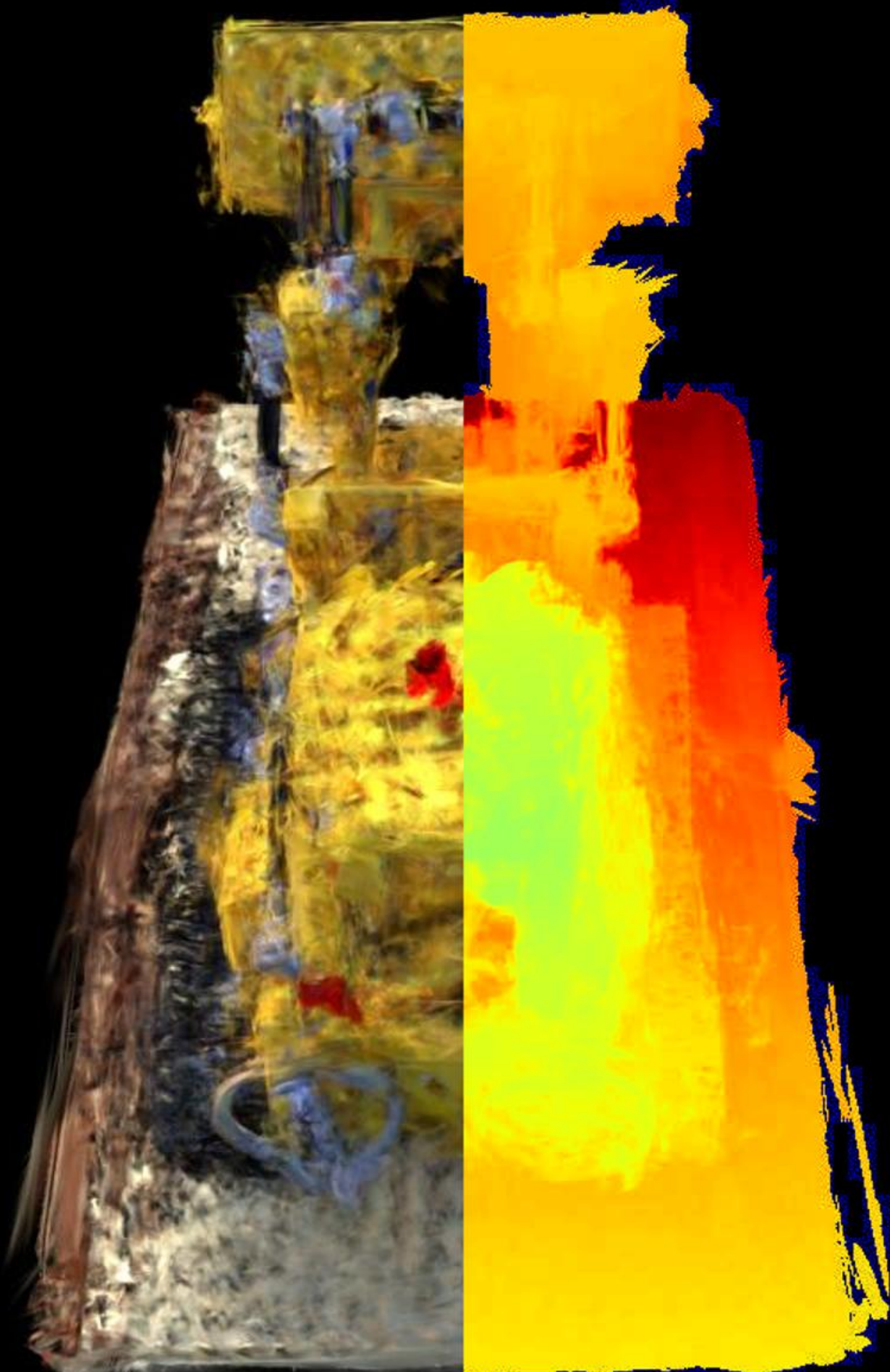
Config: VGGT | 0.0 | num_images=30 PSNR: 14.54 | LPIPS: 0.3166 | SSIM: 0.6293
