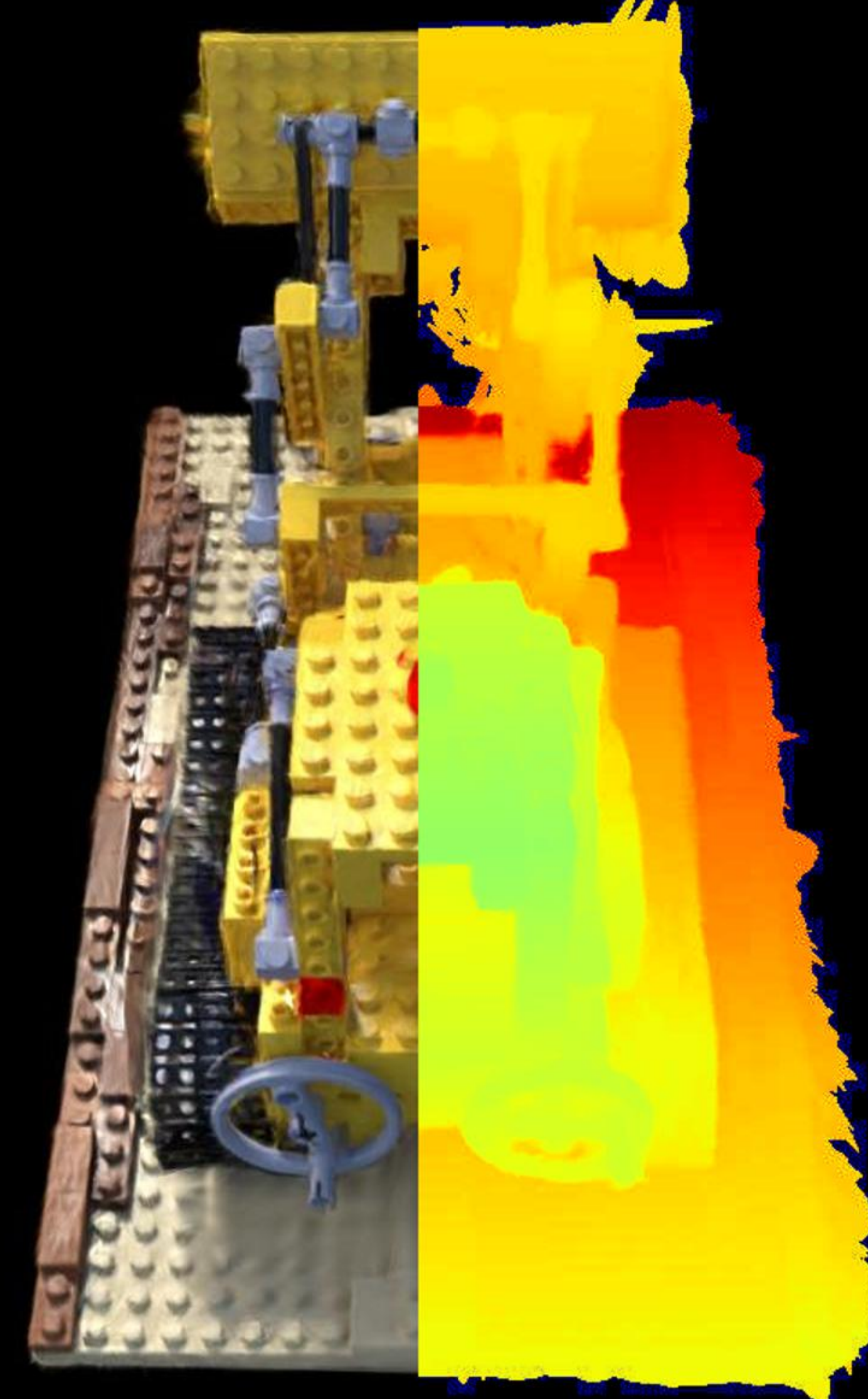
Config: VGGT | 1.0 | num_images=40 PSNR: 15.33 | LPIPS: 0.2650 | SSIM: 0.6685
