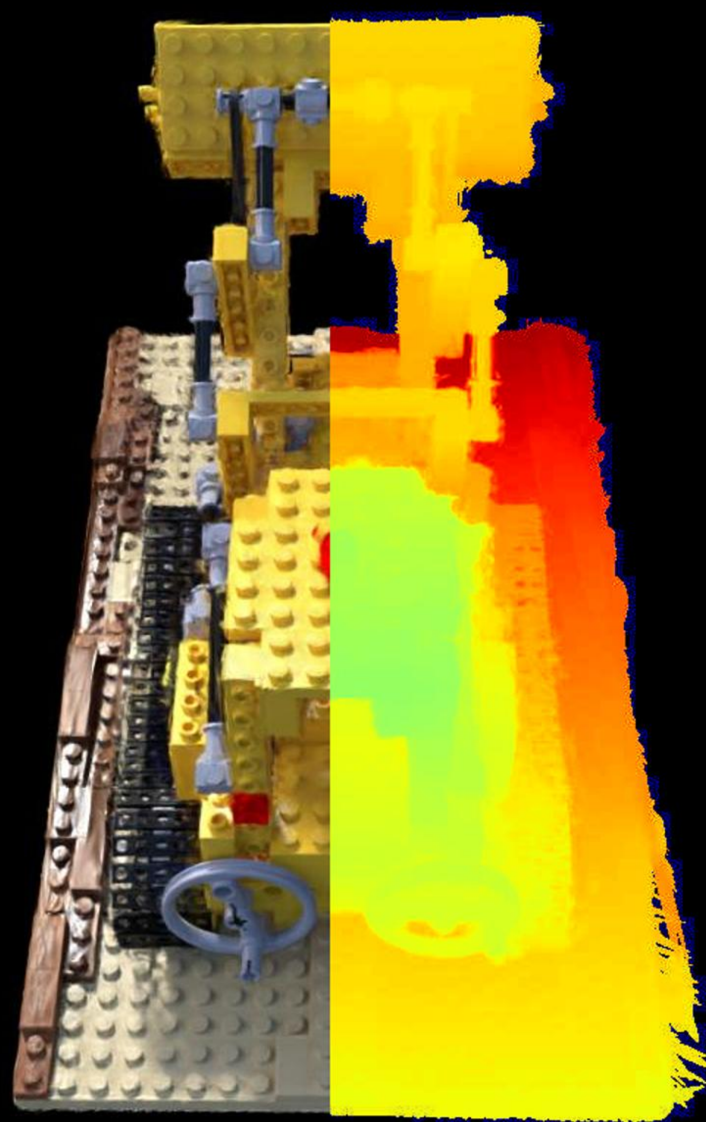
Config: VGGT | 0.01 | num_images=40 PSNR: 15.02 | LPIPS: 0.2549 | SSIM: 0.6617
