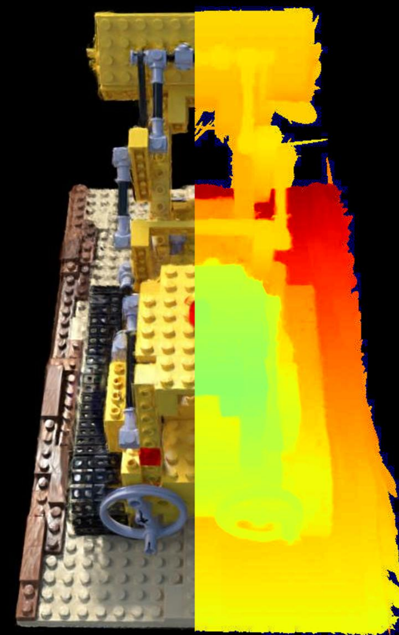
Config: VGGT | 0.1 | num_images=40 PSNR: 15.20 | LPIPS: 0.2522 | SSIM: 0.6638
