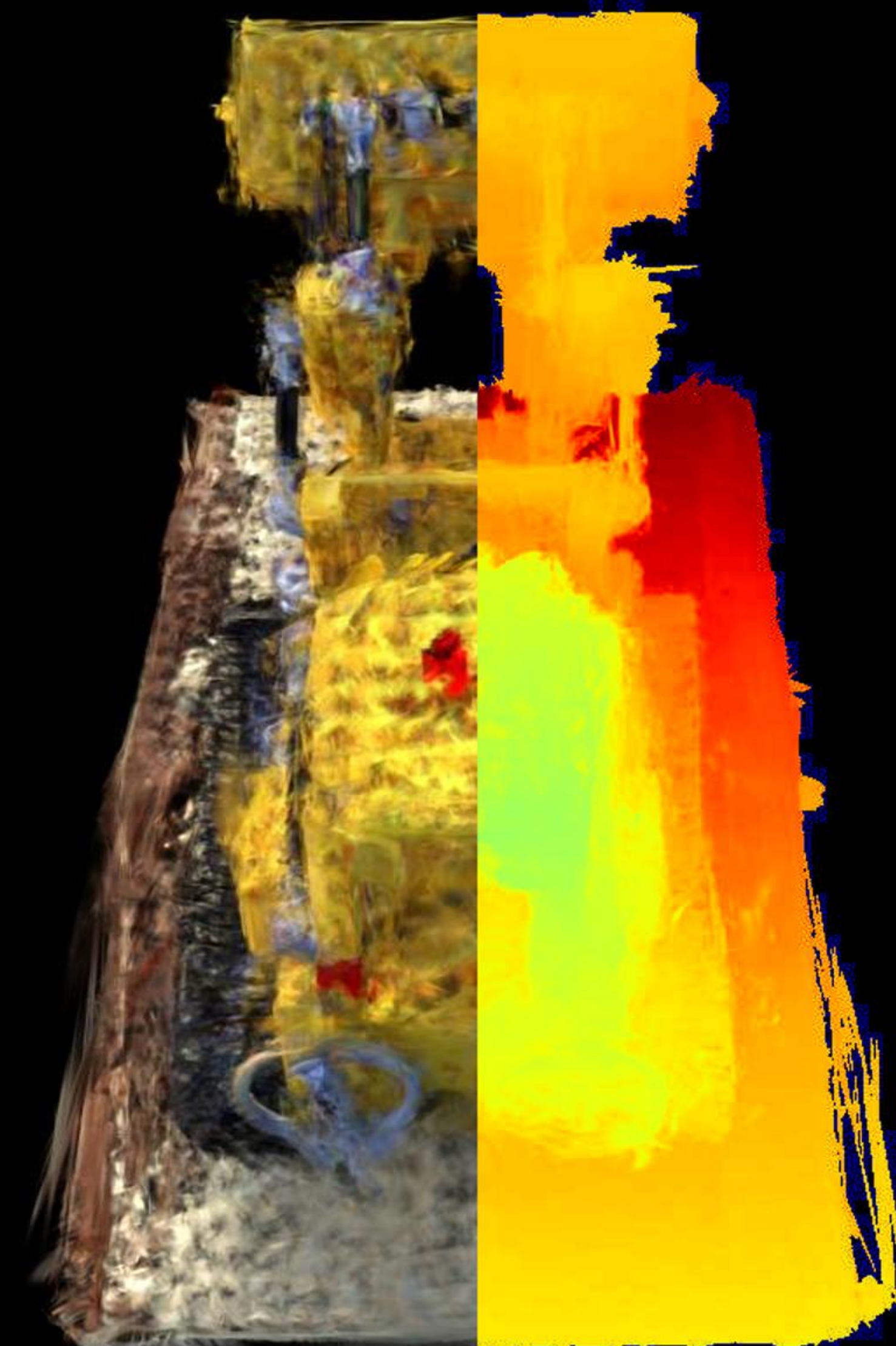
Config: VGGT | 0.01 | num_images=30 PSNR: 14.58 | LPIPS: 0.3130 | SSIM: 0.6308
