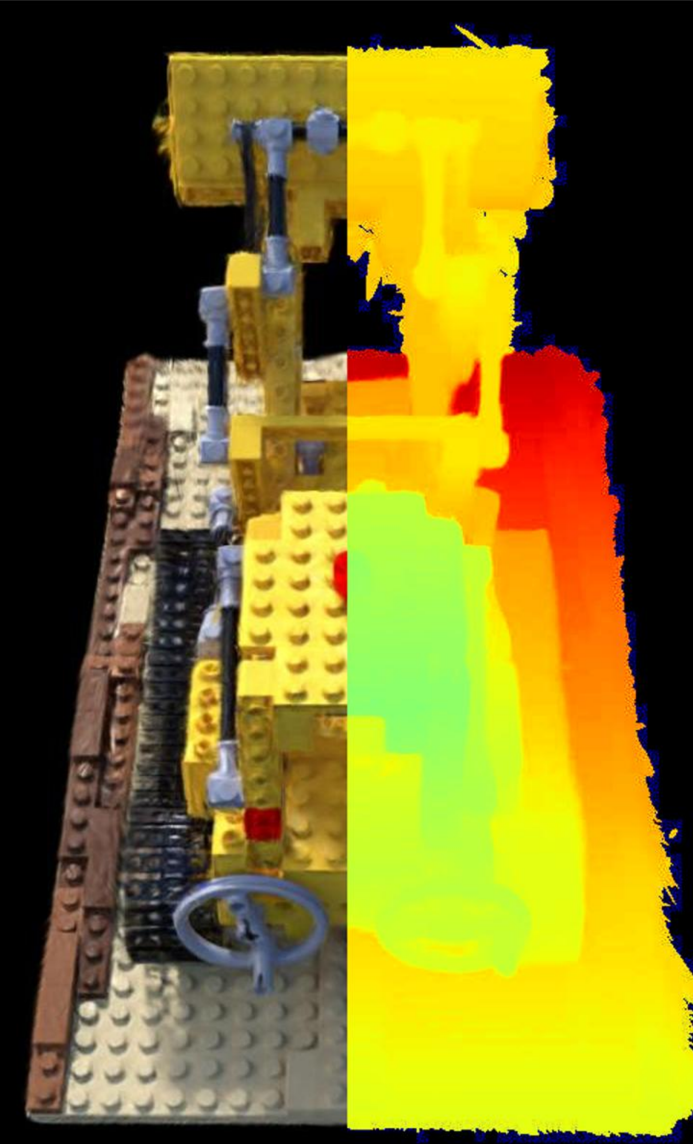
Config: VGGT | 1.0 | num_images=100 PSNR: 15.26 | LPIPS: 0.2628 | SSIM: 0.6662
