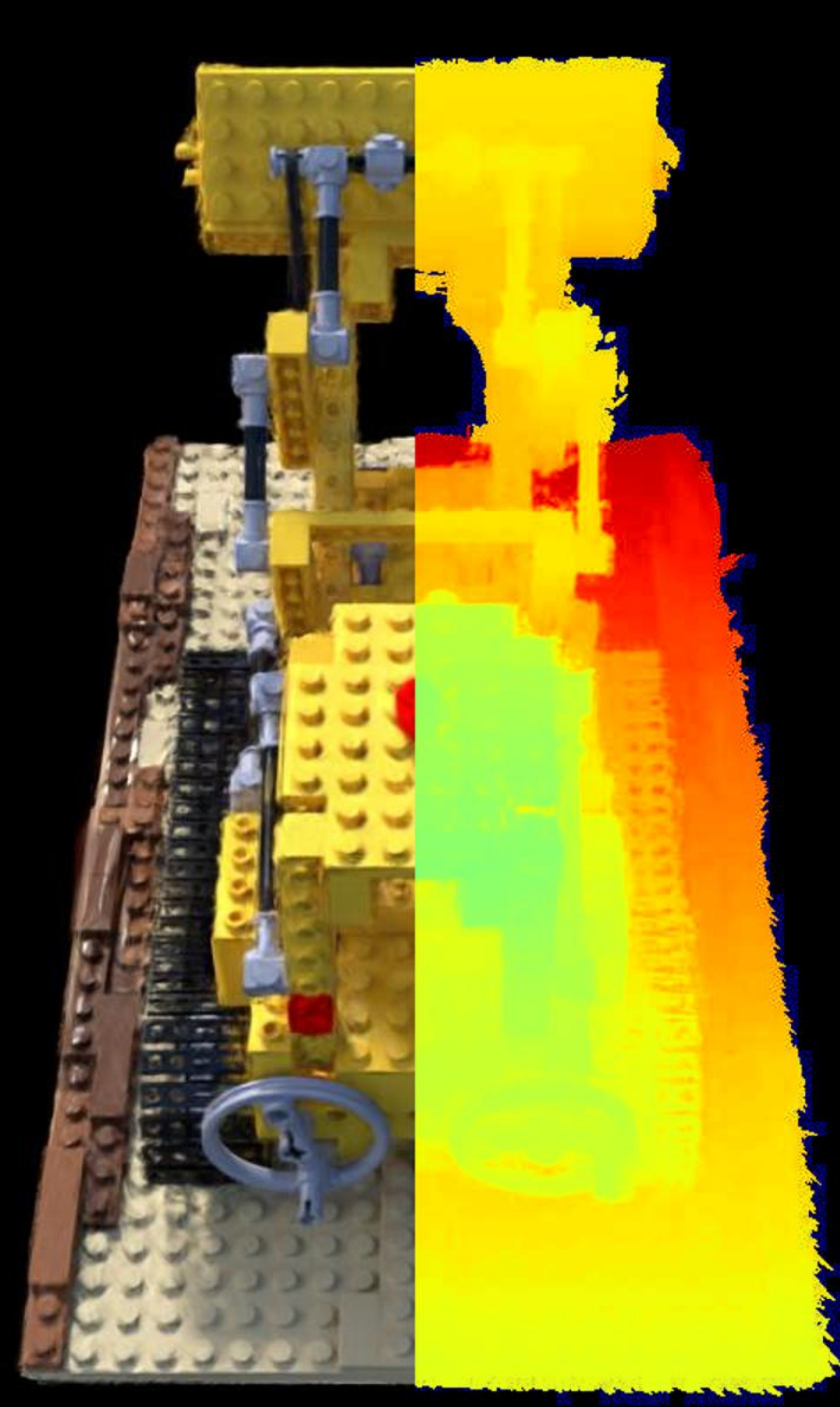
Config: VGGT | 0.0 | num_images=100 PSNR: 15.16 | LPIPS: 0.2529 | SSIM: 0.6653
