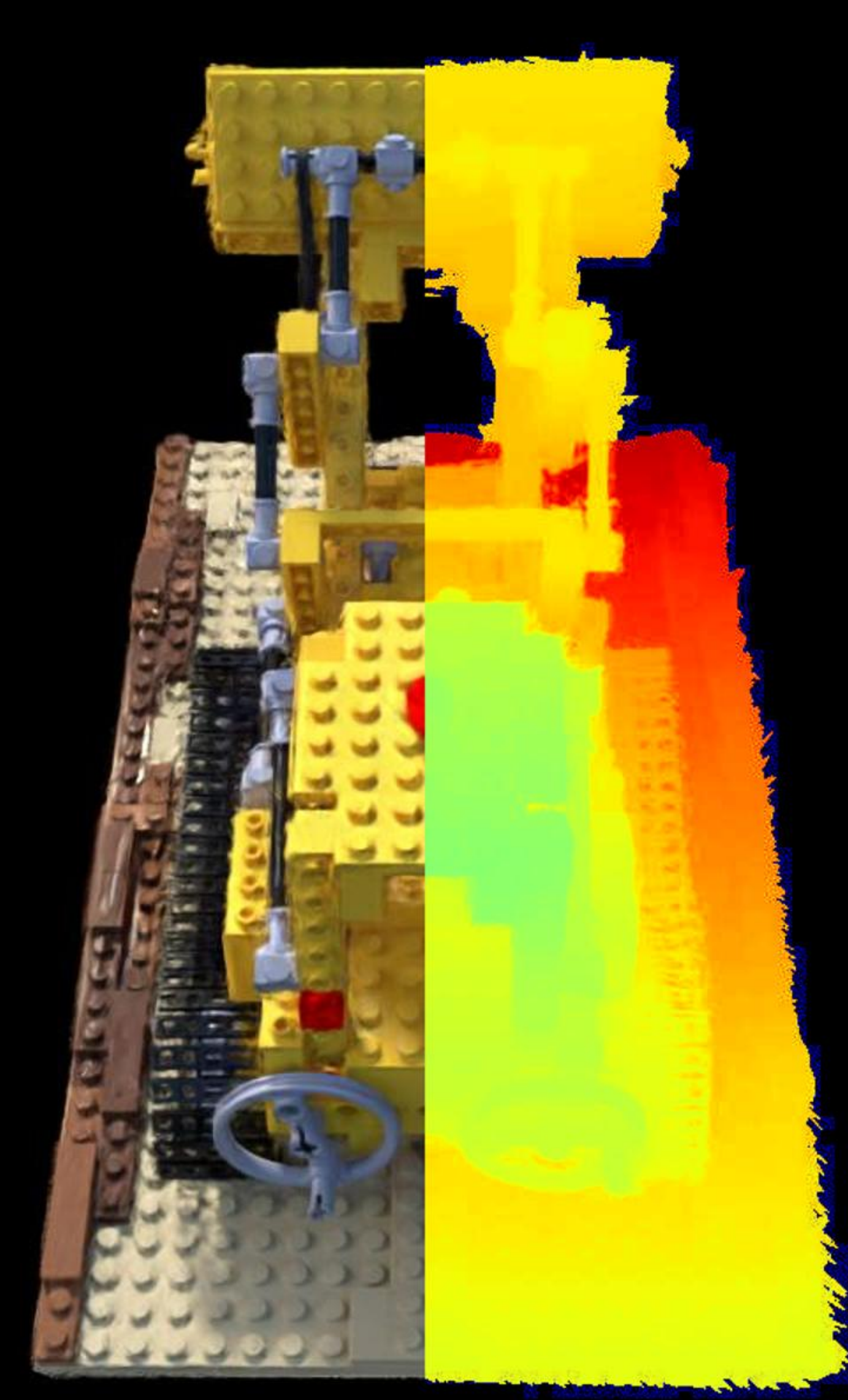
Config: VGGT | 0.01 | num_images=100 PSNR: 15.18 | LPIPS: 0.2532 | SSIM: 0.6660
