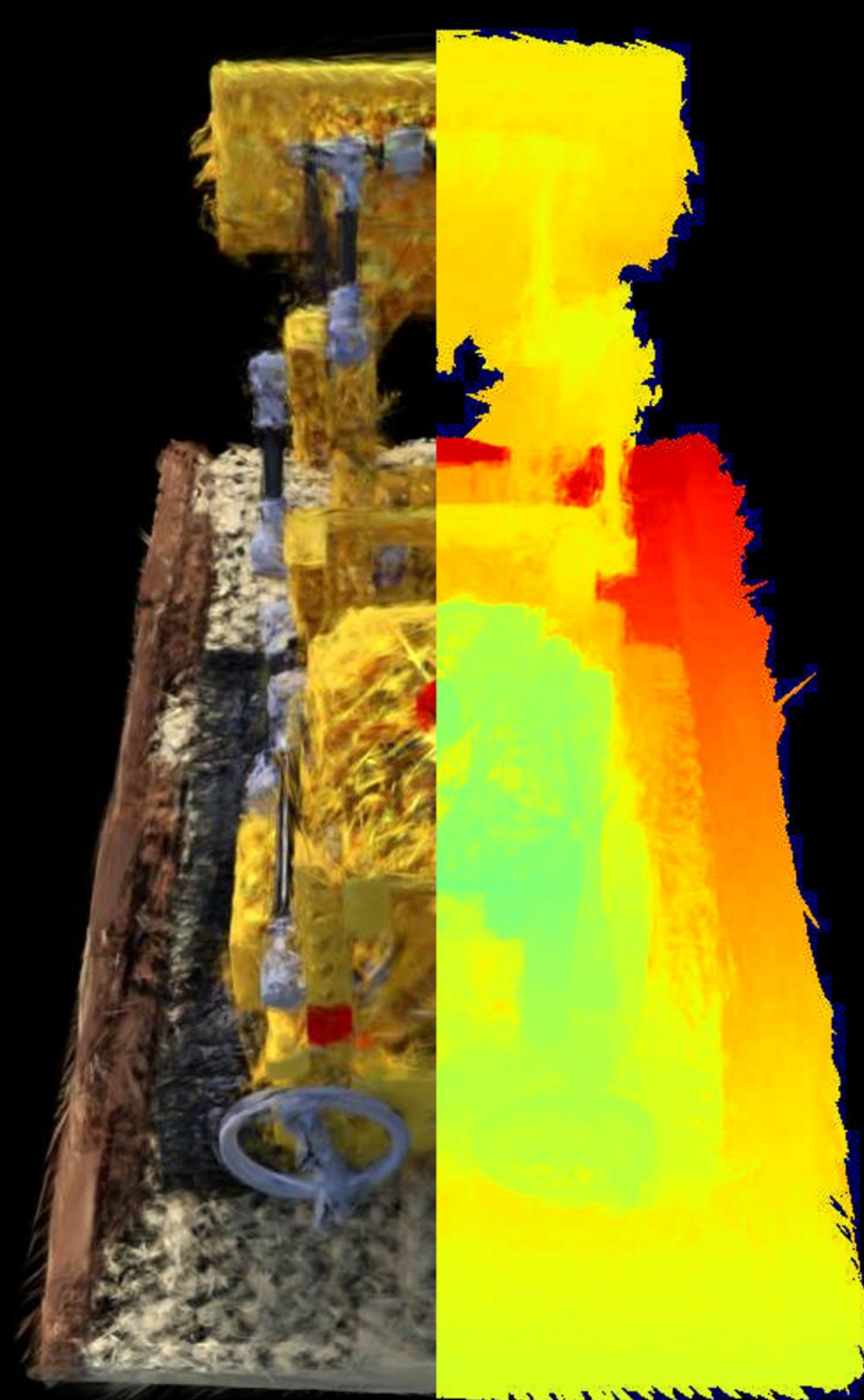
Config: VGGT | 0.01 | num_images=40 PSNR: 15.01 | LPIPS: 0.3001 | SSIM: 0.6256
