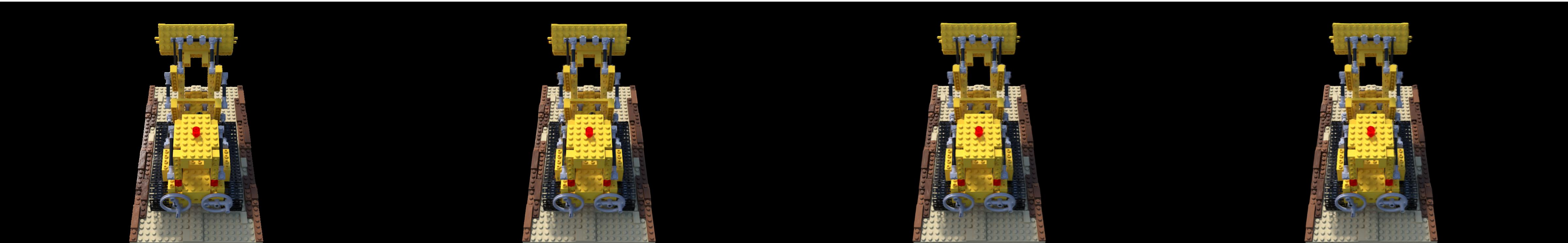
Ground Truth
