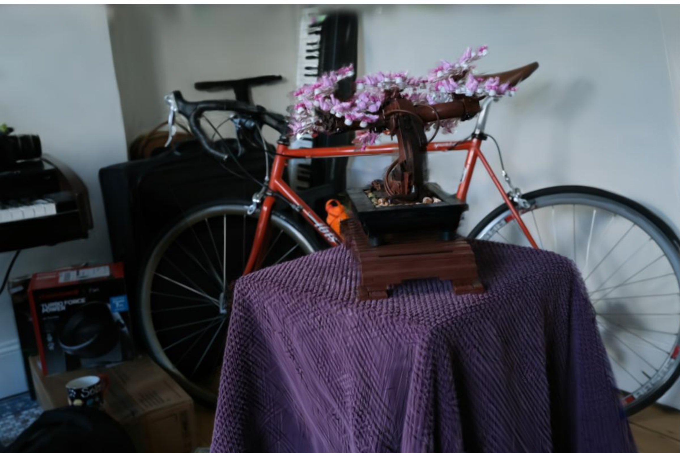
Config: VGGT | Random Init | | Use BA PSNR: 17.74 | LPIPS: 0.3604 | SSIM: 0.5683
