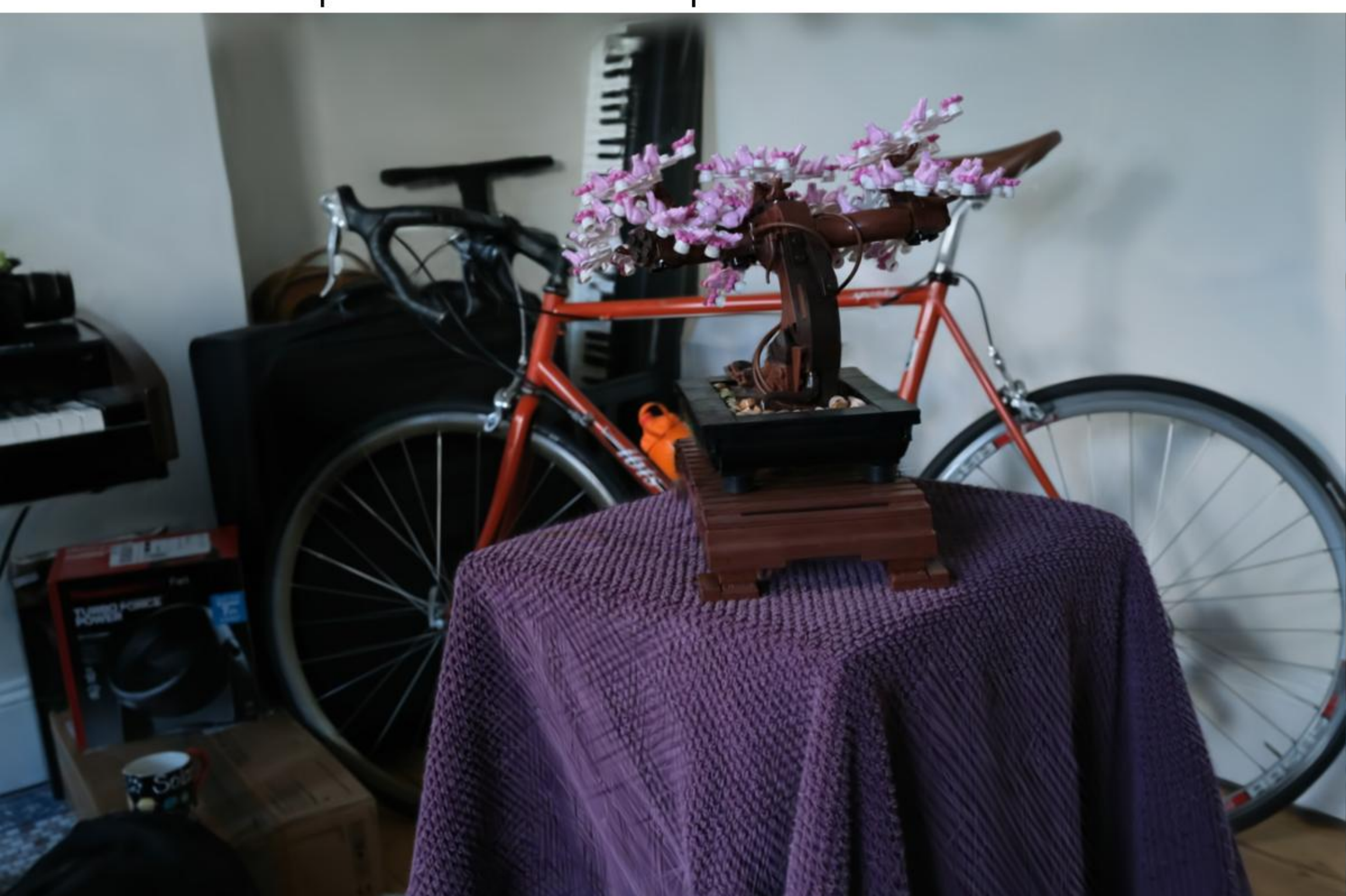
Config: VGGT | Random Init | Pose Opt | Use BA PSNR: 18.99 | LPIPS: 0.2984 | SSIM: 0.6015
