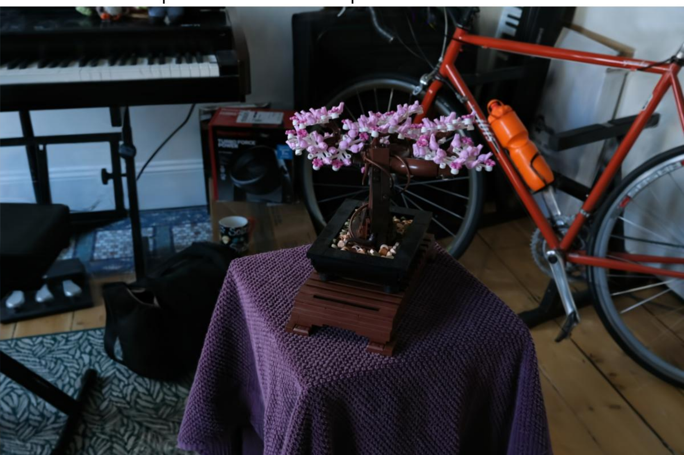
Config: COLMAP | Random Init | Pose Opt | PSNR: 28.02 | LPIPS: 0.0970 | SSIM: 0.8568
