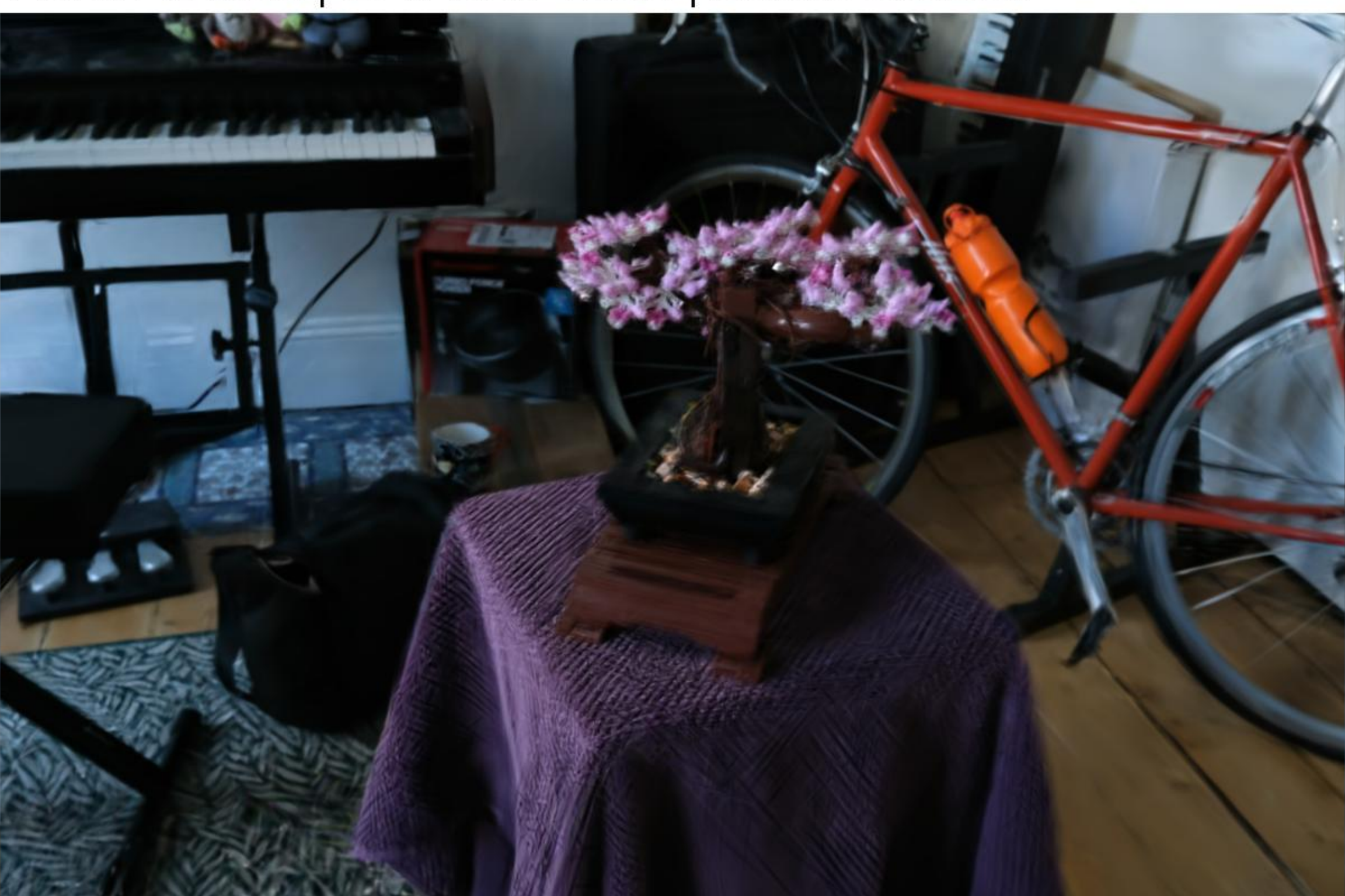
Config: VGGT | Random Init | | PSNR: 16.83 | LPIPS: 0.3947 | SSIM: 0.5379
