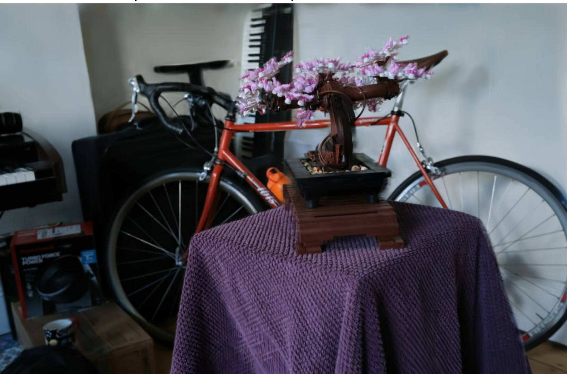
Config: COLMAP | Random Init | | PSNR: 21.20 | LPIPS: 0.1930 | SSIM: 0.6166
