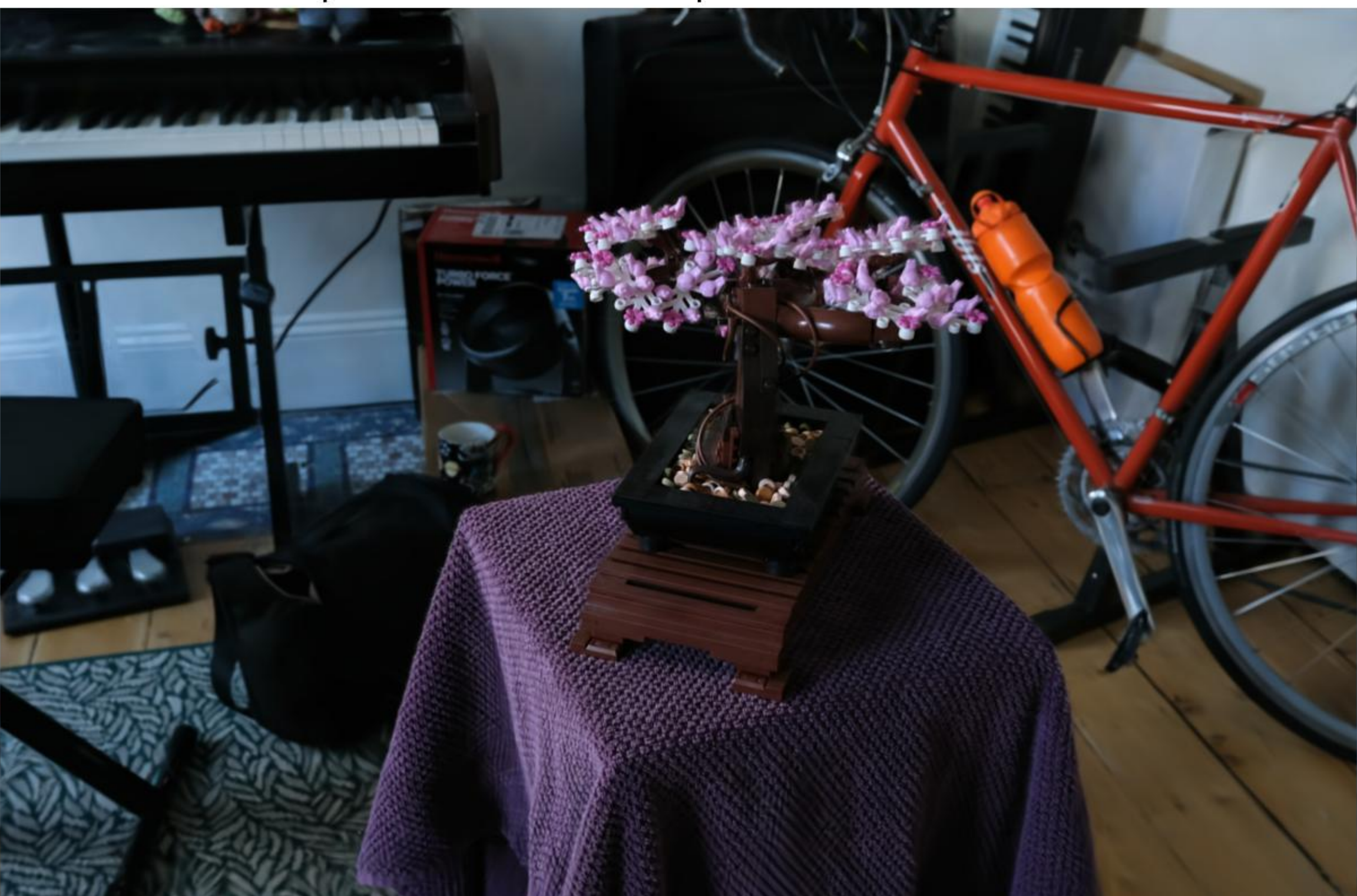
Config: COLMAP | Random Init | | PSNR: 21.83 | LPIPS: 0.1335 | SSIM: 0.6365
