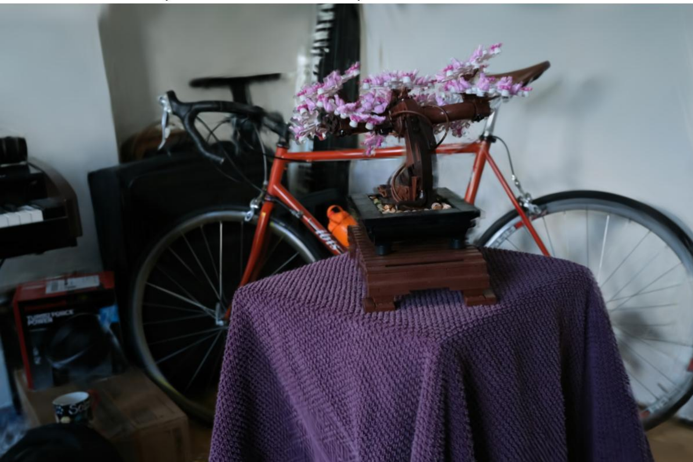
Config: Combined | | VGGTpcd | 100000 PSNR: 20.92 | LPIPS: 0.1908 | SSIM: 0.6088
