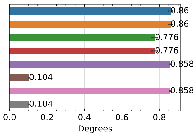
RRE ↓
