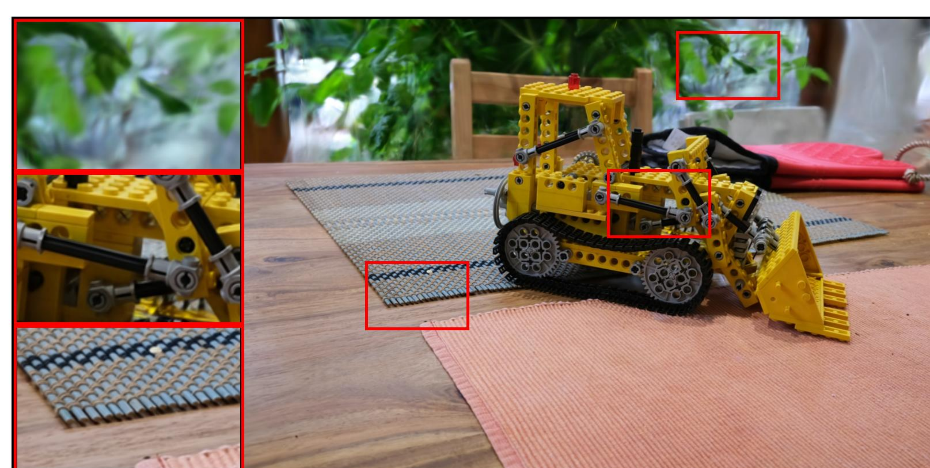
kitchen: VGGT | random | num_points=100000 PSNR: 25.89 | LPIPS: 0.1295 | SSIM: 0.8895
