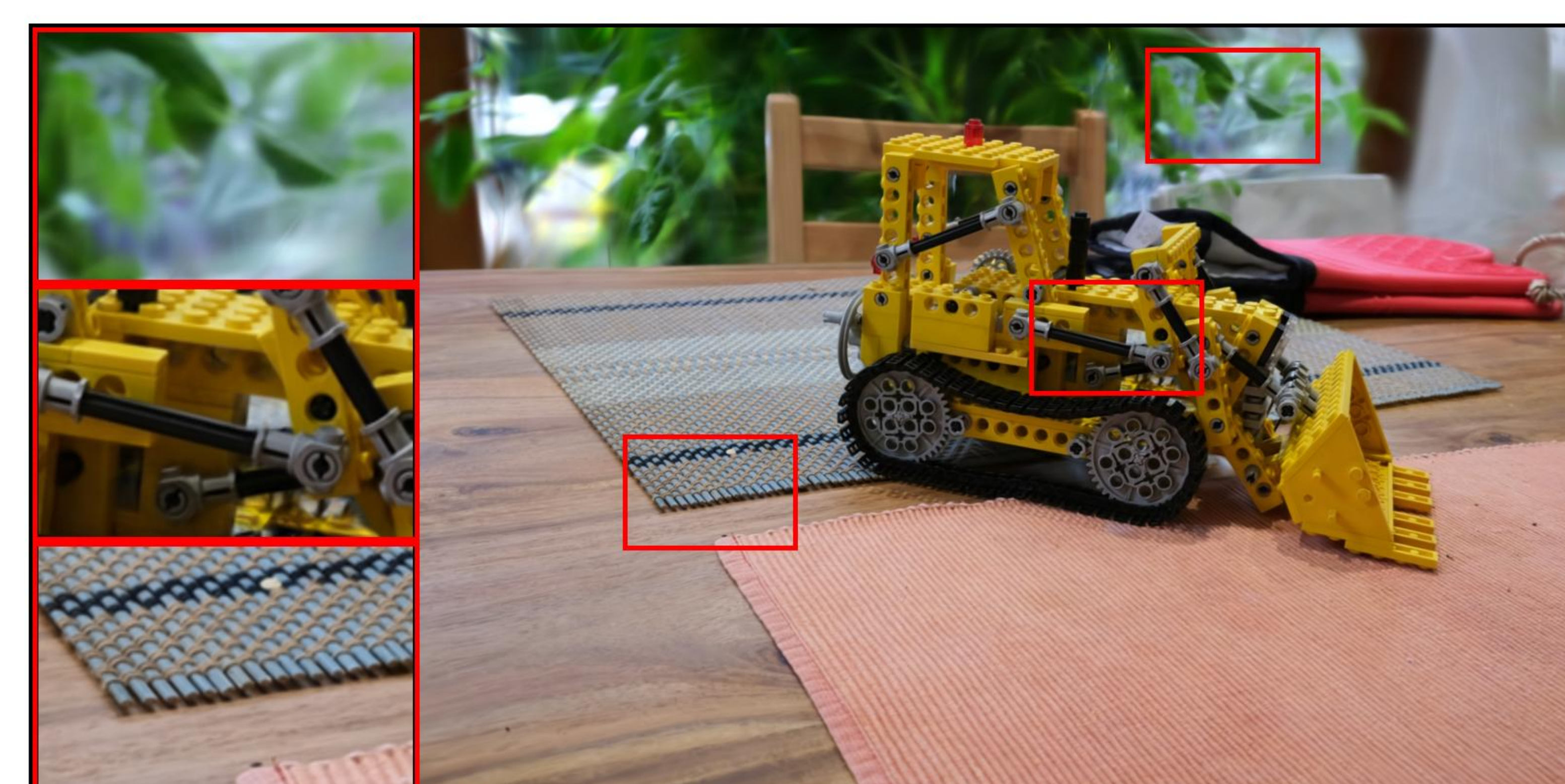
kitchen: VGGT | random | num_points=10000 PSNR: 26.19 | LPIPS: 0.1440 | SSIM: 0.8844
