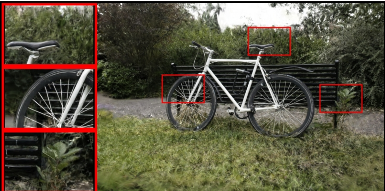
bicycle: VGGT | farthestpose | num_images=40 PSNR: 16.25 | LPIPS: 0.4340 | SSIM: 0.2180
