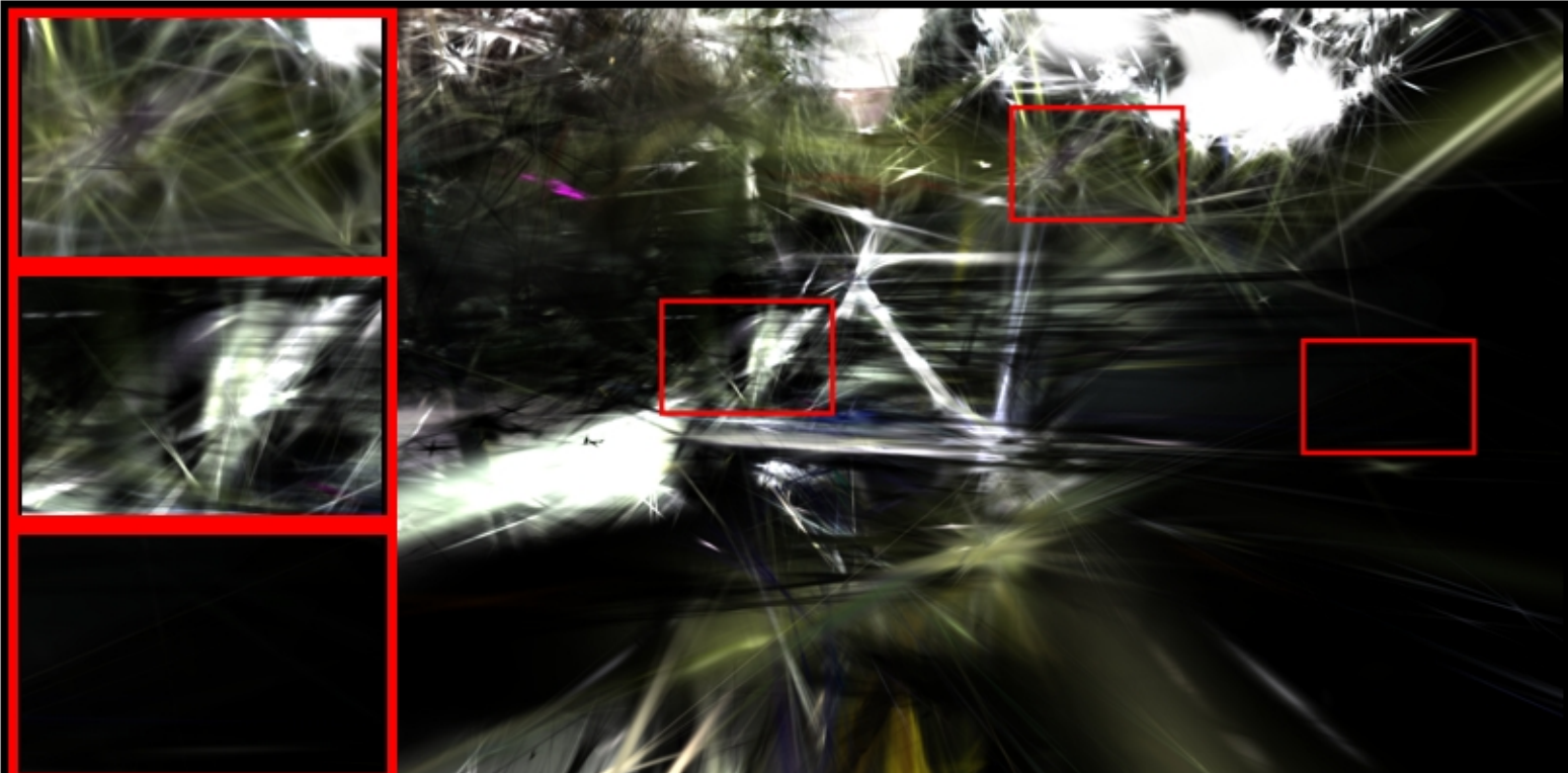
bicycle: COLMAP | farthestpose | num_images=30 PSNR: 10.86 | LPIPS: 0.8103 | SSIM: 0.1551
