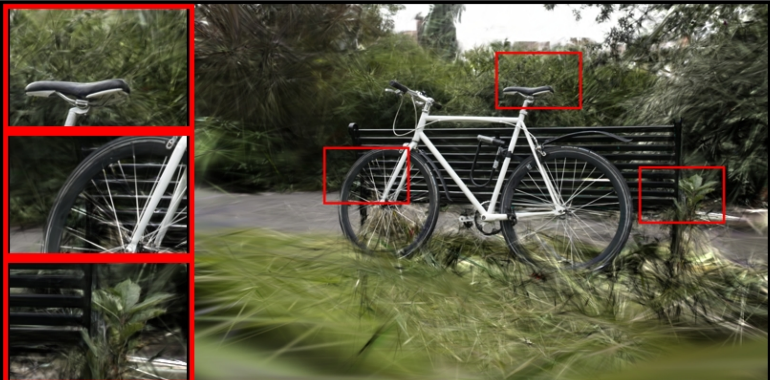
bicycle: COLMAP | farthestpose | num_images=40 PSNR: 13.76 | LPIPS: 0.6845 | SSIM: 0.2436
