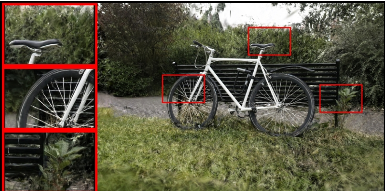
bicycle: VGGT | farthestpose | num_images=30 PSNR: 16.09 | LPIPS: 0.4458 | SSIM: 0.2097
