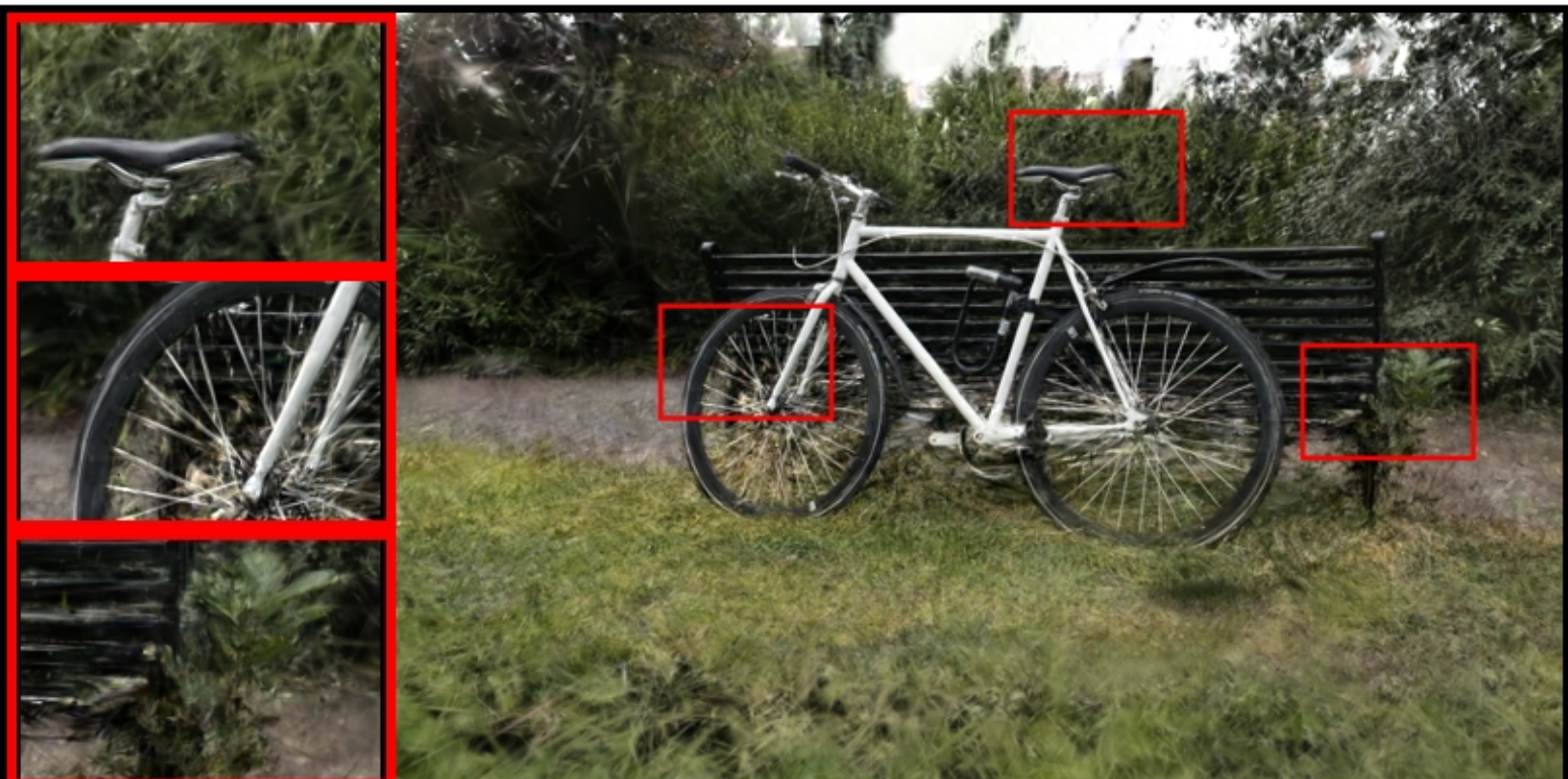
bicycle: VGGT | minfarthestpose | num_images=30 PSNR: 16.63 | LPIPS: 0.3991 | SSIM: 0.2130
