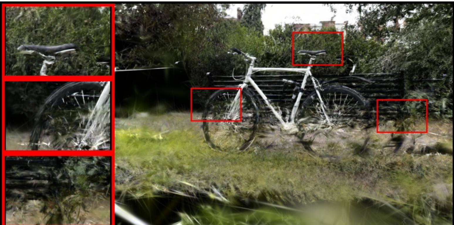
bicycle: VGGT | minfarthestpose | num_images=10 PSNR: 14.90 | LPIPS: 0.5090 | SSIM: 0.1689
