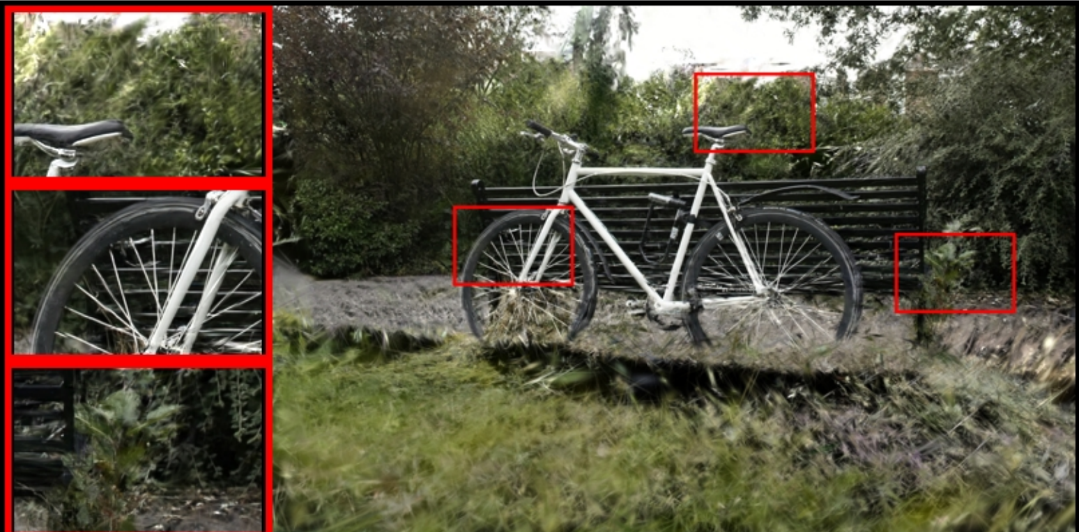
bicycle: VGGT | farthestpose | num_images=10 PSNR: 13.89 | LPIPS: 0.5661 | SSIM: 0.1504
