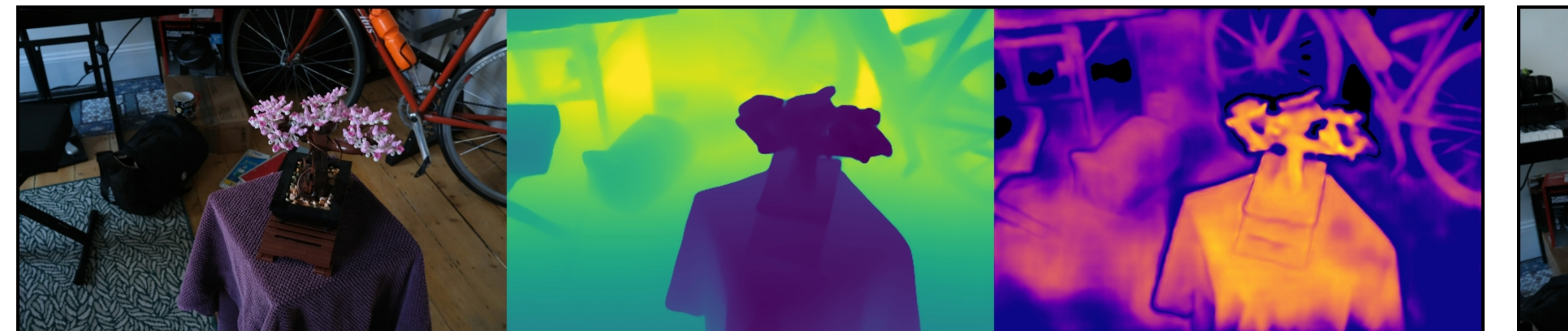
bonsai: VGGT | minfarthestpose | num_images=10 Original | Depth (max=1.78) | Confidence (max=4.15)
