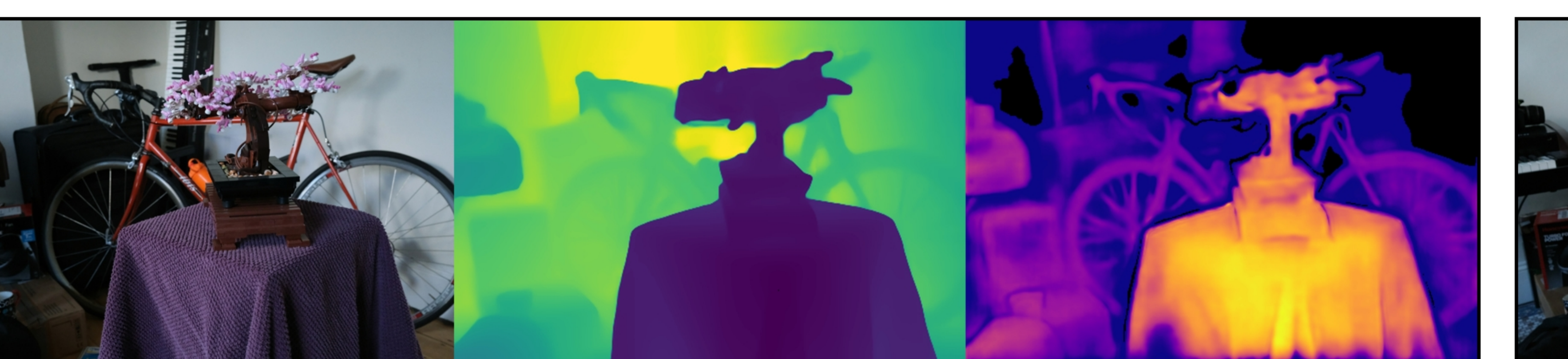
bonsai: VGGT | farthestpose | num_images=30 Original | Depth (max=2.22) | Confidence (max=4.19)
