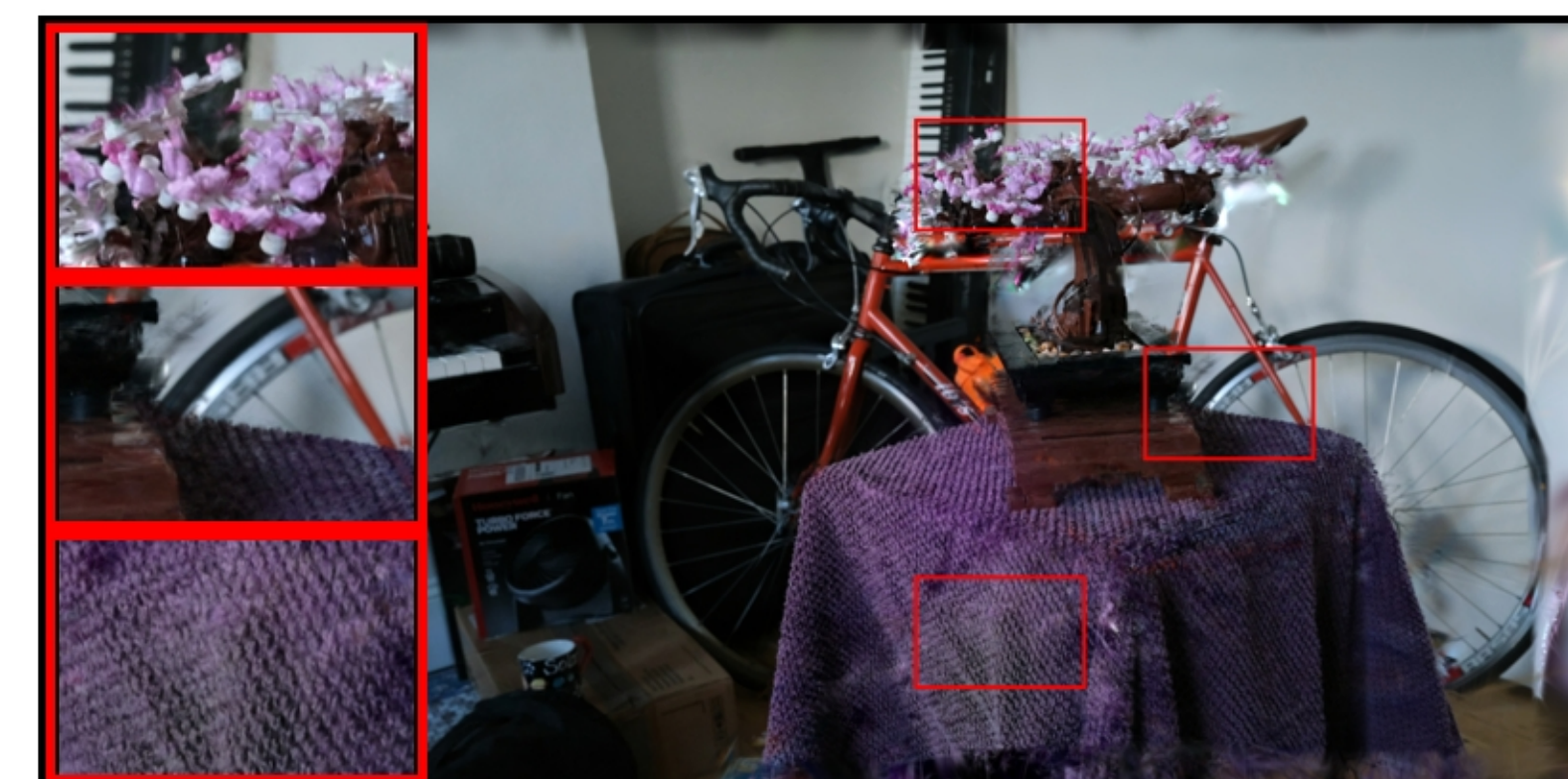
bonsai: VGGT | farthestpose | num_images=10 PSNR: 14.49 | LPIPS: 0.5611 | SSIM: 0.4374
