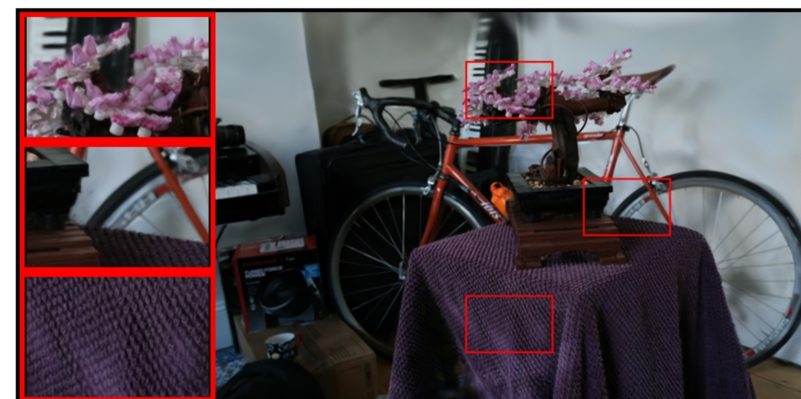
bonsai: VGGT | minfarthestpose | num_images=100 PSNR: 18.46 | LPIPS: 0.3355 | SSIM: 0.5824
