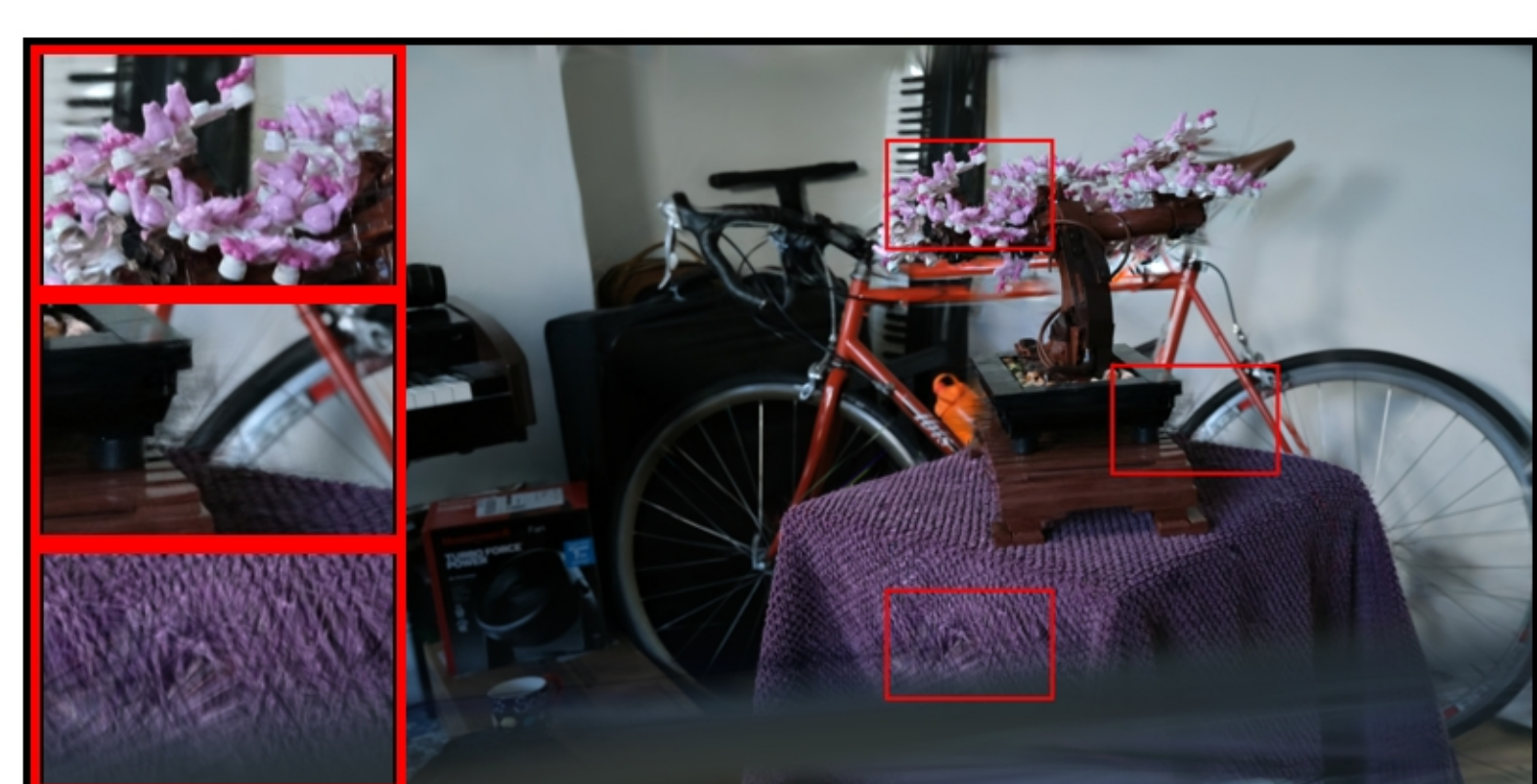
bonsai: COLMAP | farthestpose | num_images=20 PSNR: 13.06 | LPIPS: 0.5597 | SSIM: 0.4090
