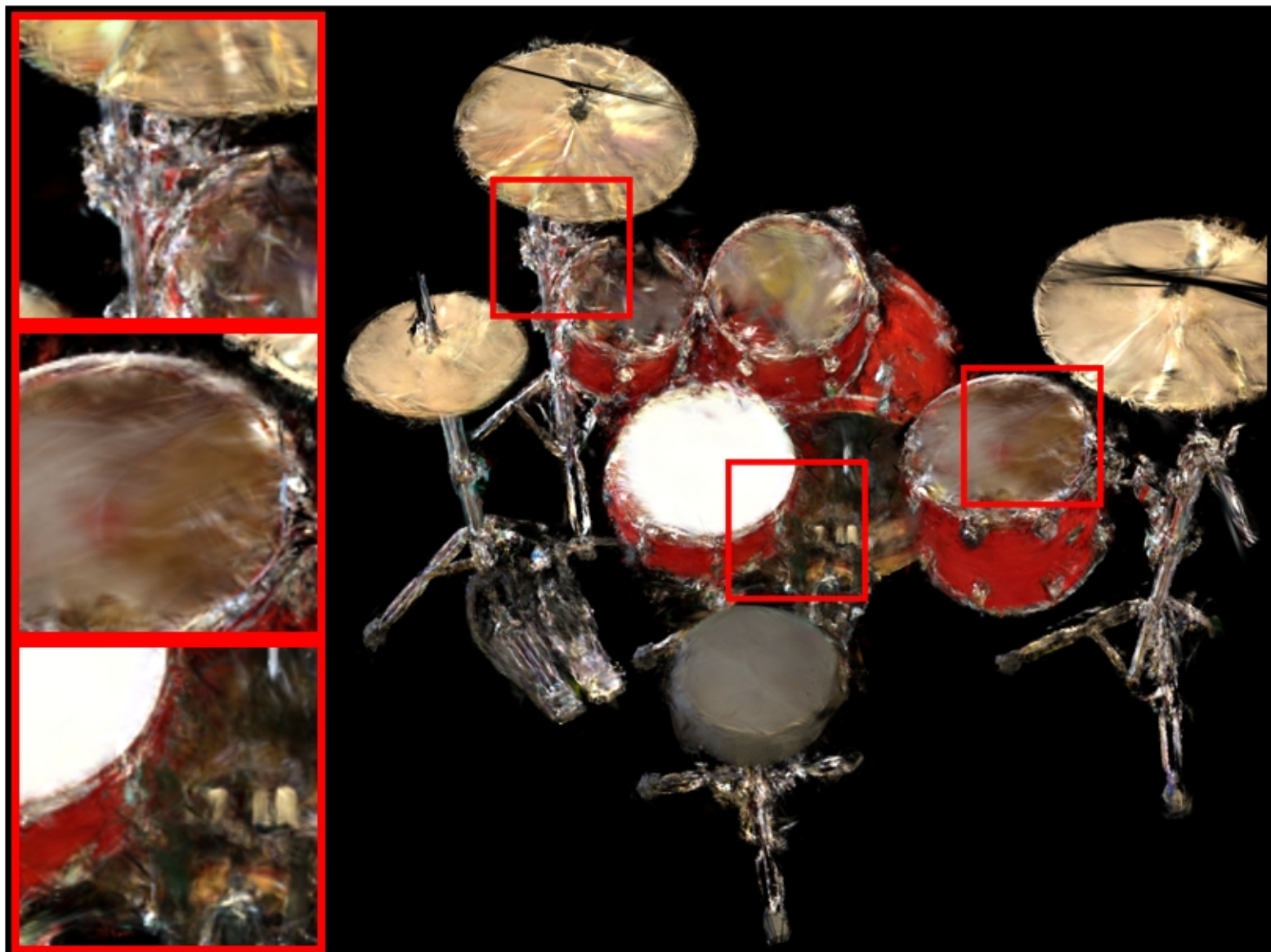
drums: VGGT | farthestpose | num_images=20 PSNR: 13.02 | LPIPS: 0.3515 | SSIM: 0.6519
