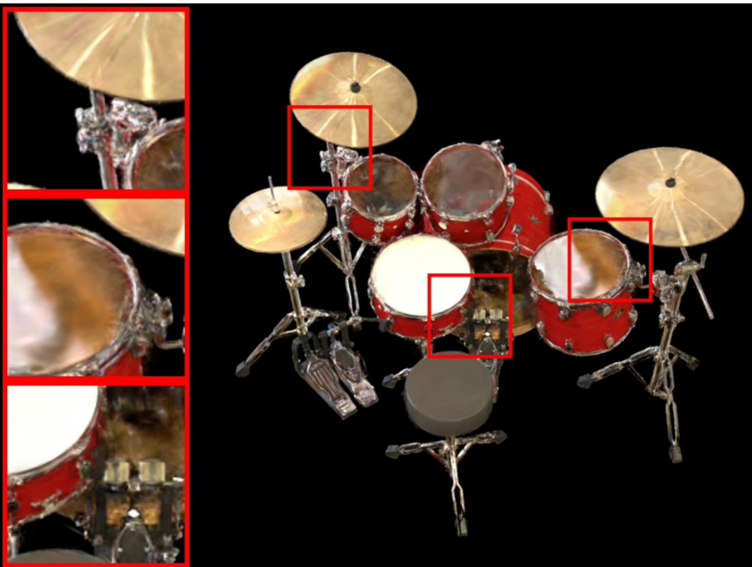
drums: VGGT | farthestpose | num_images=40 PSNR: 17.64 | LPIPS: 0.1120 | SSIM: 0.7948
