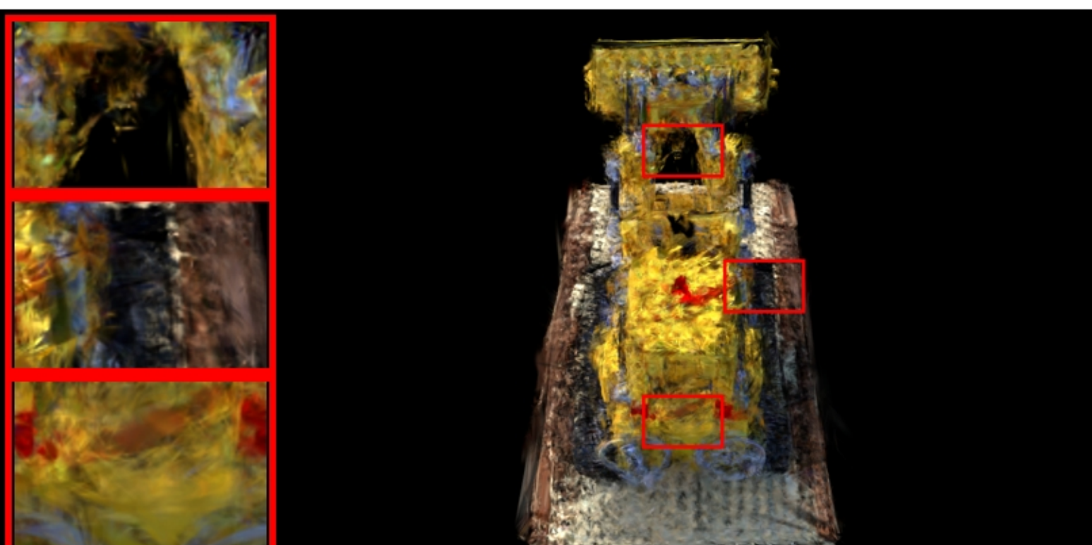
lego: VGGT | farthestpose | num_images=30 PSNR: 13.85 | LPIPS: 0.3084 | SSIM: 0.6320
