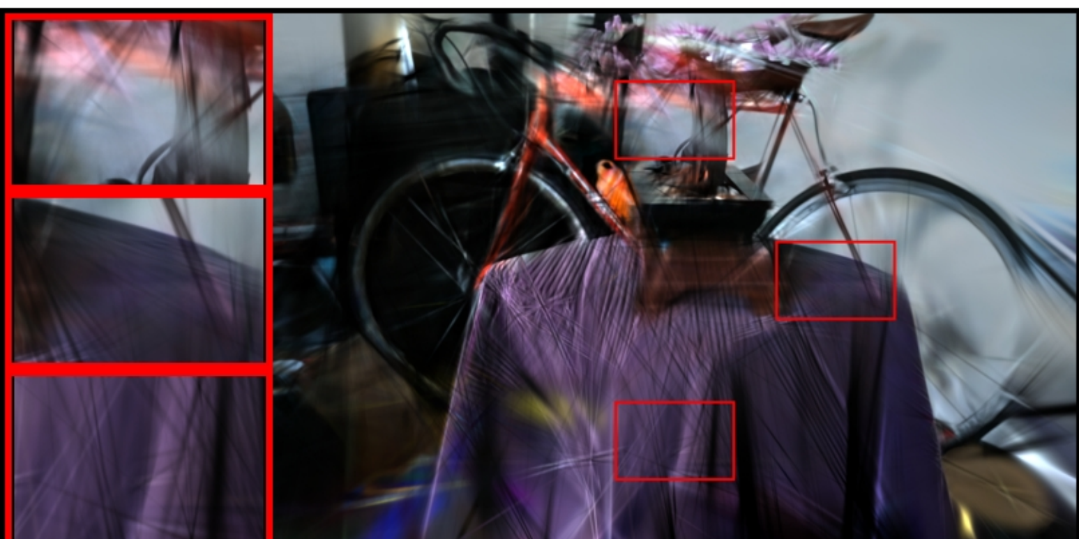
bonsai: COLMAP | farthestpose | num_images=10 PSNR: 10.37 | LPIPS: 0.8213 | SSIM: 0.3029
