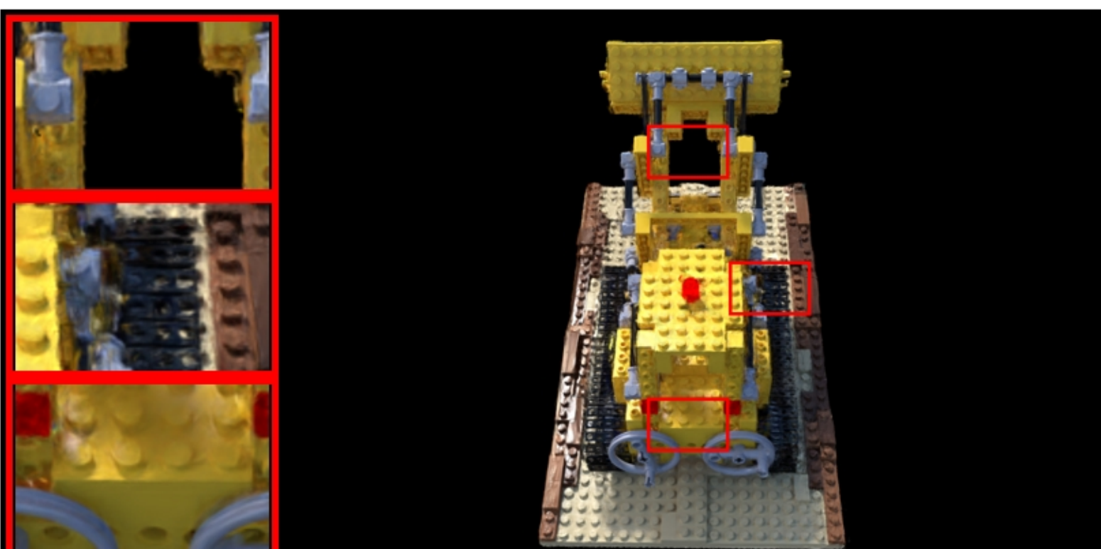
lego: VGGT | farthestpose | num_images=40 PSNR: 14.32 | LPIPS: 0.2649 | SSIM: 0.6631
