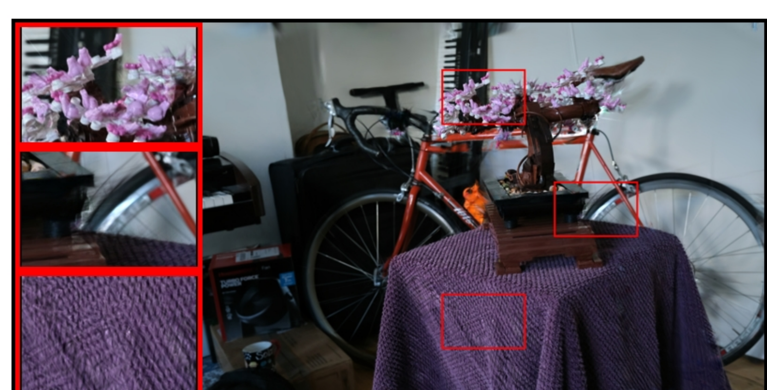
bonsai: COLMAP | farthestpose | num_images=20 PSNR: 12.16 | LPIPS: 0.5964 | SSIM: 0.3499
