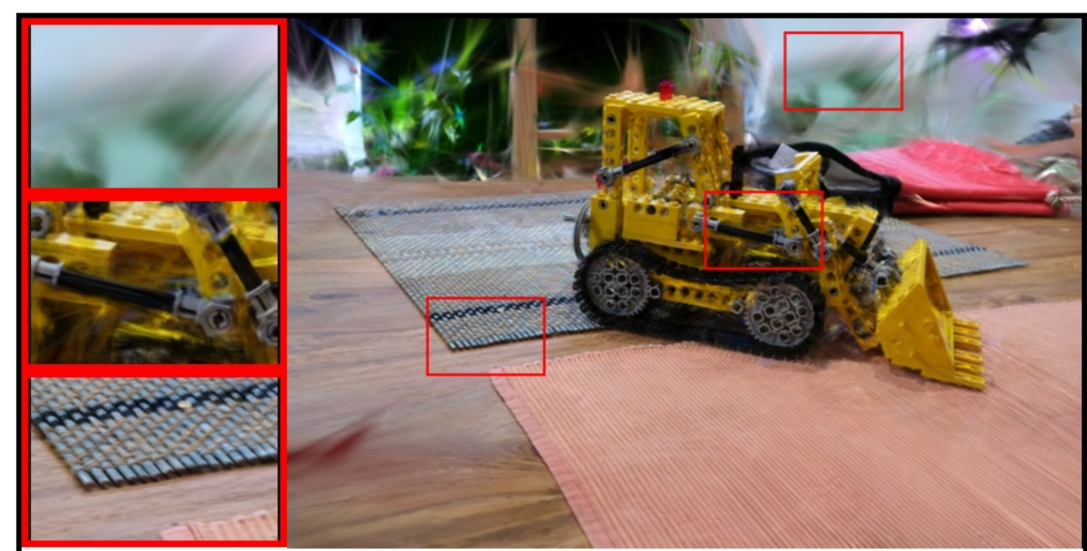
kitchen: COLMAP | farthestpose | num_images=20 PSNR: 17.51 | LPIPS: 0.4069 | SSIM: 0.5586
