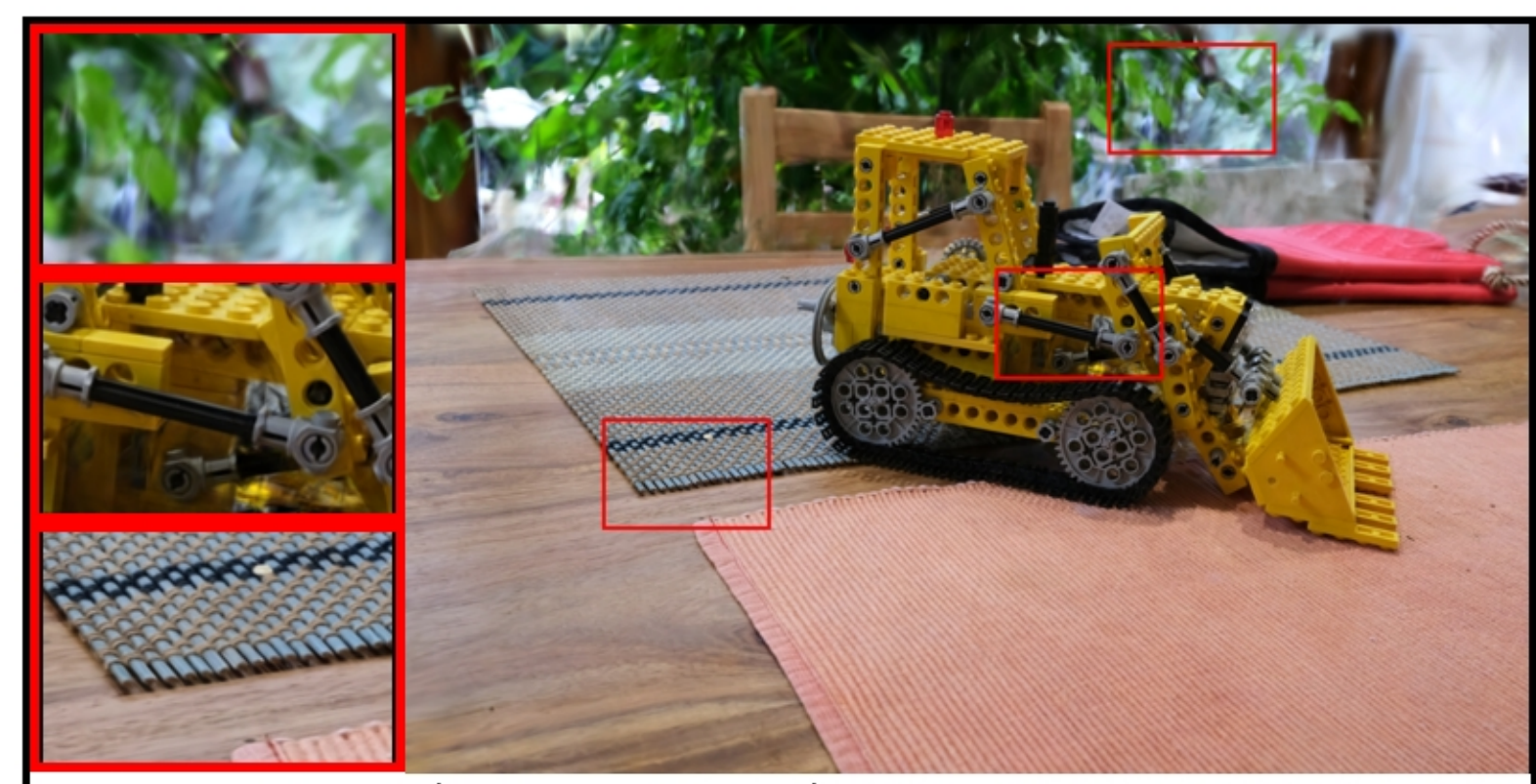
kitchen: VGGT | farthestpose | num_images=40 PSNR: 18.97 | LPIPS: 0.2114 | SSIM: 0.4483
