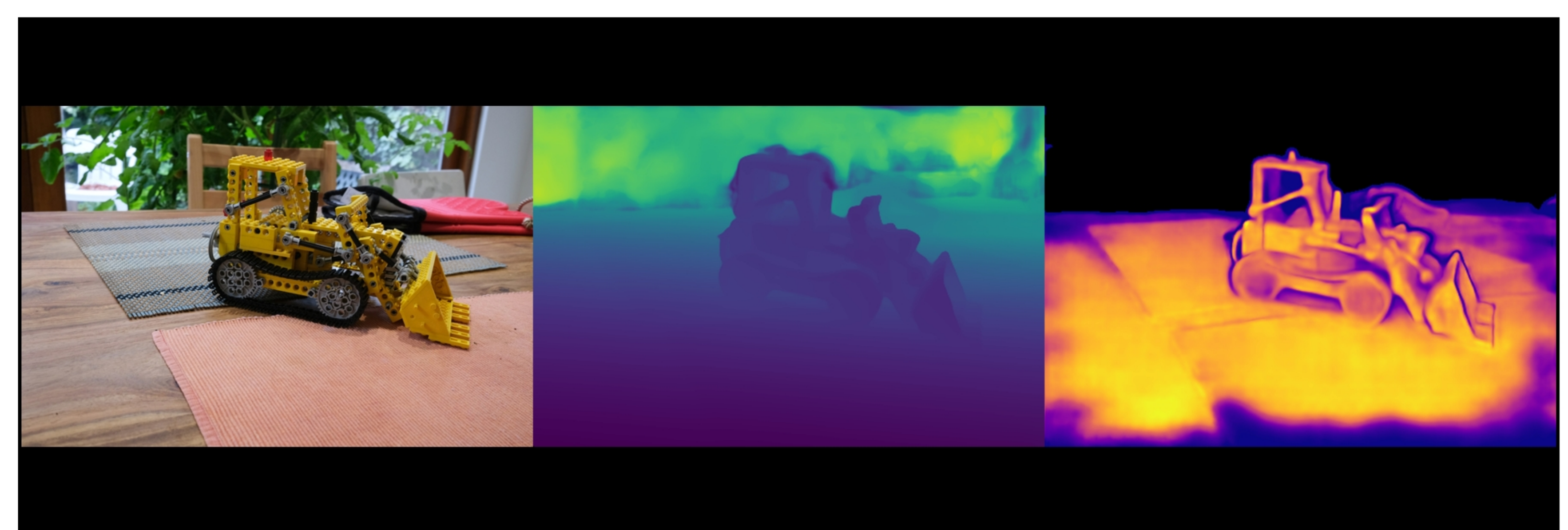
kitchen: VGGT | minfarthestpose | num_images=20 Original | Depth (max=2.47) | Confidence (max=27.37)
