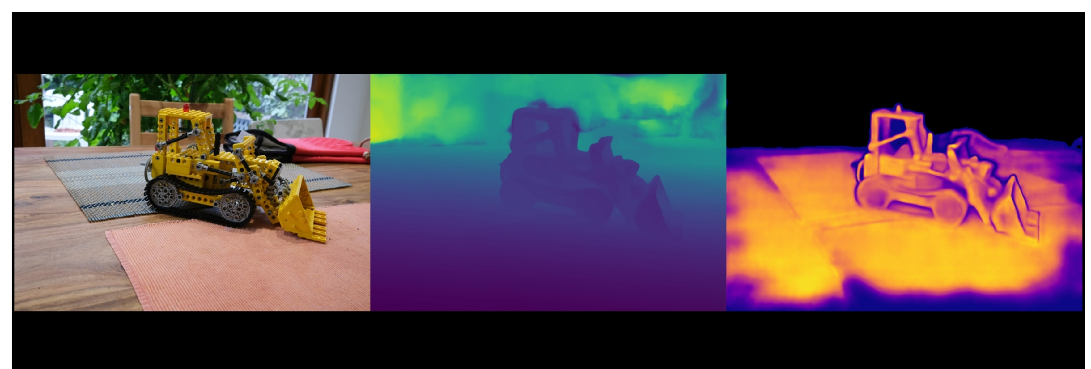
kitchen: VGGT | minfarthestpose | num_images=10 Original | Depth (max=2.54) | Confidence (max=26.08)
