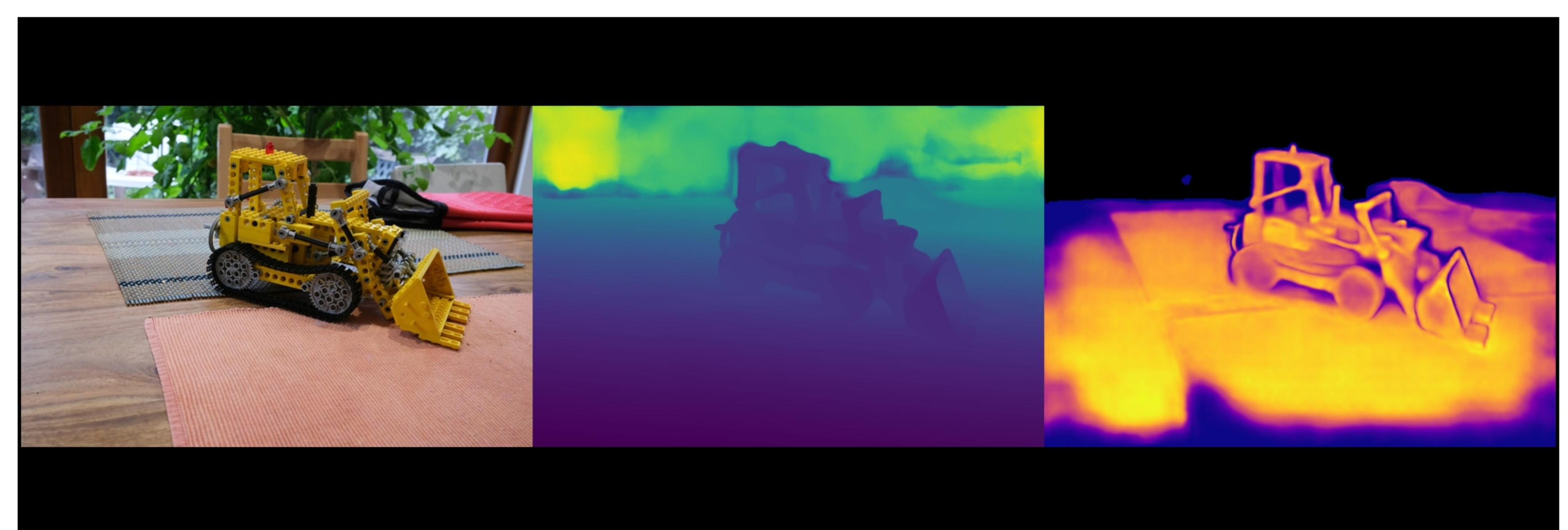
kitchen: VGGT | farthestpose | num_images=30 Original | Depth (max=2.51) | Confidence (max=24.44)
