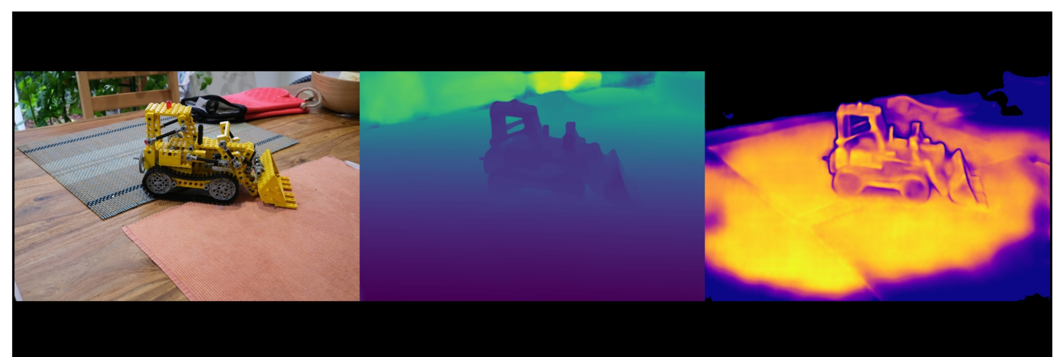
kitchen: VGGT | farthestpose | num_images=20 Original | Depth (max=2.24) | Confidence (max=23.39)
