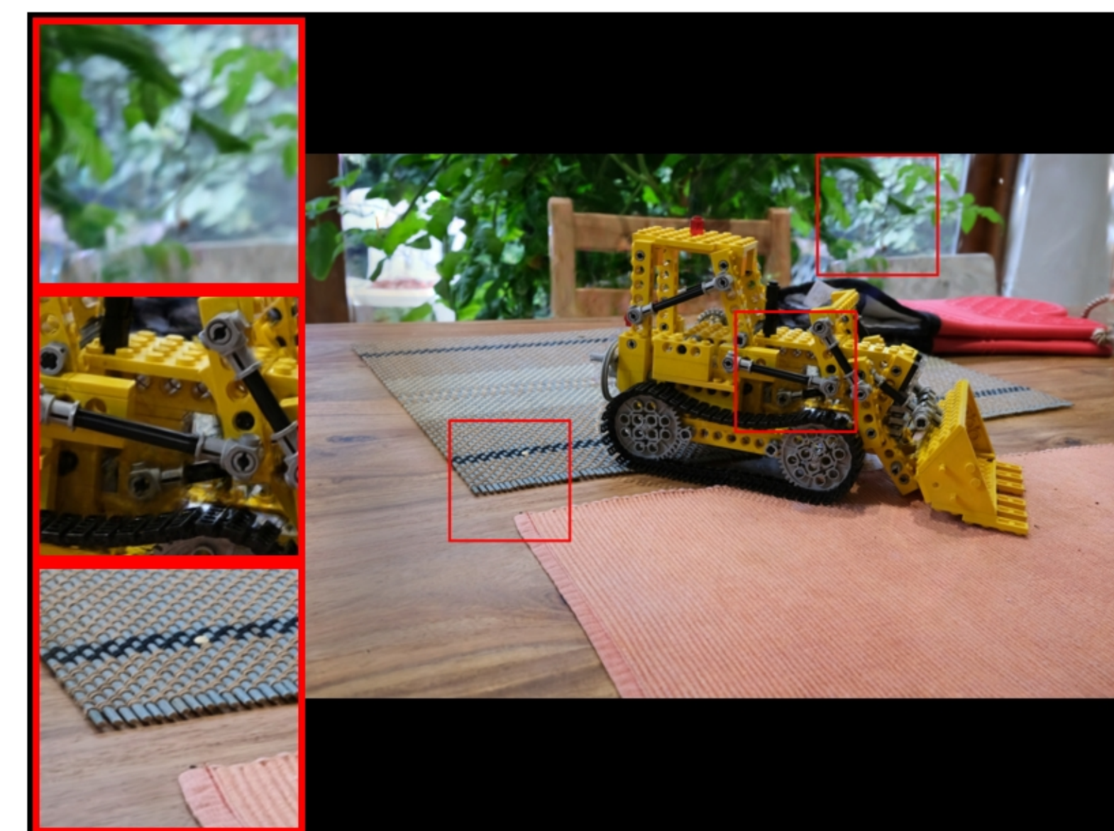
kitchen: VGGT | minfarthestpose | num_images=20 PSNR: 18.30 | LPIPS: 0.2524 | SSIM: 0.4351
