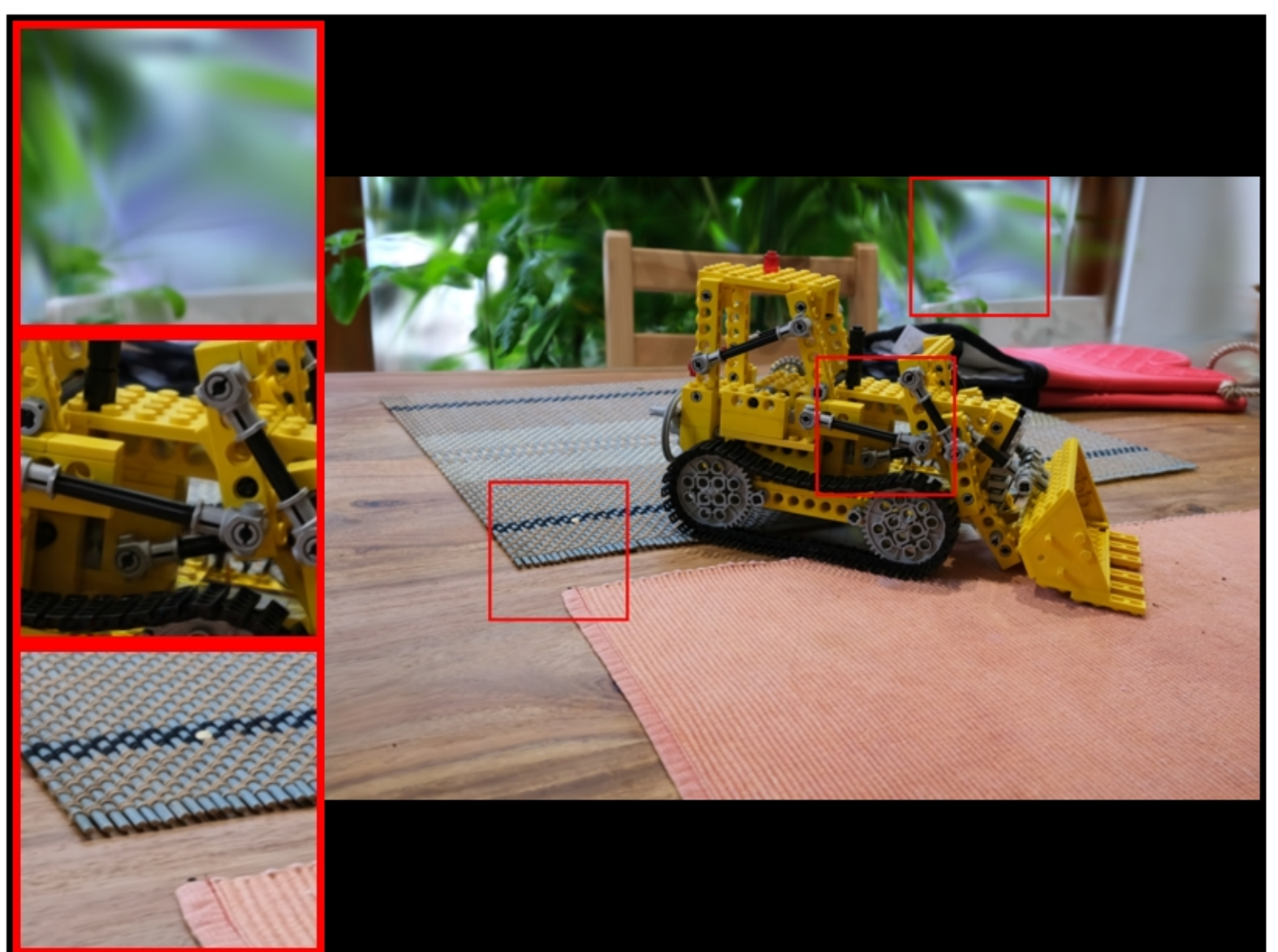
kitchen: COLMAP | minfarthestpose | num_images=100 PSNR: 22.44 | LPIPS: 0.1272 | SSIM: 0.5514
