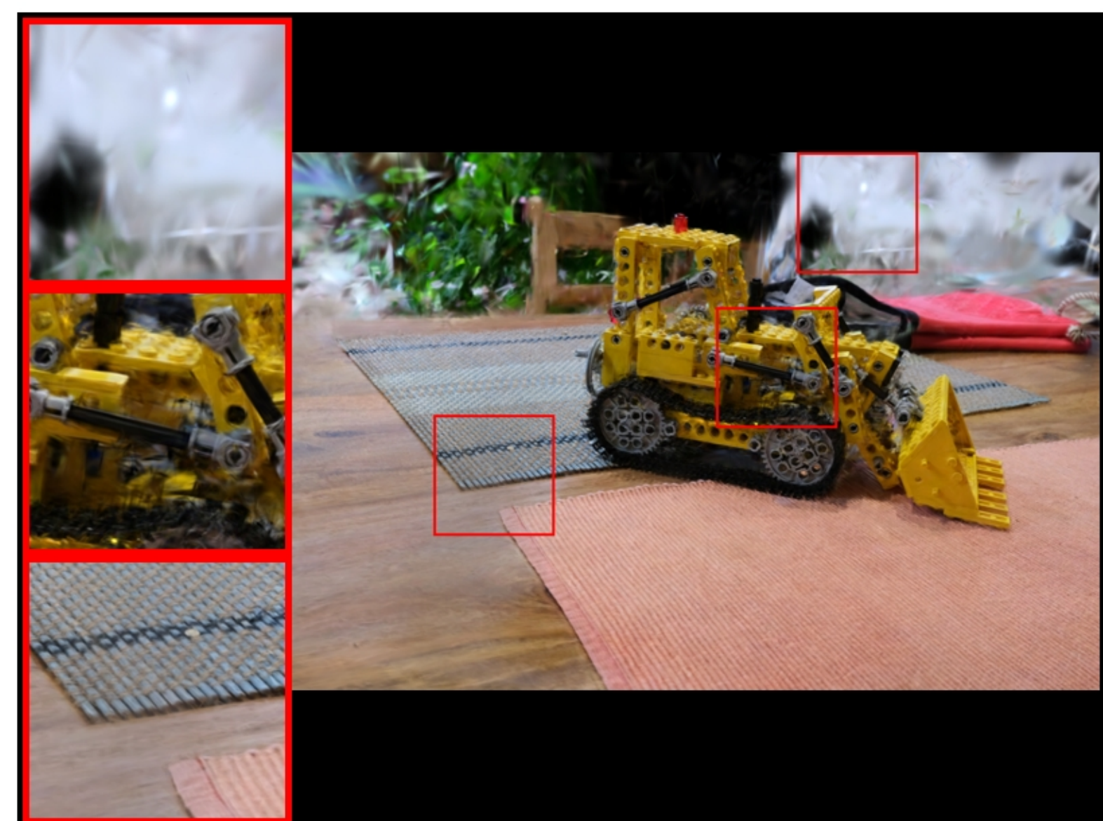
kitchen: VGGT | farthestpose | num_images=20 PSNR: 17.51 | LPIPS: 0.2900 | SSIM: 0.4111
