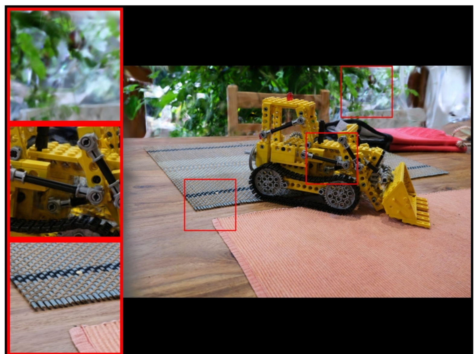
kitchen: VGGT | farthestpose | num_images=30 PSNR: 19.27 | LPIPS: 0.2263 | SSIM: 0.4959
