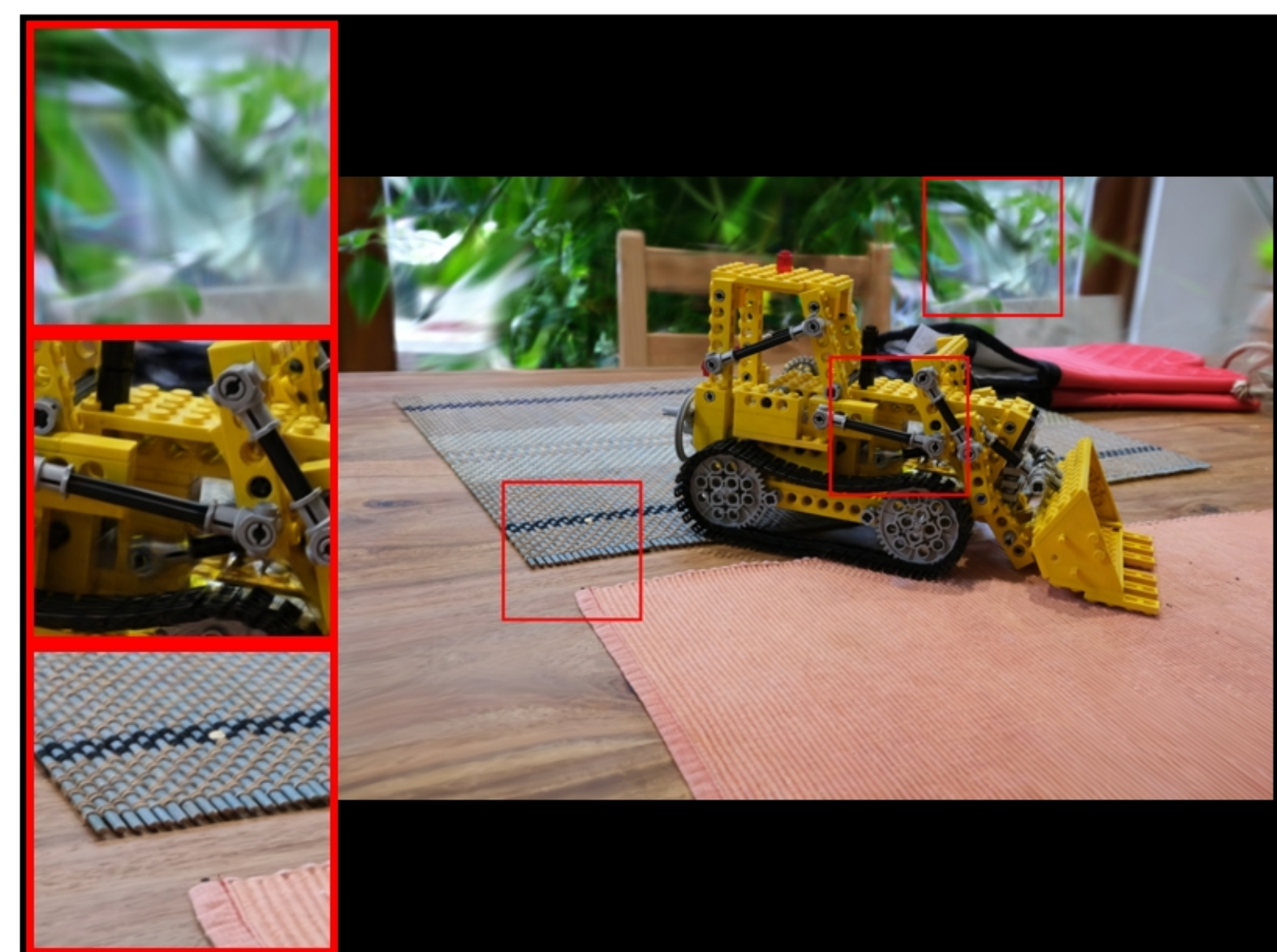
kitchen: COLMAP | minfarthestpose | num_images=30 PSNR: 20.69 | LPIPS: 0.2098 | SSIM: 0.5228
