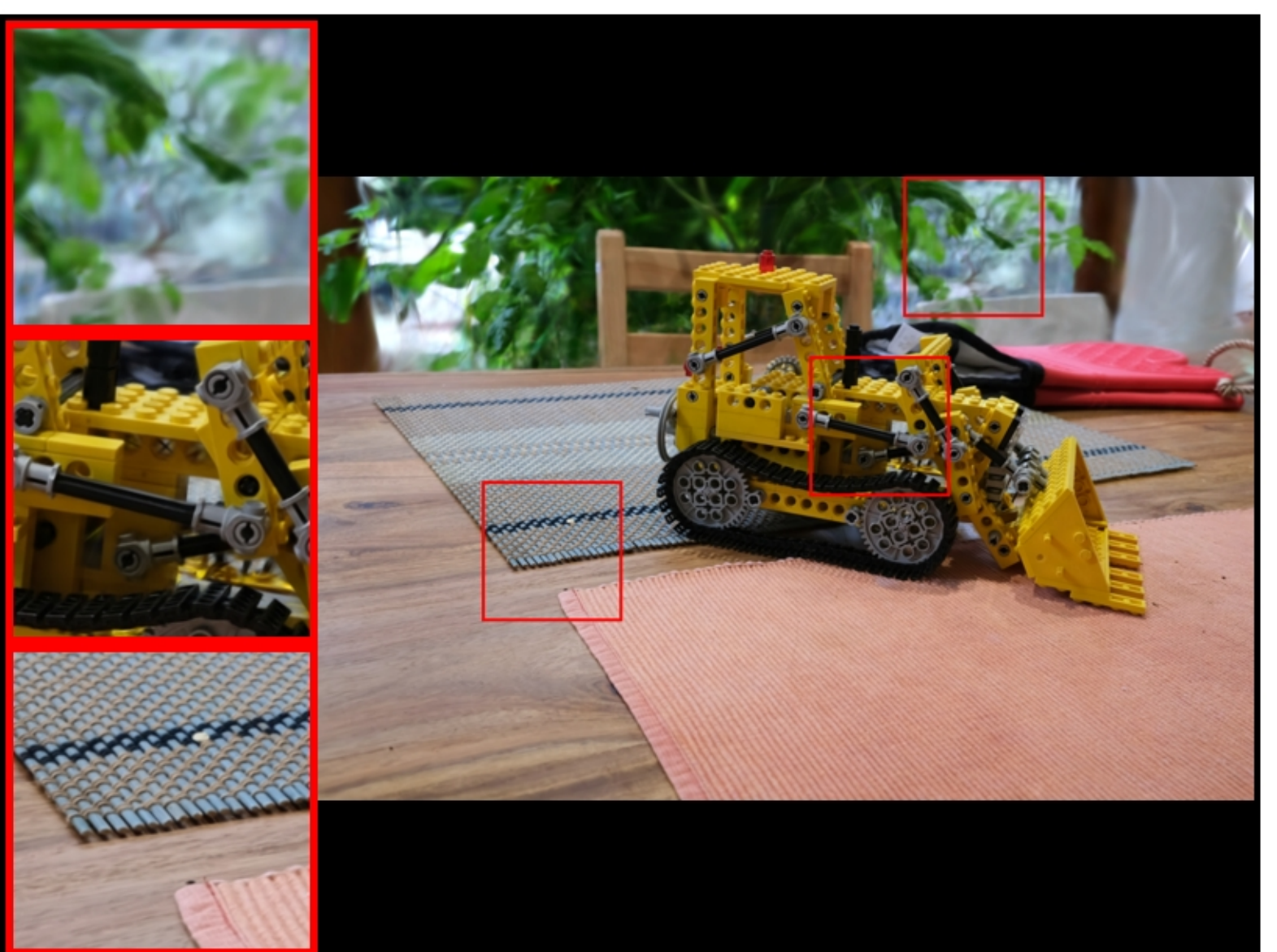
kitchen: VGGT | farthestpose | num_images=100 PSNR: 20.02 | LPIPS: 0.1764 | SSIM: 0.4138
