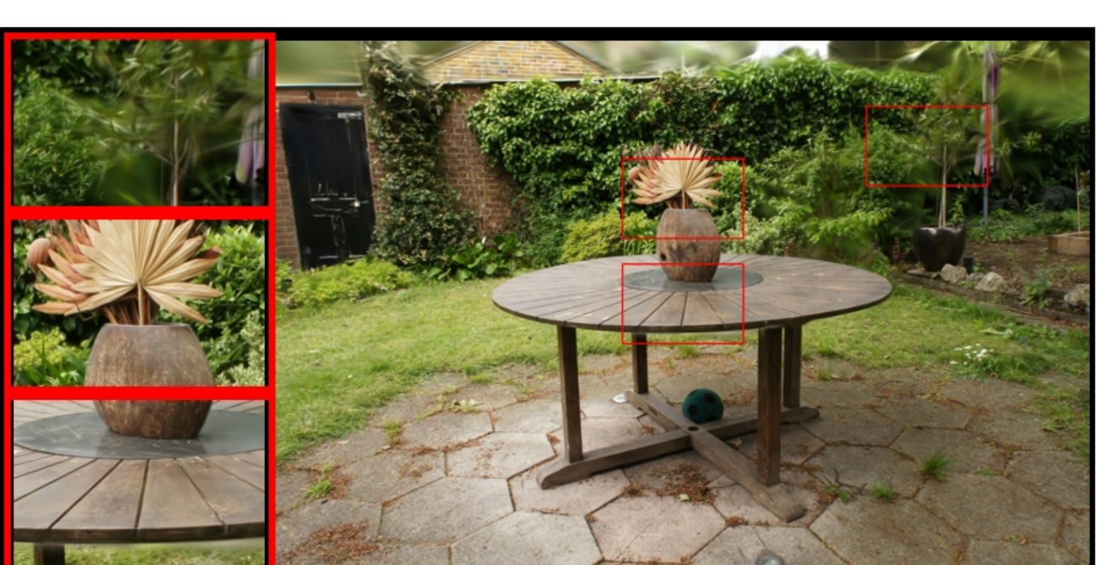
garden: COLMAP | farthestpose | num_images=100 PSNR: 22.13 | LPIPS: 0.2637 | SSIM: 0.5121
