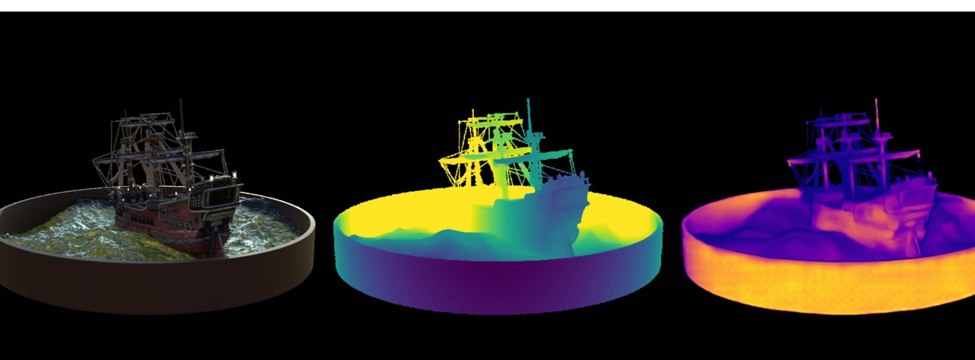
ship: VGGT | farthestpose | num_images=40 Original | Depth (max=1.30) | Confidence (max=167.46)
