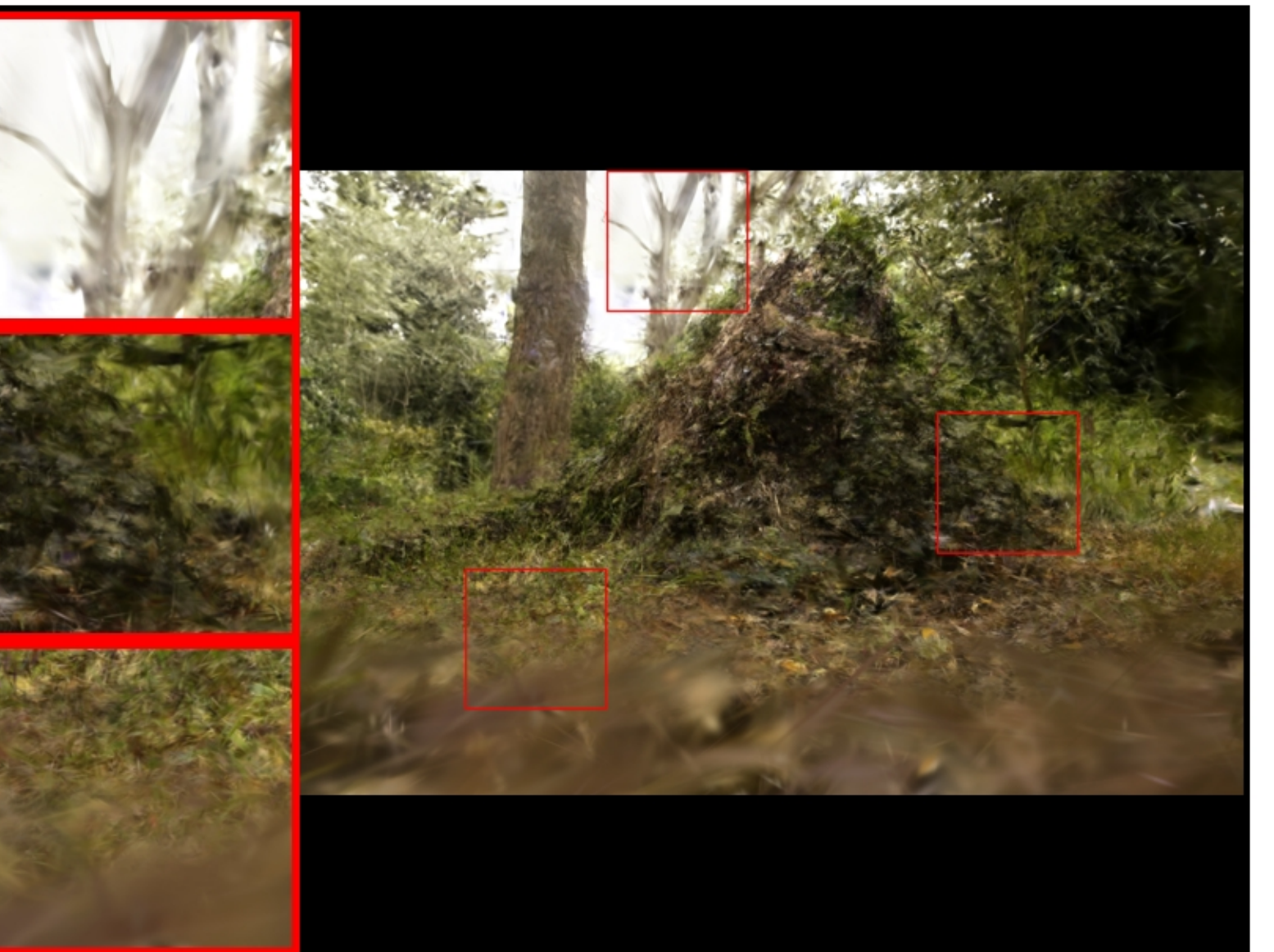
stump: VGGT | farthestpose | num_images=20 PSNR: 15.88 | LPIPS: 0.5566 | SSIM: 0.2900
