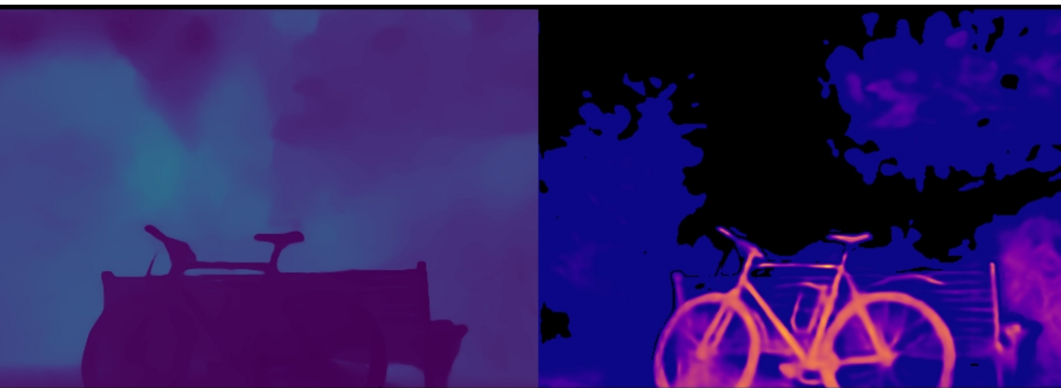
bicycle: VGGT | Pose Opt | num_images=100 Original | Depth (max=2.56) | Confidence (max=2.99)
