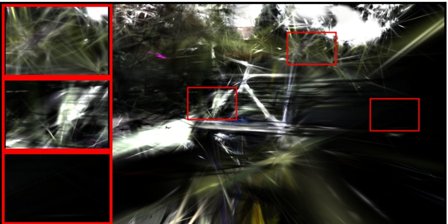
bicycle: COLMAP | Pose Opt | num_images=30 PSNR: 10.86 | LPIPS: 0.8103 | SSIM: 0.1551
