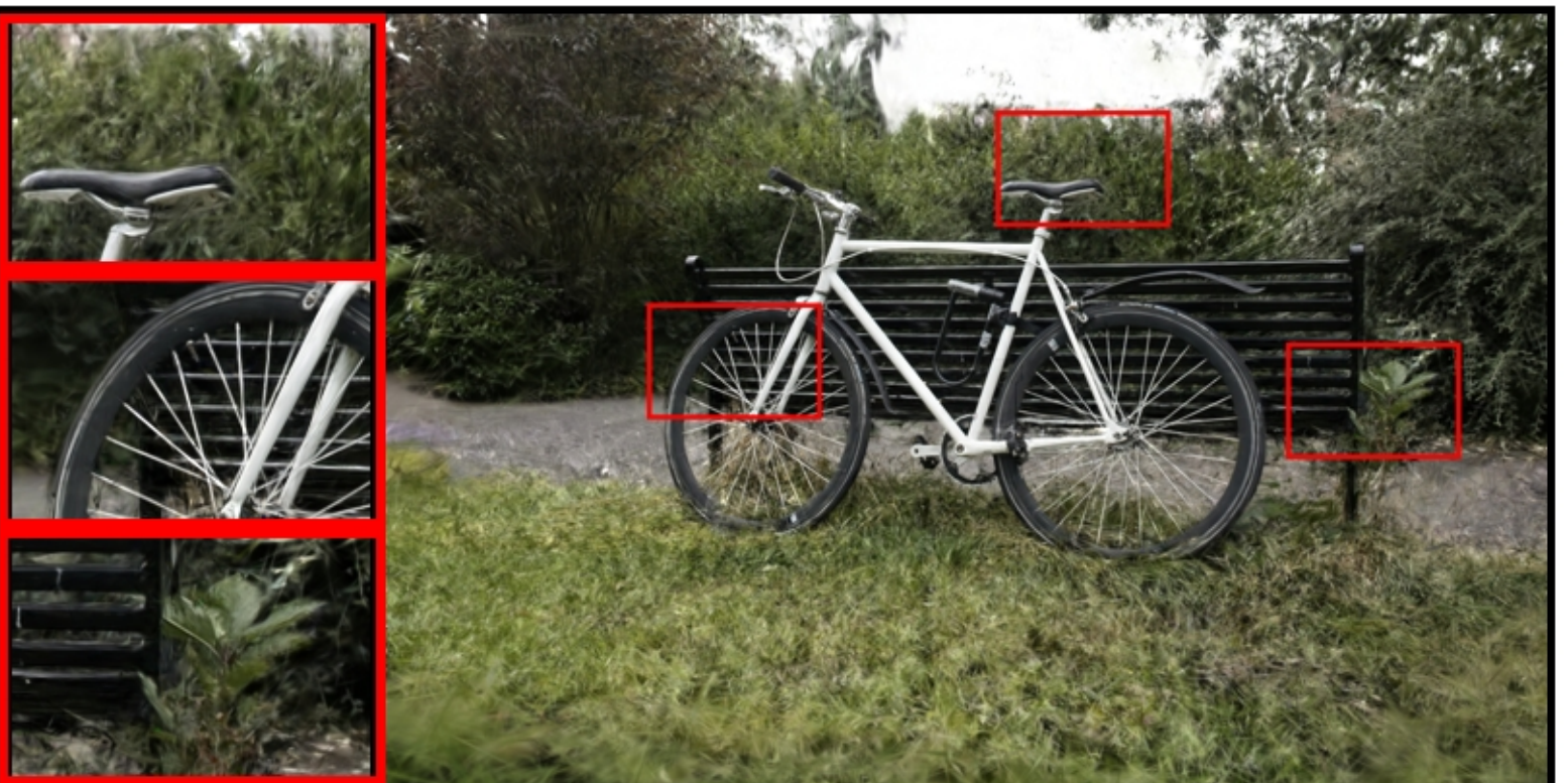
bicycle: VGGT | Pose Opt | num_images=40 PSNR: 16.25 | LPIPS: 0.4340 | SSIM: 0.2180
