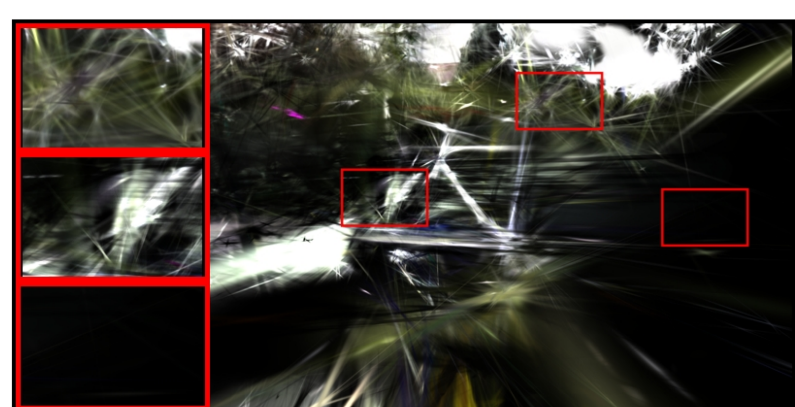
bicycle: COLMAP | Pose Opt | num_images=30 PSNR: 10.86 | LPIPS: 0.8103 | SSIM: 0.1551
