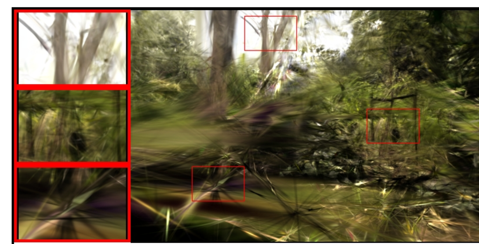
stump: COLMAP | Pose Opt | num_images=20 PSNR: 12.79 | LPIPS: 0.9256 | SSIM: 0.1493
