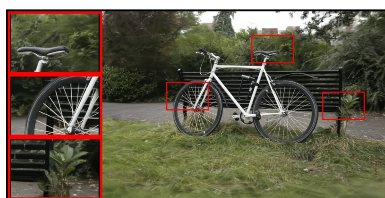
bicycle: COLMAP | Pose Opt | num_images=100 PSNR: 22.16 | LPIPS: 0.3495 | SSIM: 0.5587
