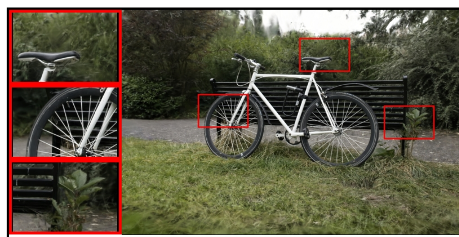
bicycle: VGGT | Pose Opt | num_images=100 PSNR: 17.38 | LPIPS: 0.3378 | SSIM: 0.2679
