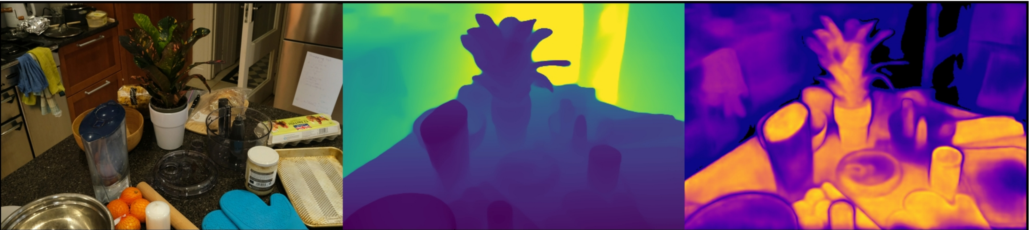
counter: VGGT | | 0.0 | Original | Depth (max=2.88) | Confidence (max=15.71)
