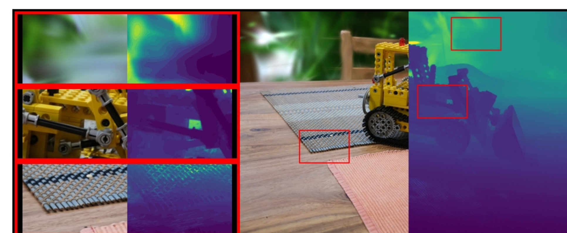
kitchen: VGGT | | 0.0 | PSNR: 20.04 | LPIPS: 0.1993 | SSIM: 0.4245
