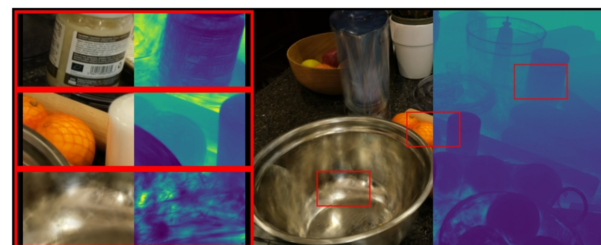
counter: VGGT | closer | 0.1 | Standard Shifted PSNR: 20.51 | LPIPS: 0.2588 | SSIM: 0.6339
