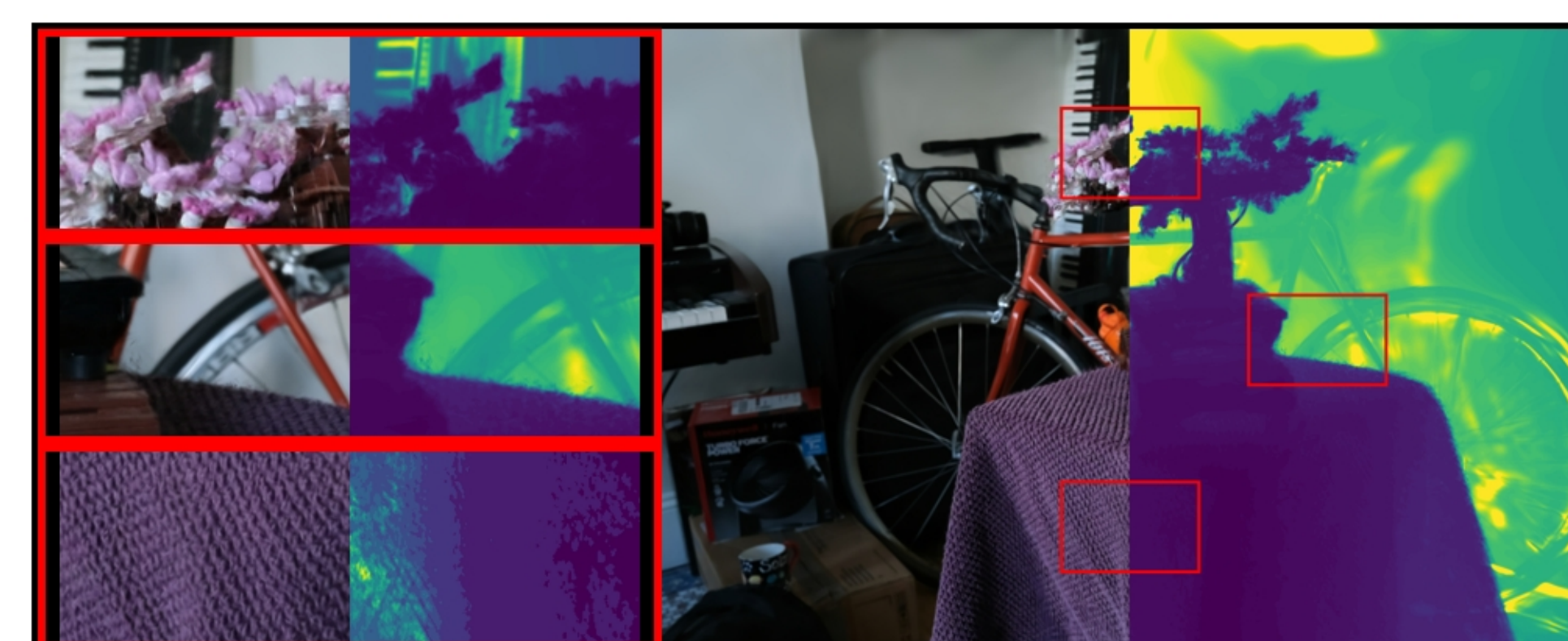
bonsai: VGGT | closer | 0.1 | Standard Shifted PSNR: 17.41 | LPIPS: 0.4003 | SSIM: 0.5601
