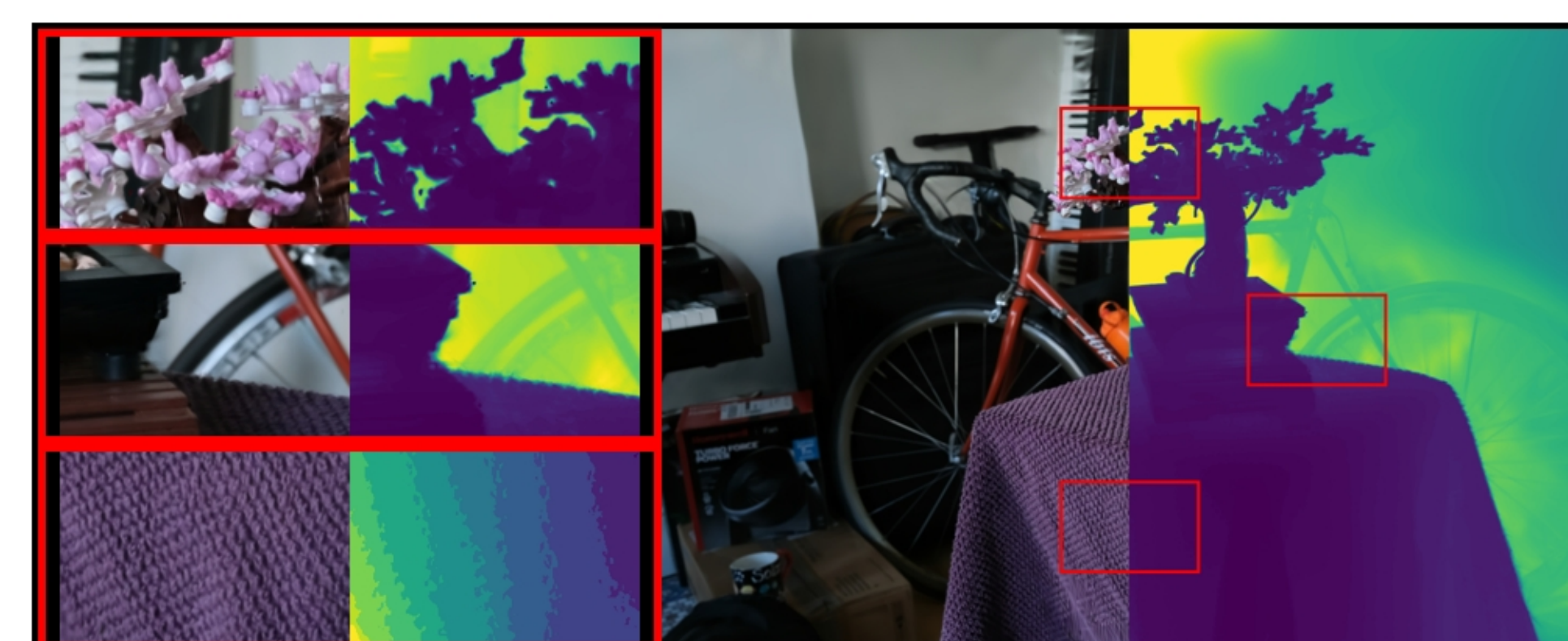
bonsai: COLMAP | points | 0.1 | PSNR: 26.85 | LPIPS: 0.1693 | SSIM: 0.8499
