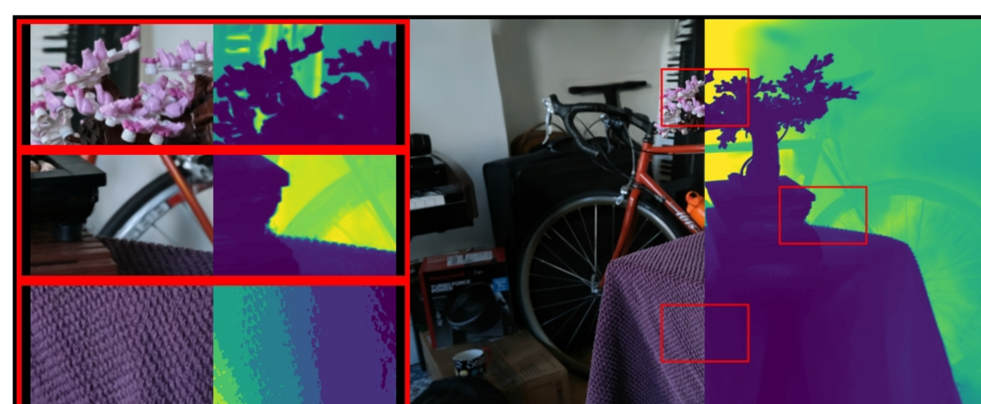
bonsai: Combined | | 0.0 | PSNR: 25.20 | LPIPS: 0.1691 | SSIM: 0.7971
