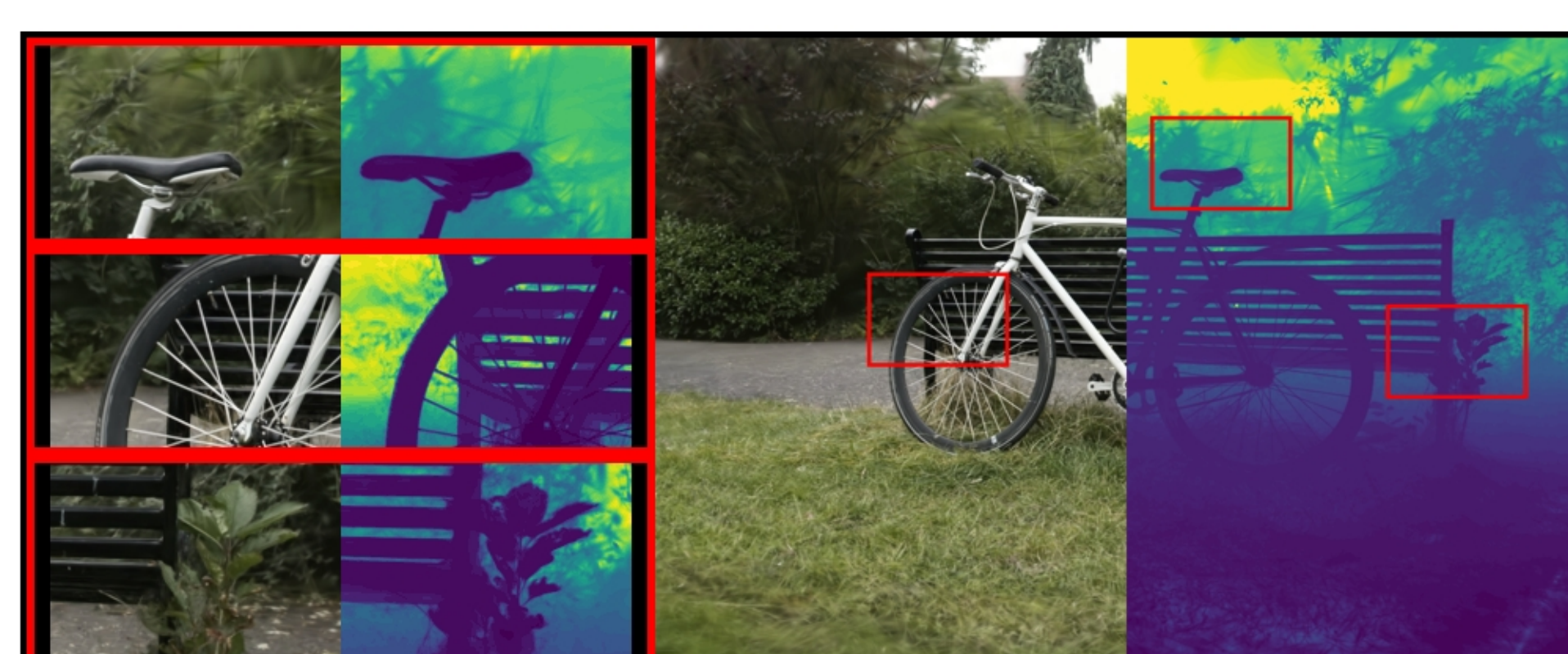
bicycle: Combined | | 0.0 | PSNR: 22.23 | LPIPS: 0.2571 | SSIM: 0.5663
