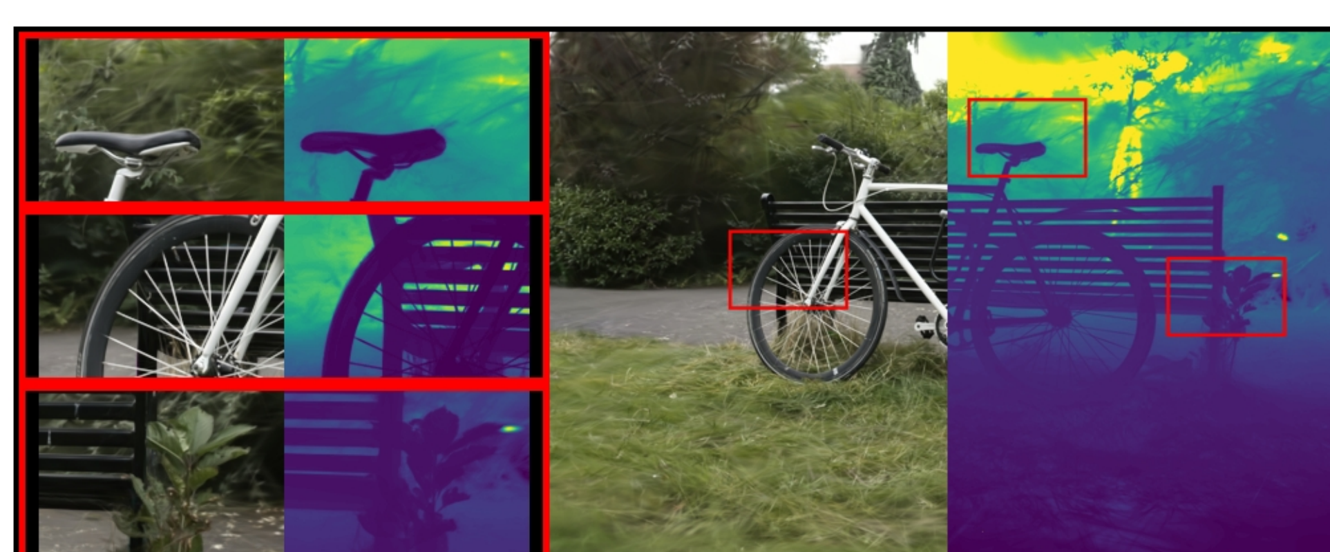
bicycle: COLMAP | | 0.0 | PSNR: 22.16 | LPIPS: 0.3495 | SSIM: 0.5587
