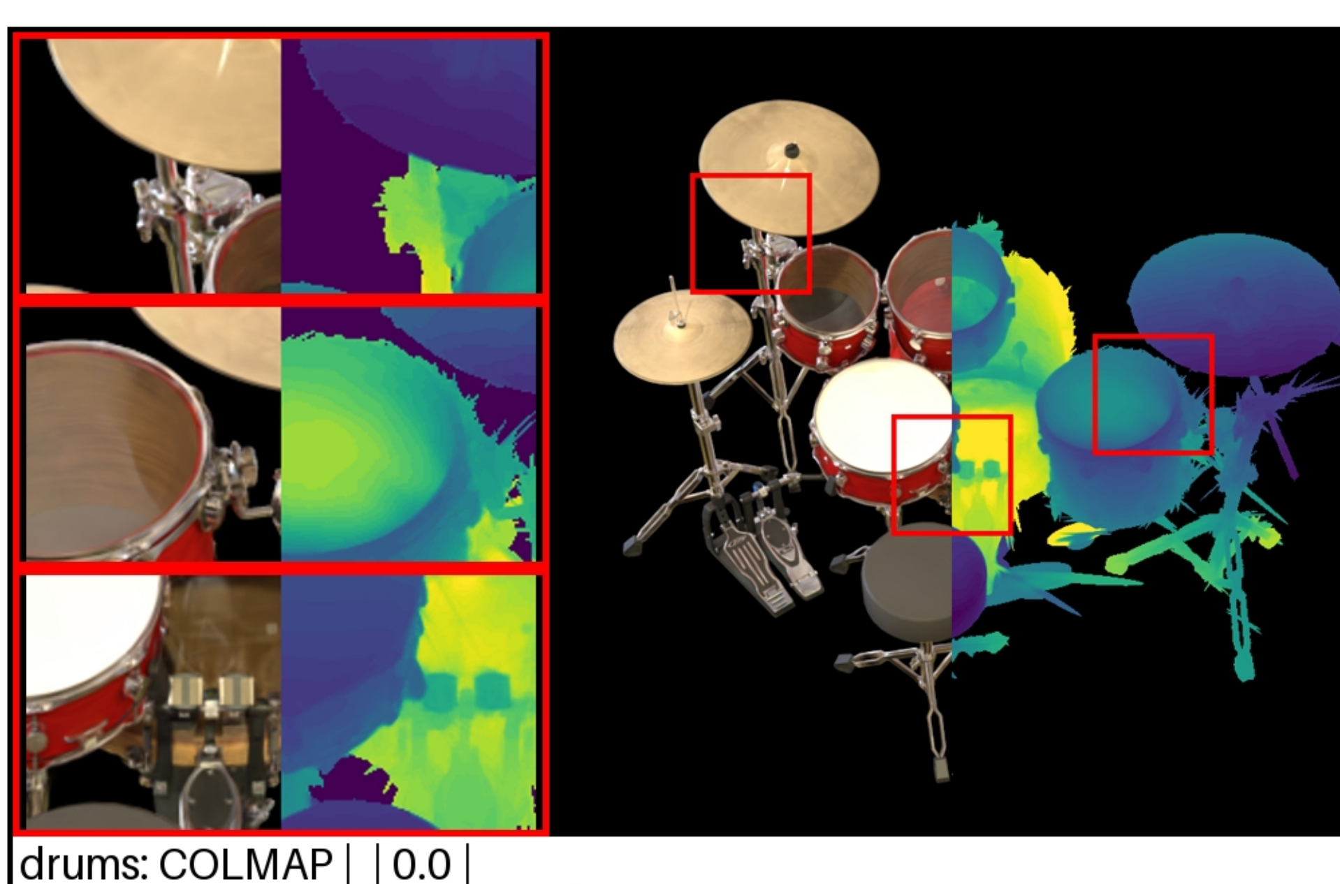
drums: COLMAP | | 0.0 | PSNR: 22.80 | LPIPS: 0.0892 | SSIM: 0.9061
