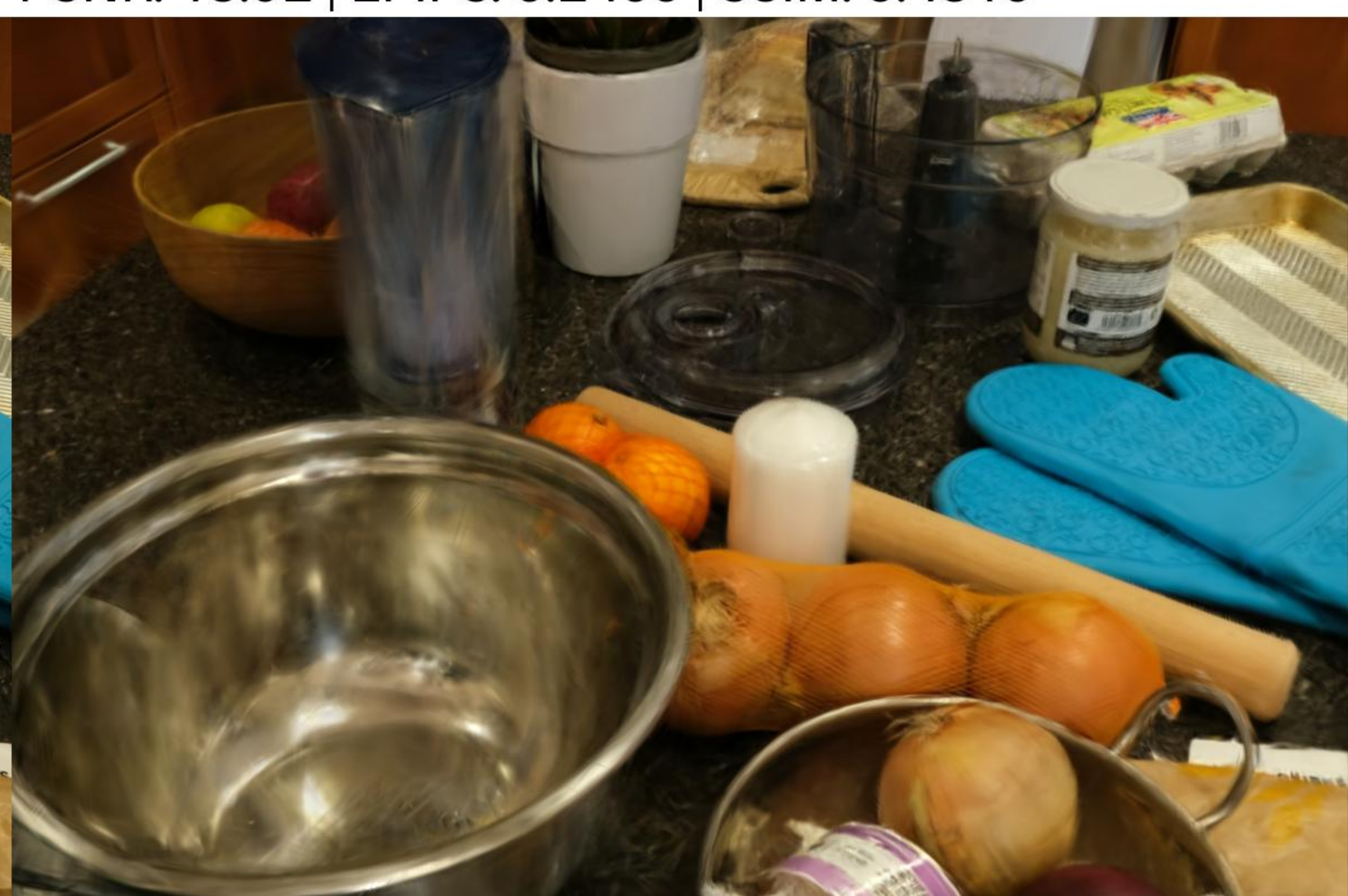
Config: VGGT | random | num_points=100000 PSNR: 18.41 | LPIPS: 0.3619 | SSIM: 0.5902
