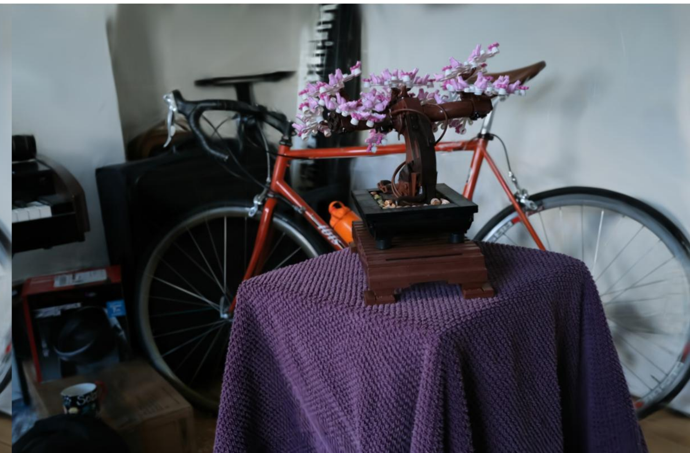
Config: VGGT | imagefps | num_points=100000 PSNR: 27.71 | LPIPS: 0.1387 | SSIM: 0.9172
