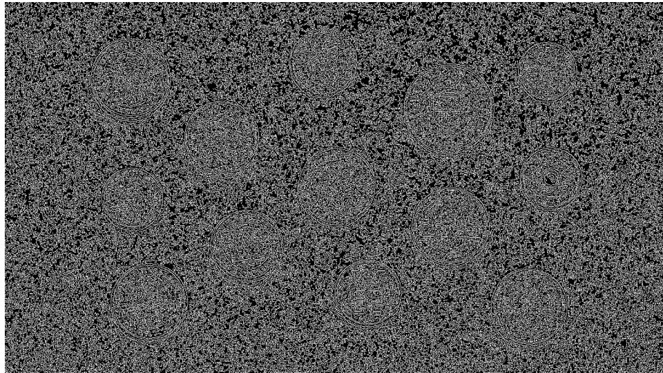
Without Gaussian
