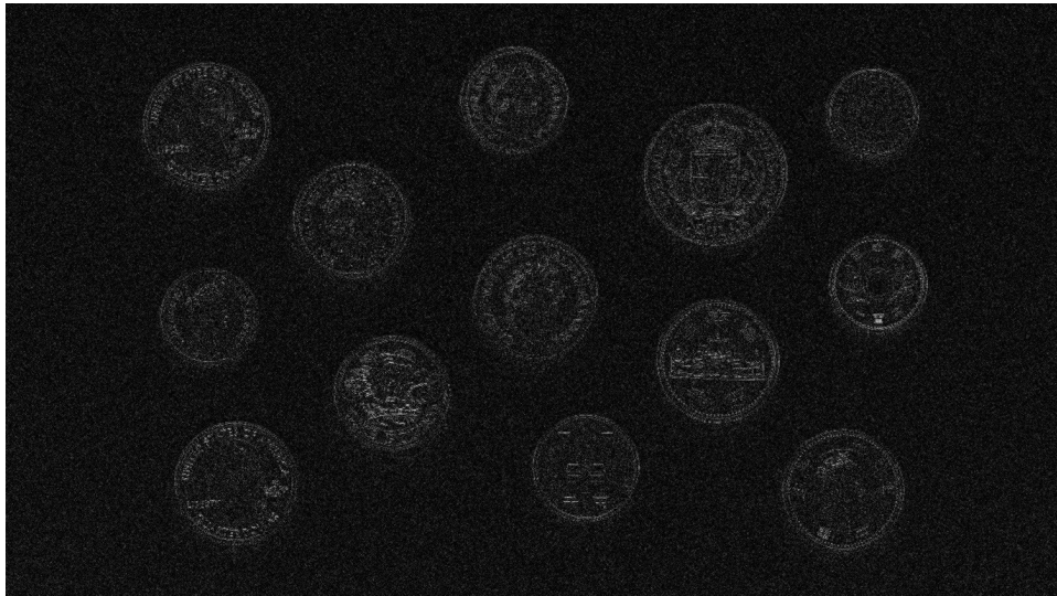
Direct Laplacian
