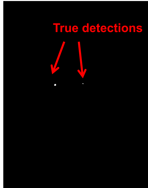
Thresholded Image
