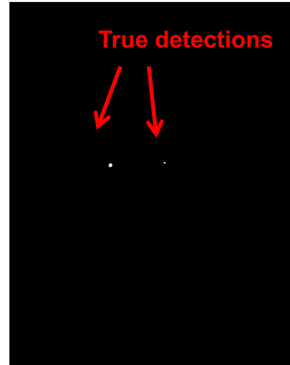
Thresholded image
