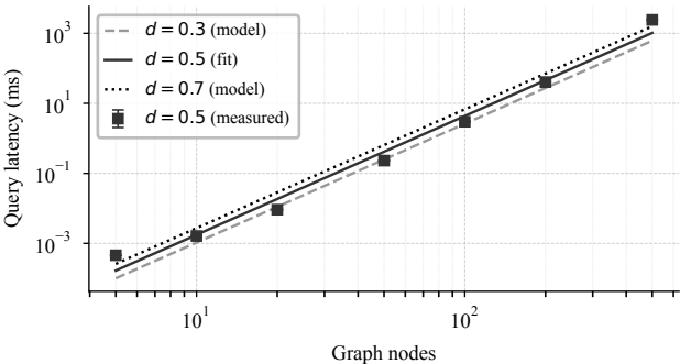
B6: Trust Graph Query Scaling (noisy-OR, depth \leq 4 )
