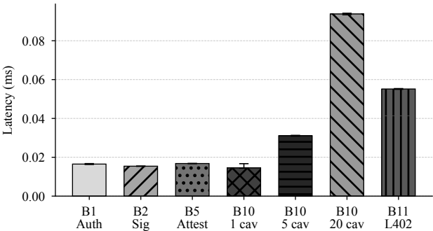
Crypto/Attestation/L402 Benchmarks (B1, B2, B5, B10, B11)
